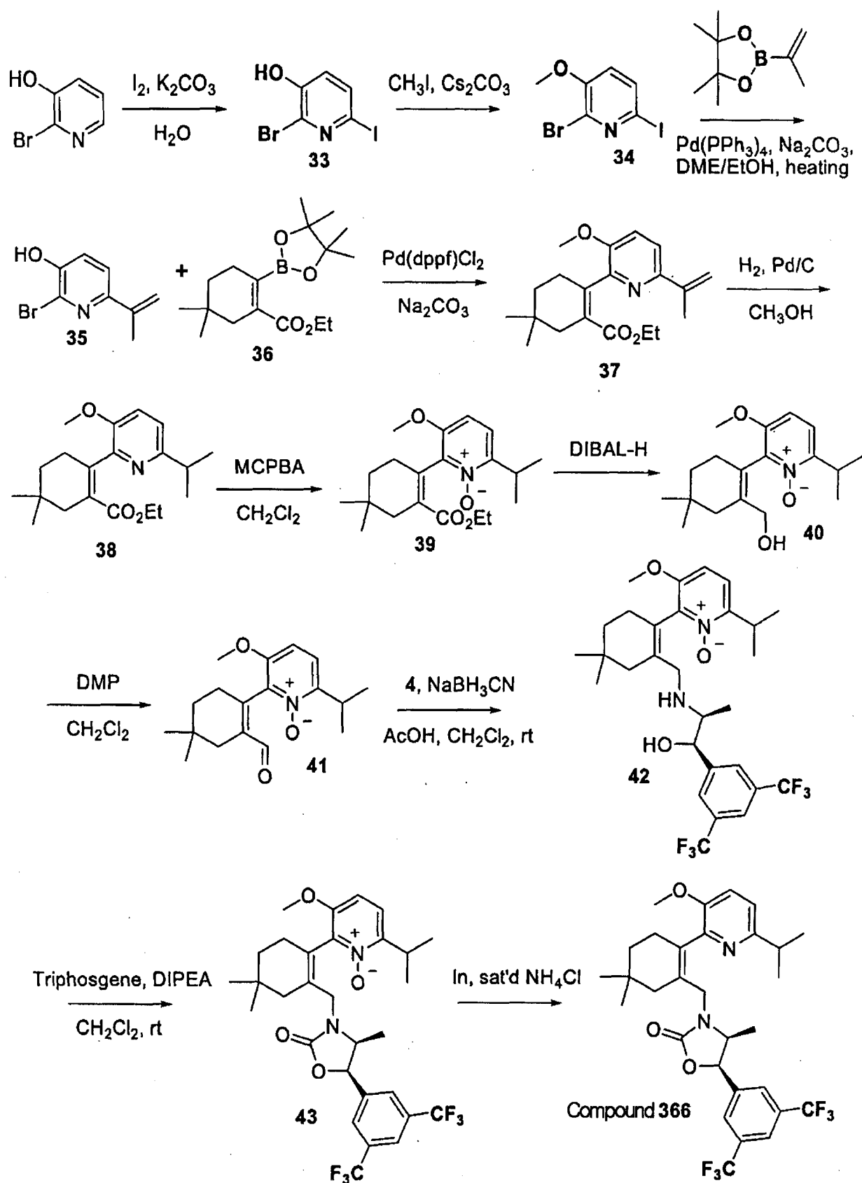
[Reaction Scheme 8]
