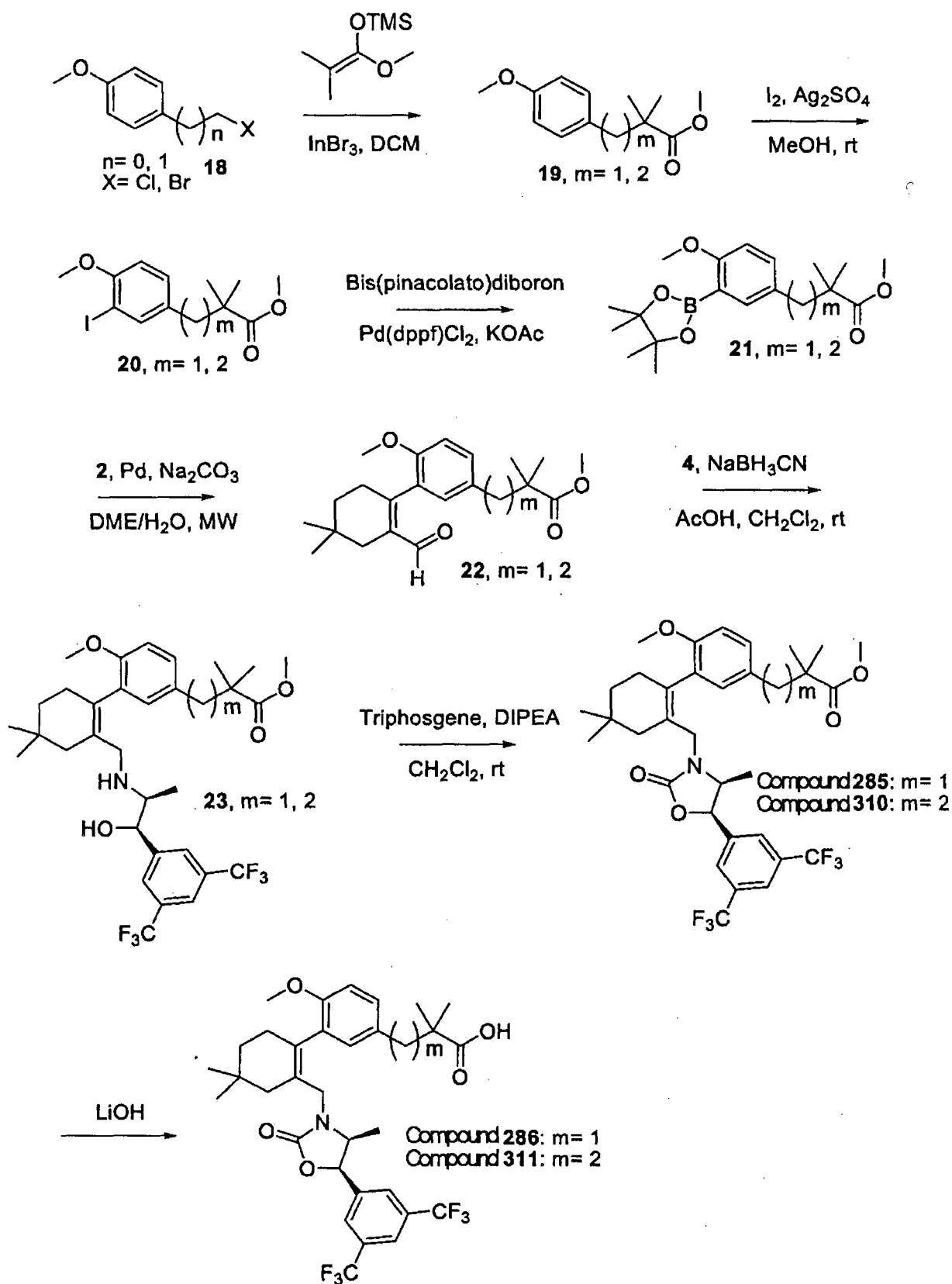
[Reaction Scheme 6]
