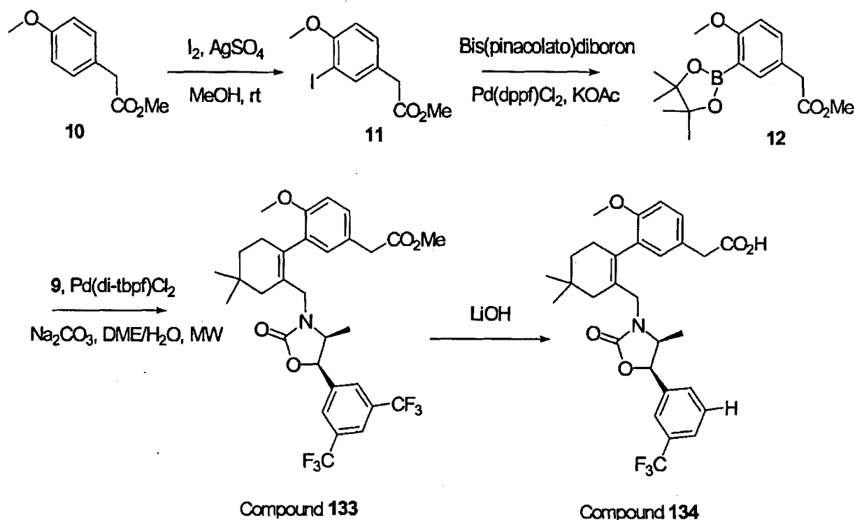
[Reaction Scheme 4]
