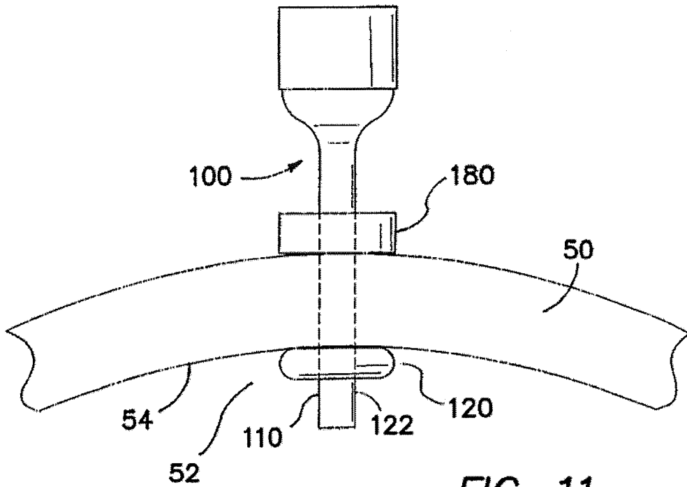
FIG. 11 PRIOR ART
