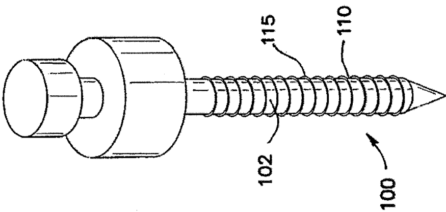
FIG. 6 PRIOR ART
