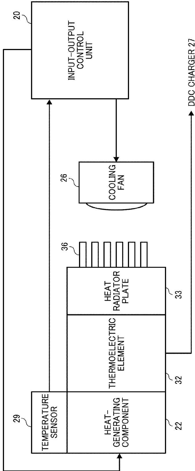
FIG. 3 RELATED ART
