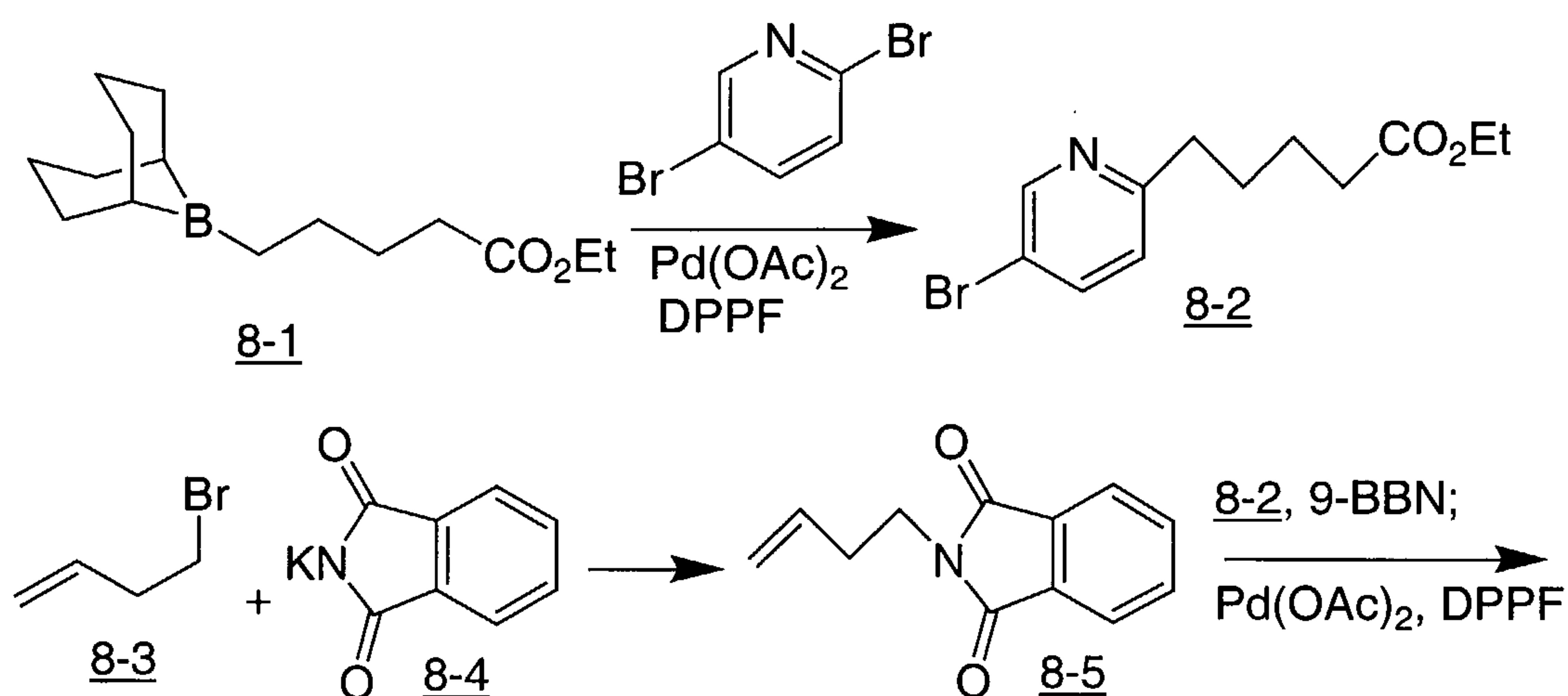
Scheme 8
