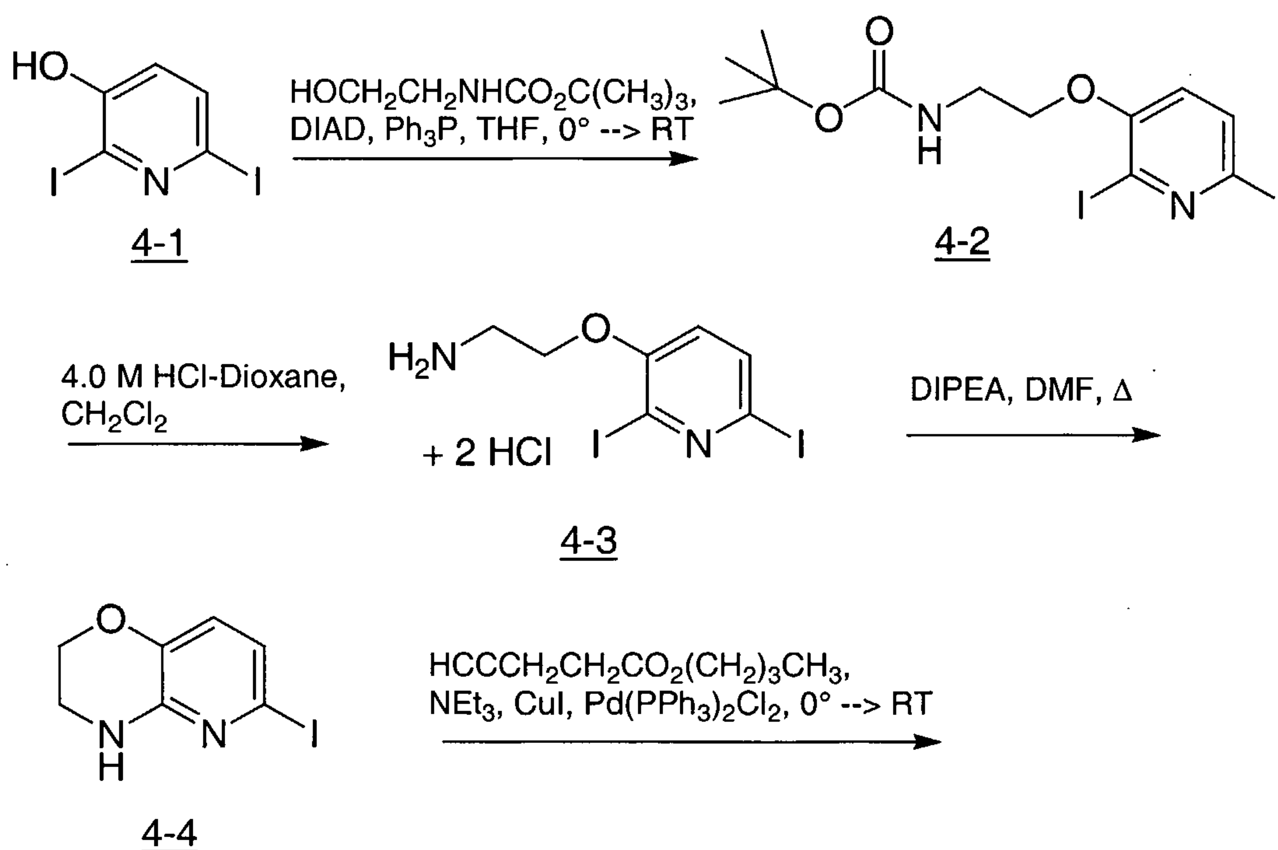
Scheme 4
