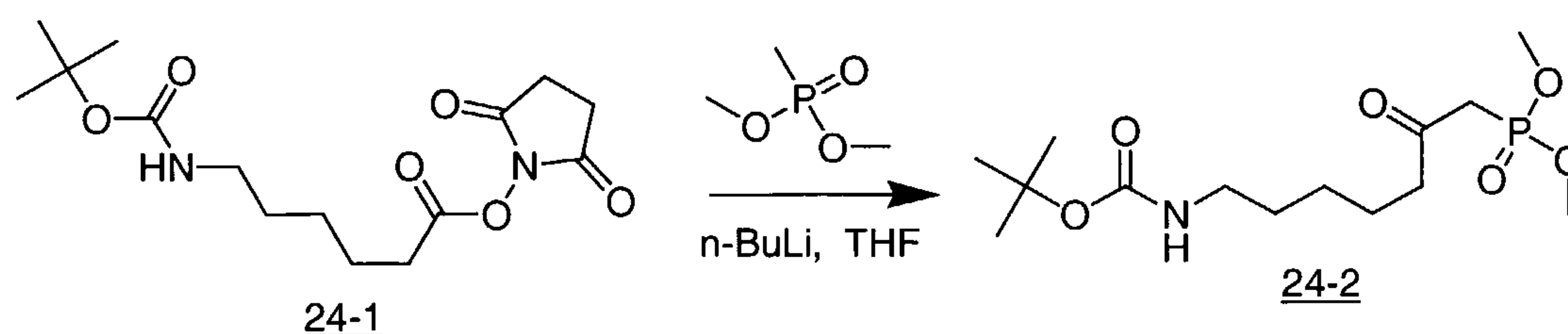
Scheme 24
