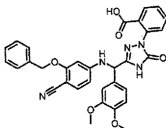
[Chemical Formula 474]
