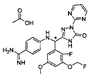
[Chemical Formula 292]
