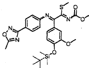
[Chemical Formula 104]
