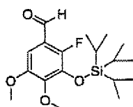
[Chemical Formula 227]
