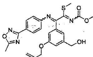
[Chemical Formula 262]
