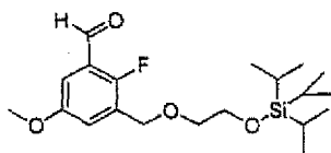
[Chemical Formula 550]
