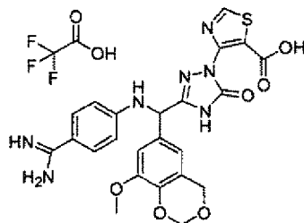
[Chemical Formula 425]
