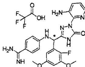
[Chemical Formula 362]
