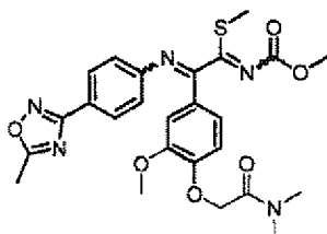
[Chemical Formula 294]
