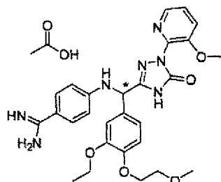
[Chemical Formula 661]
