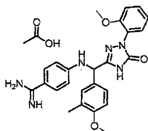
[Chemical Formula 651]
