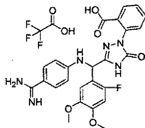
[Chemical Formula 38]
