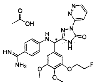
[Chemical Formula 271]
