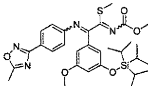
[Chemical Formula 59]
