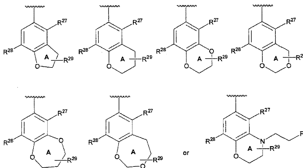
[Chemical Formula 20]
