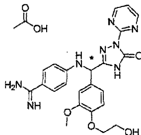
[Chemical Formula 824]
