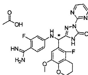
[Chemical Formula 803]
