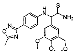
[Chemical Formula 120]
