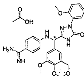
[Chemical Formula 278]
