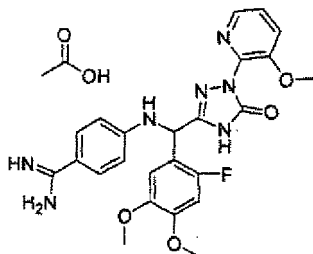
[Chemical Formula 326]
