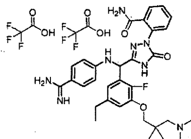
[Chemical Formula 633]
