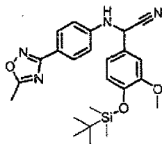
[Chemical Formula 102]
