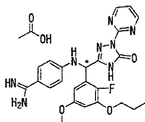
[Chemical Formula 765]
