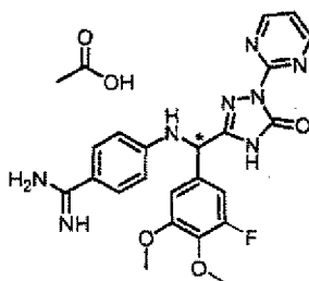
[Chemical Formula 313]
