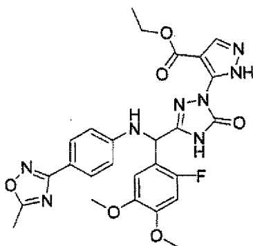
[Chemical Formula 399]
