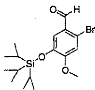
[Chemical Formula 319]
