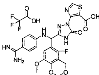
[Chemical Formula 422]
