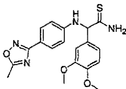
[Chemical Formula 168]
