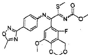
[Chemical Formula 155]
