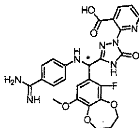
[Chemical Formula 452]
