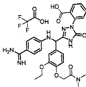
[Chemical Formula 743]
