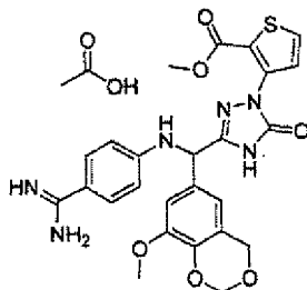
[Chemical Formula 388]
