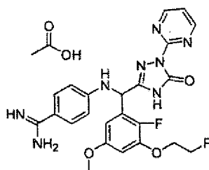
[Chemical Formula 56]
