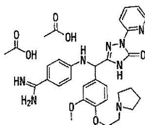
[Chemical Formula 763]
