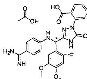
[Chemical Formula 39]
