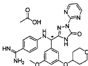
[Chemical Formula 223]
