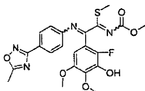
[Chemical Formula 228]
