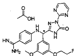
[Chemical Formula 221]
