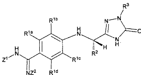
[Chemical Formula 3]
