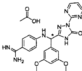
[Chemical Formula 70]
