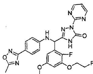
[Chemical Formula 55]
