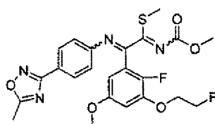
[Chemical Formula 54]
