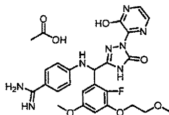
[Chemical Formula 804]
