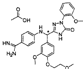
[Chemical Formula 662]
