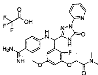
[Chemical Formula 618]
