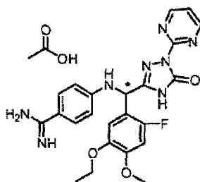
[Chemical Formula 311]
