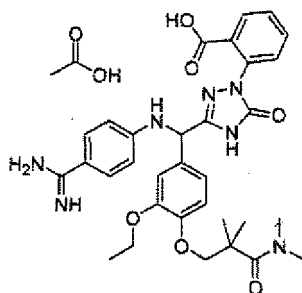
[Chemical Formula 764]
