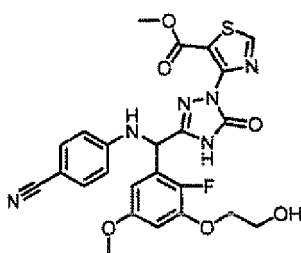
[Chemical Formula 472]
