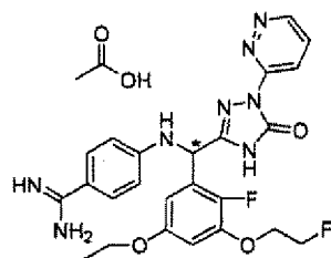
[Chemical Formula 234]
