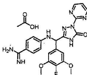
[Chemical Formula 654]
