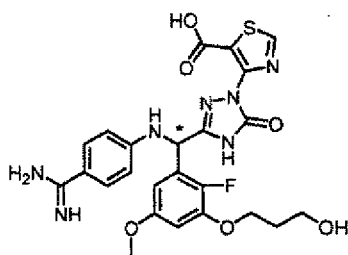
[Chemical Formula 417]
