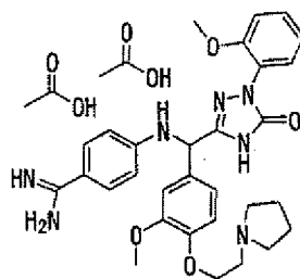
[Chemical Formula 762]
