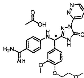
[Chemical Formula 757]
