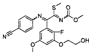
[Chemical Formula 471]
