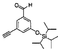
[Chemical Formula 195]
