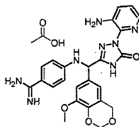
[Chemical Formula 217]
