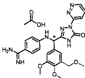
[Chemical Formula 656]
