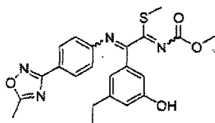
[Chemical Formula 241]
