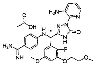
[Chemical Formula 532]
