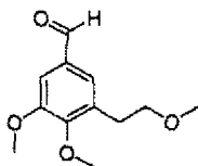
[Chemical Formula 335]
