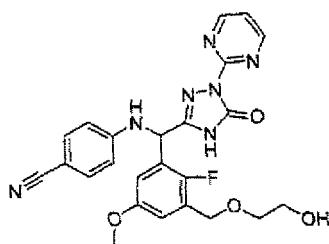
[Chemical Formula 552]
