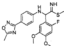
[Chemical Formula 34]
