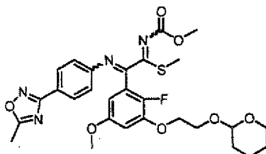
[Chemical Formula 437]
