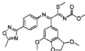
[Chemical Formula 256]
