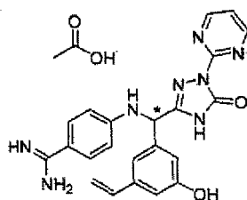
[Chemical Formula 200]
