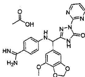
[Chemical Formula 682]
