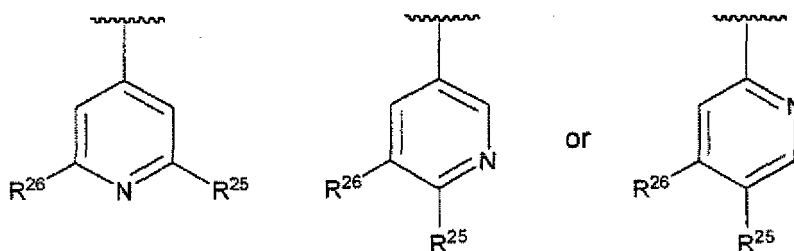
[Chemical Formula 17]
