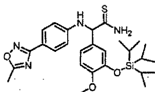
[Chemical Formula 95]
