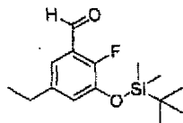
[Chemical Formula 350]
