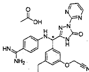
[Chemical Formula 587]
