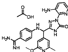
[Chemical Formula 112]
