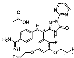
[Chemical Formula 287]
