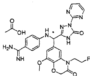
[Chemical Formula 565]
