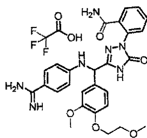
[Chemical Formula 741]
