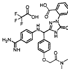
, [Chemical Formula 745]
