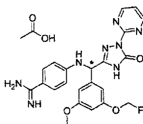
[Chemical Formula 293]
