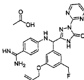
[Chemical Formula 705]
