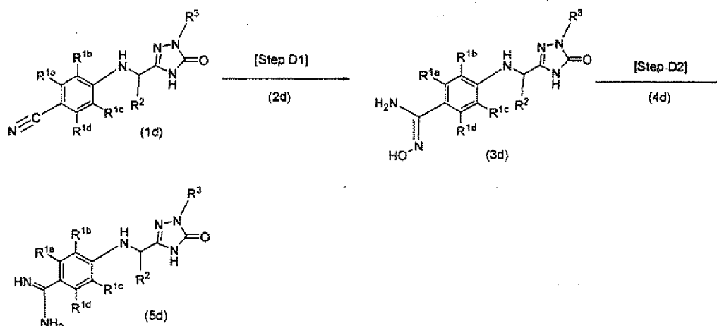
[Chemical Formula 29]
