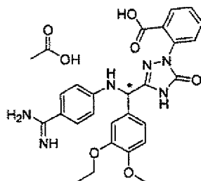
[Chemical Formula 634]
