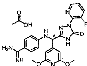
[Chemical Formula 216]
