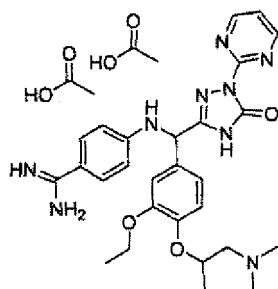
[Chemical Formula 723]
