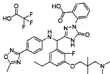
[Chemical Formula 375]
