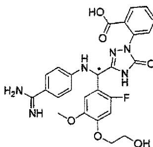
[Chemical Formula 460]
