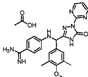
[Chemical Formula 650]
