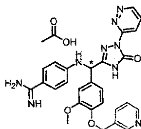
[Chemical Formula 760]
