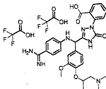
[Chemical Formula 742]
