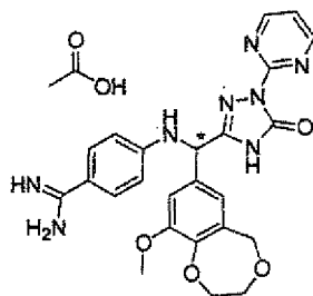
[Chemical Formula 666]
