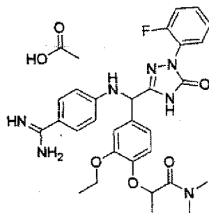
[Chemical Formula 719]
