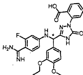
[Chemical Formula 792]
