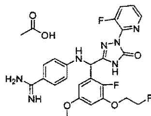
[Chemical Formula 628]
