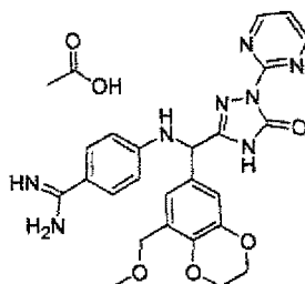
[Chemical Formula 680]
