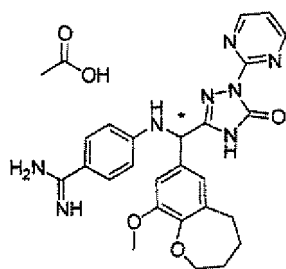
[Chemical Formula 811]
