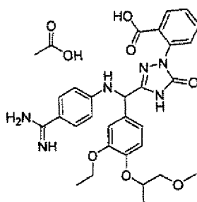
[Chemical Formula 722]
