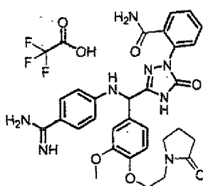
[Chemical Formula 758]
