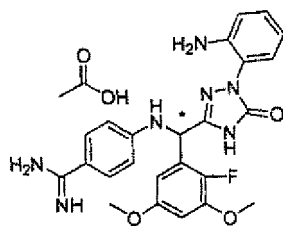
[Chemical Formula 787]
