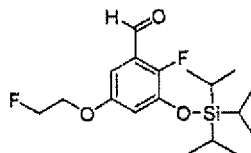
[Chemical Formula 285]
