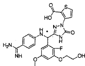
[Chemical Formula 572]
