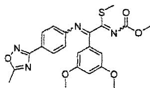
[Chemical Formula 567]
