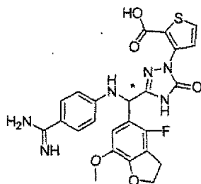
[Chemical Formula 546]
