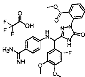
[Chemical Formula 299]
