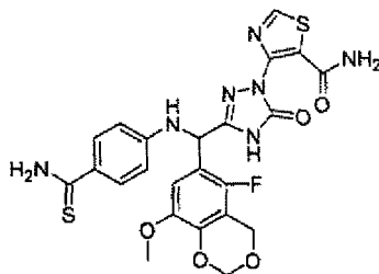
[Chemical Formula 418]
