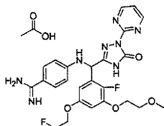
[Chemical Formula 623]
