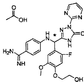
[Chemical Formula 584]
