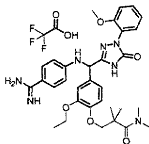
[Chemical Formula 753]
