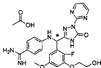
[Chemical Formula 439]
