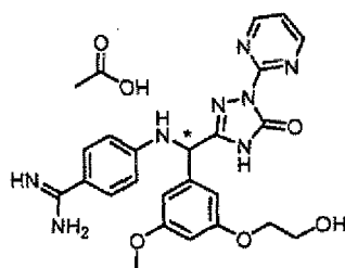
[Chemical Formula 797]
