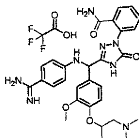
[Chemical Formula 751]
