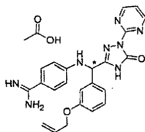
[Chemical Formula 588]
