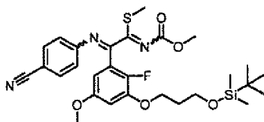
[Chemical Formula 416]
