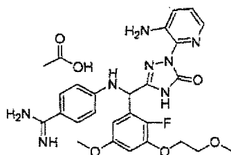
[Chemical Formula 531]
