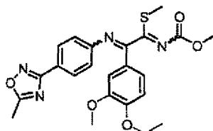
[Chemical Formula 106]
