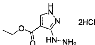
[Chemical Formula 398]
