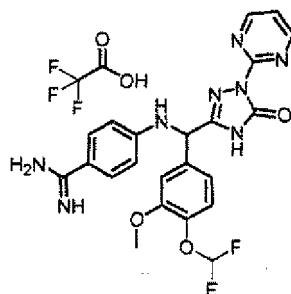
[Chemical Formula 652]
