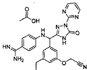
[Chemical Formula 246]
