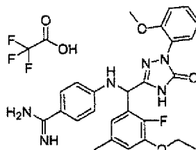
[Chemical Formula 620]
