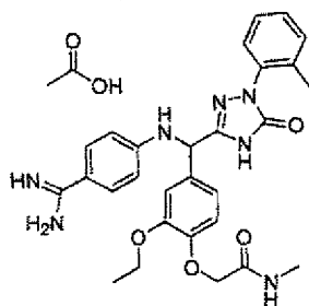
[Chemical Formula 668]
