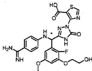
[Chemical Formula 427]
