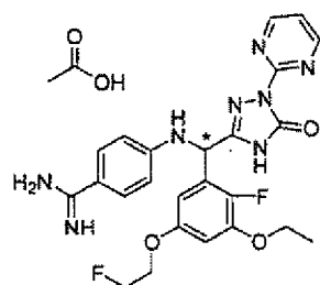
[Chemical Formula 627]
