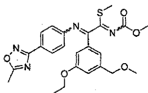
[Chemical Formula 259]
