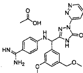
[Chemical Formula 239]
