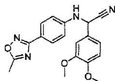
[Chemical Formula 167]
