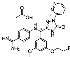
[Chemical Formula 224]
