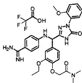
[Chemical Formula 746]
