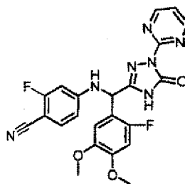
[Chemical Formula 378]
