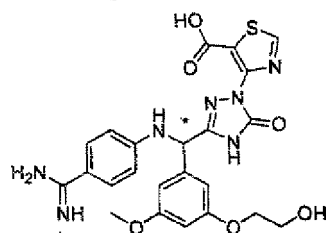
[Chemical Formula 776]
