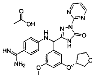
[Chemical Formula 63]
