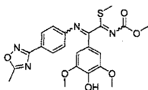
[Chemical Formula 265]
