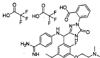
[Chemical Formula 773]
