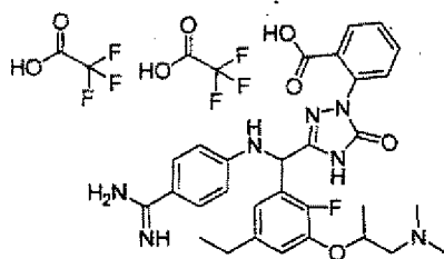
[Chemical Formula 771]
