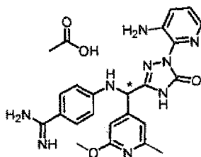
[Chemical Formula 113]
