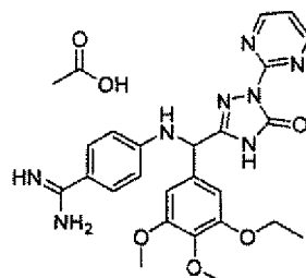
[Chemical Formula 614]
