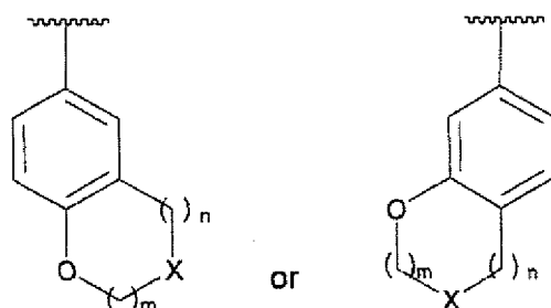
[Chemical Formula 11]
