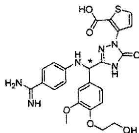
[Chemical Formula 823]
