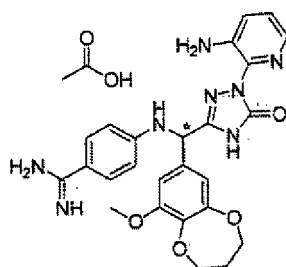
[Chemical Formula 164]
