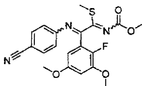
[Chemical Formula 44]
