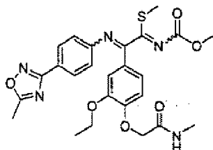
[Chemical Formula 329]
