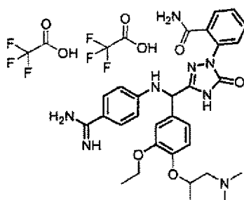
[Chemical Formula 636]
