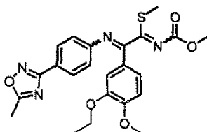
[Chemical Formula 98]
