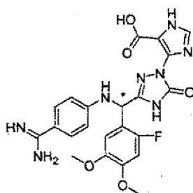
[Chemical Formula 488]
