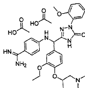
[Chemical Formula 713]
