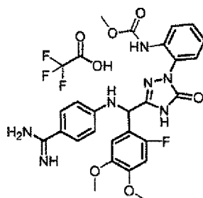
[Chemical Formula 641]
