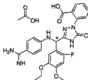
[Chemical Formula 324]
