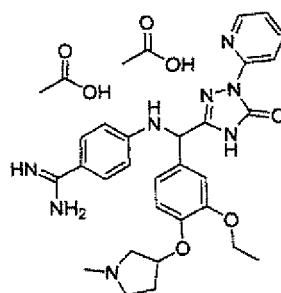
[Chemical Formula 717]
