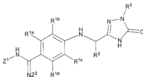
[Chemical Formula 1]
