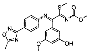
[Chemical Formula 69]
