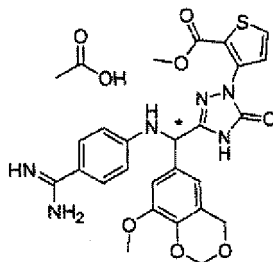
[Chemical Formula 389]
