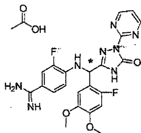
[Chemical Formula 582]
