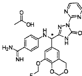
[Chemical Formula 631]
