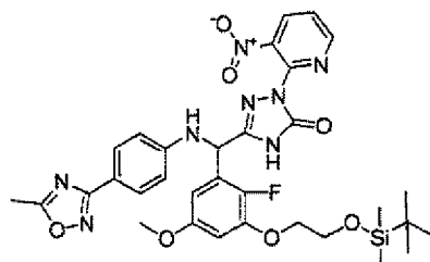
[Chemical Formula 525]
