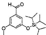
[Chemical Formula 58]
