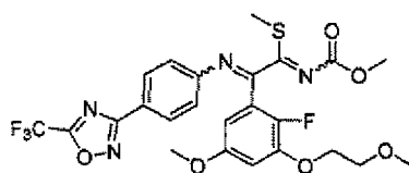
[Chemical Formula 529]
