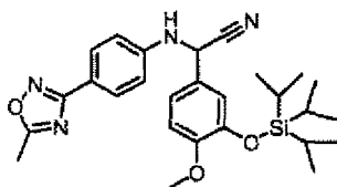
[Chemical Formula 94]
