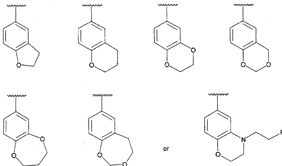
[Chemical Formula 12]
