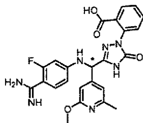
[Chemical Formula 440]
