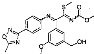
[Chemical Formula 80]
