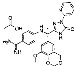
[Chemical Formula 544]
