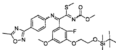
[Chemical Formula 524]
