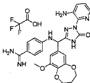
[Chemical Formula 163]
