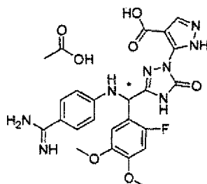
[Chemical Formula 509]
