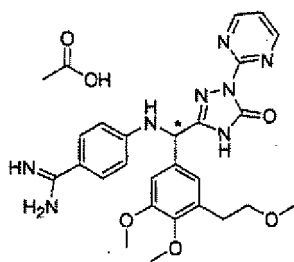
[Chemical Formula 337]
