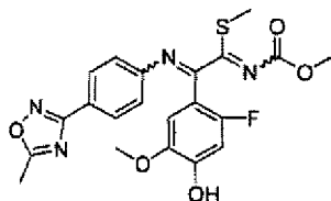
[Chemical Formula 458]
