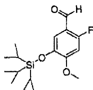
[Chemical Formula 320]
