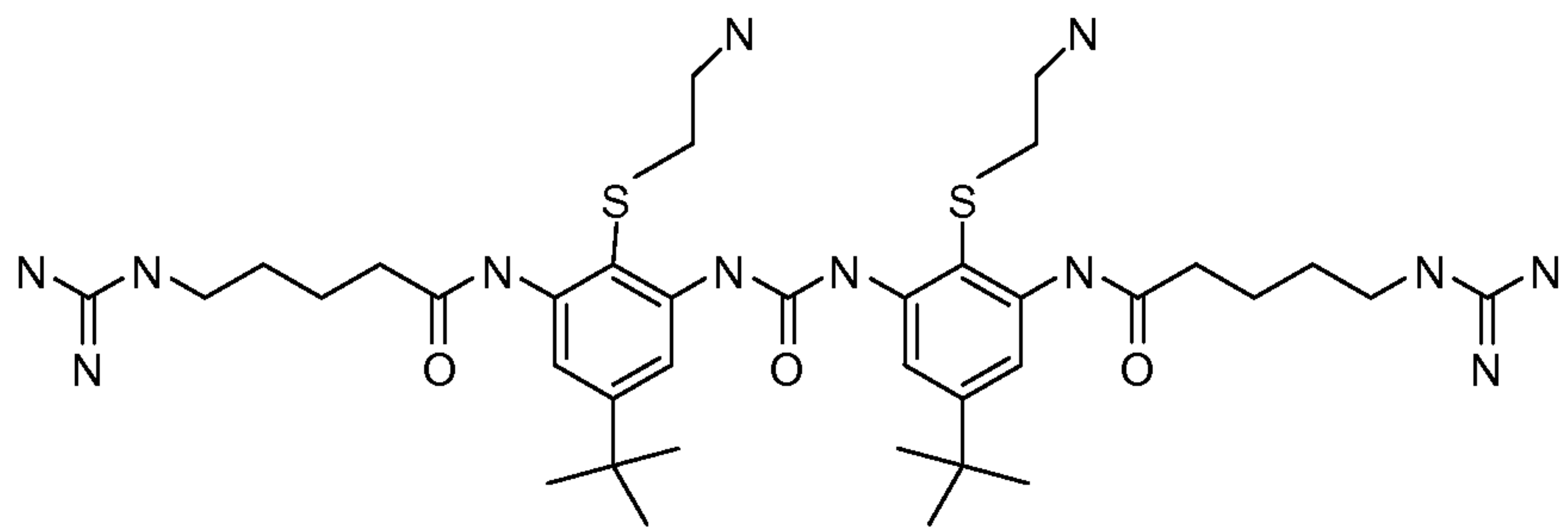
Compound 103
