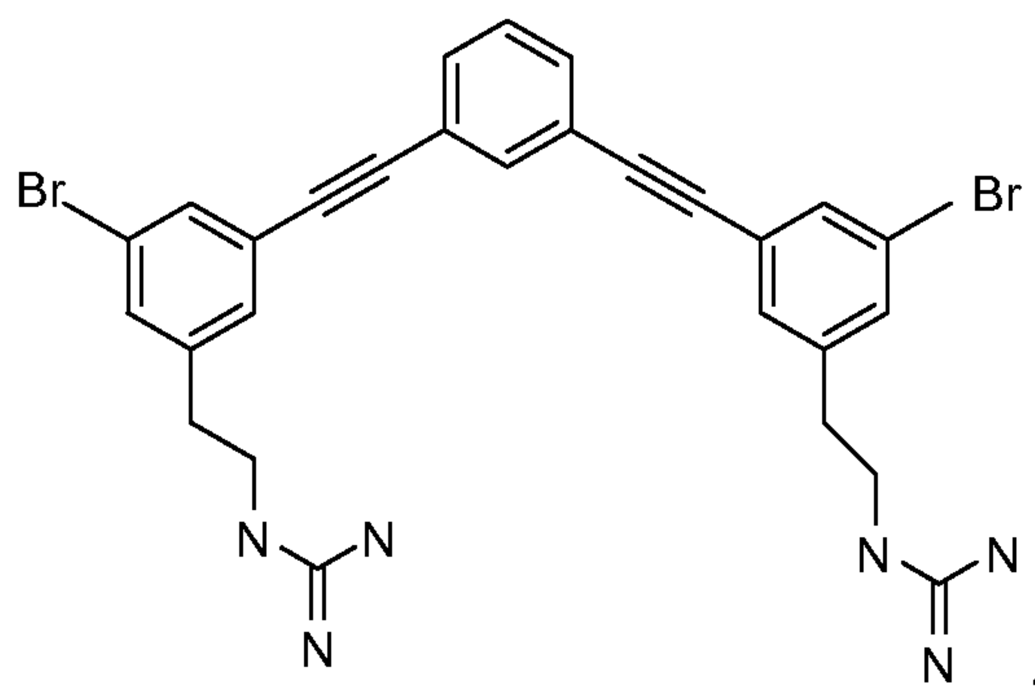
Compound 115
