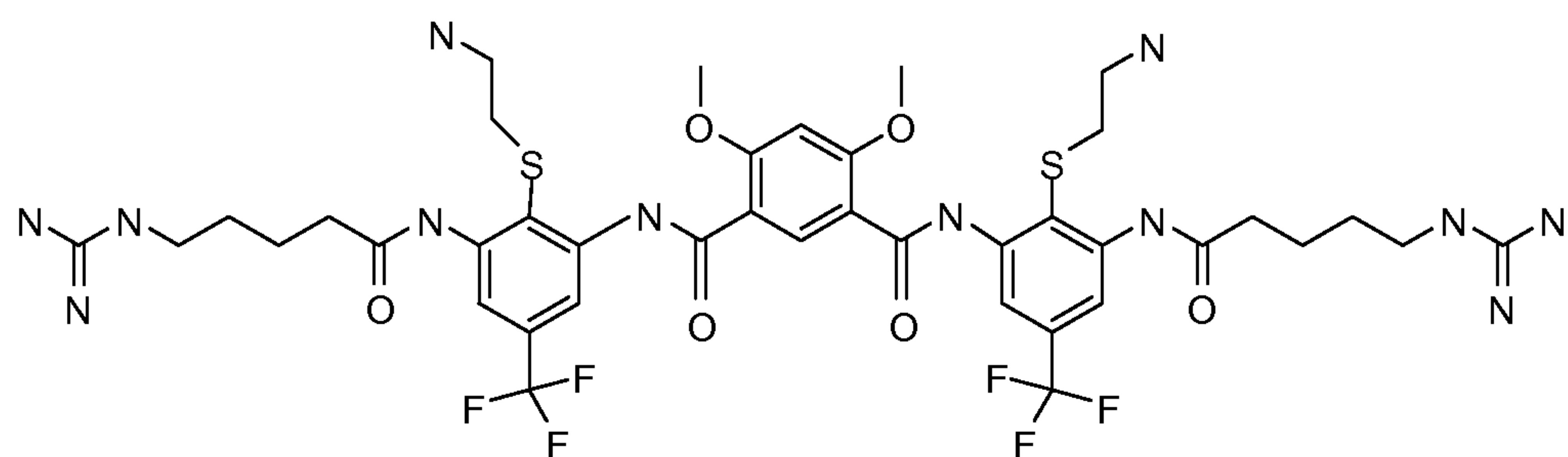
Compound 101
