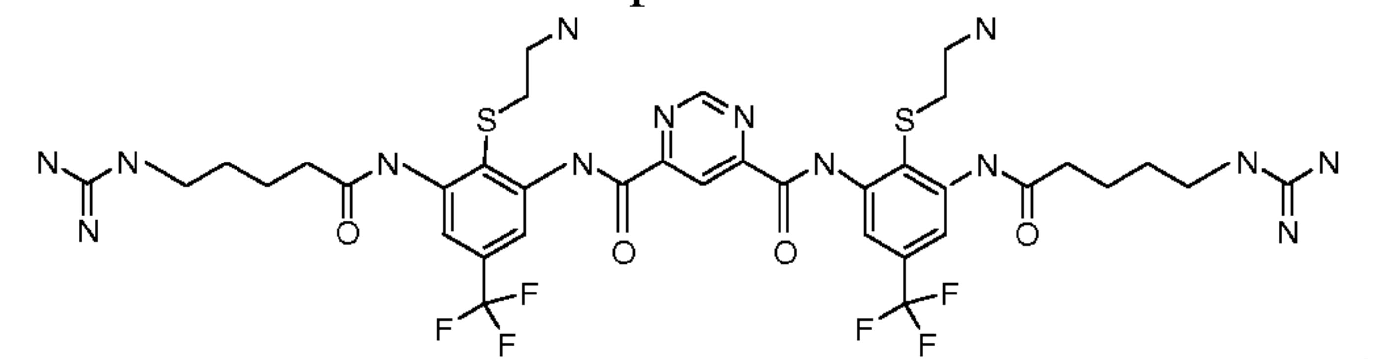
Compound 124
