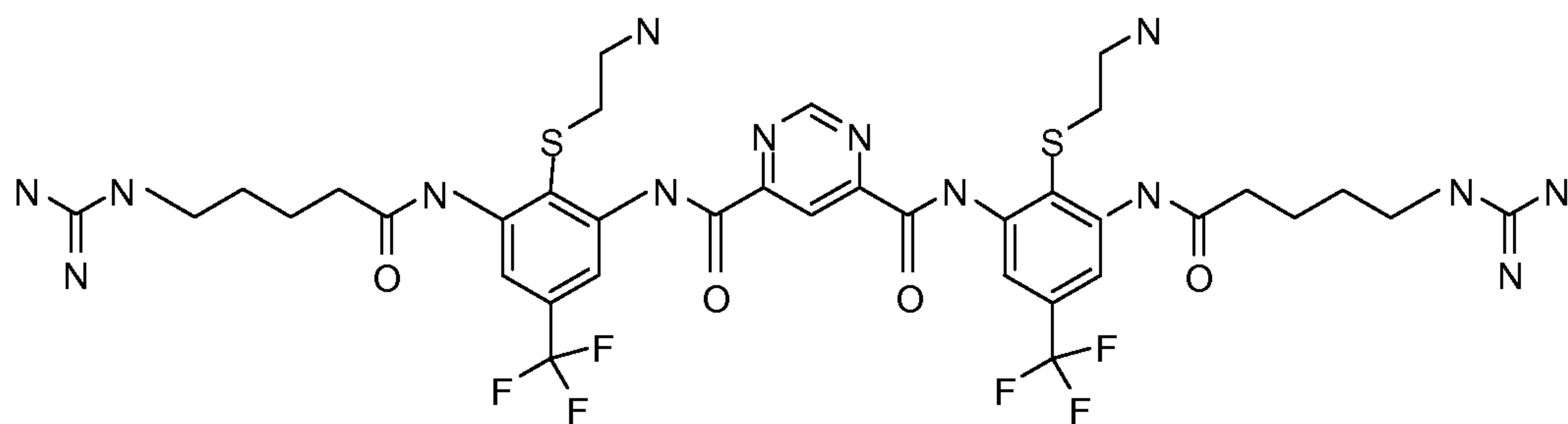
Compound 124
