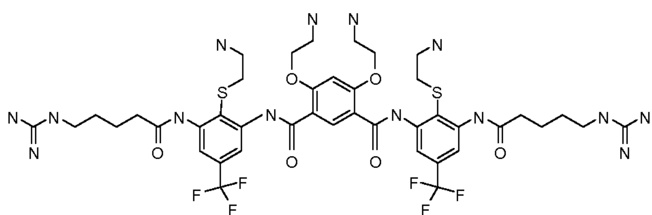
Compound 102
