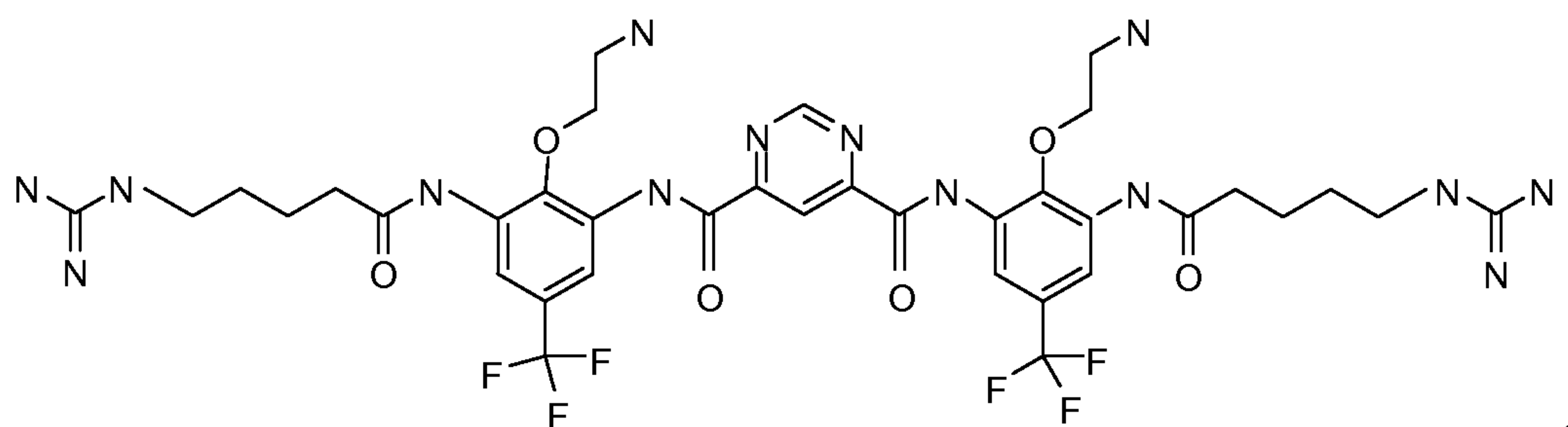
Compound 114
