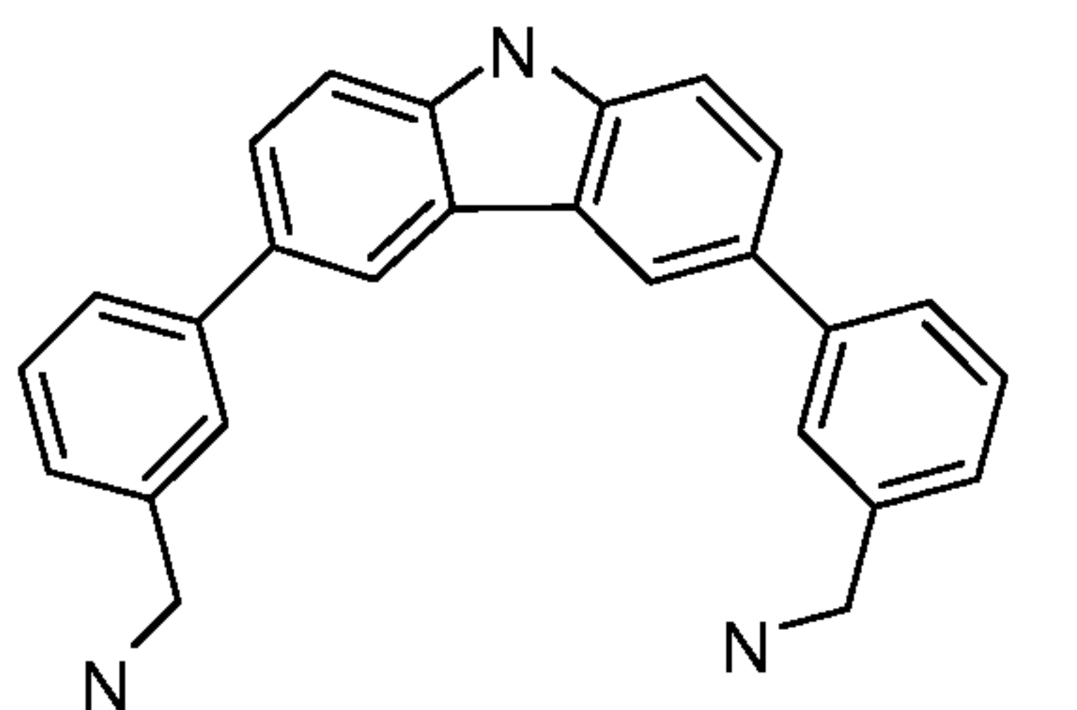
Compound 118
