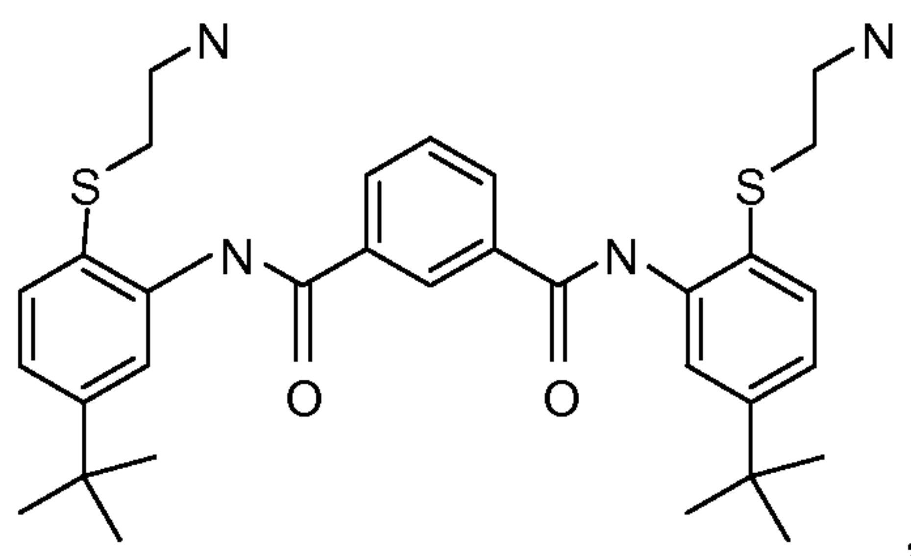
Compound 100
