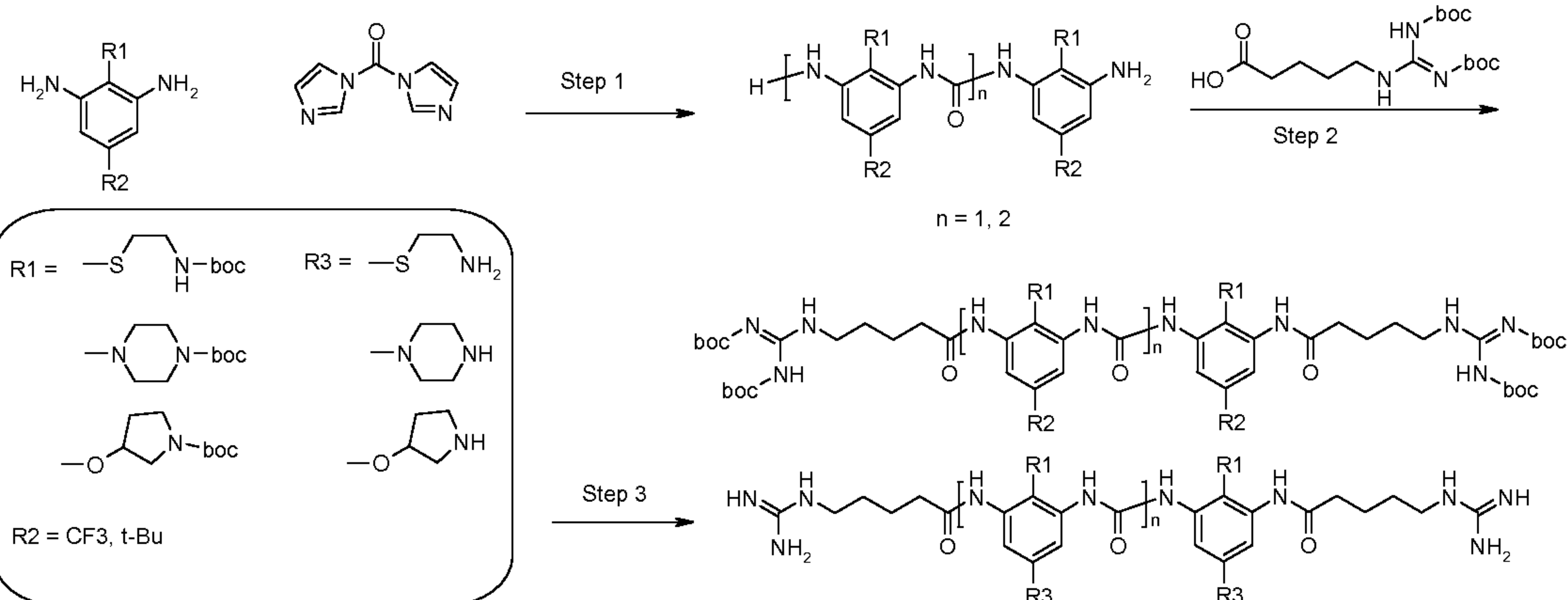
Compound 150
