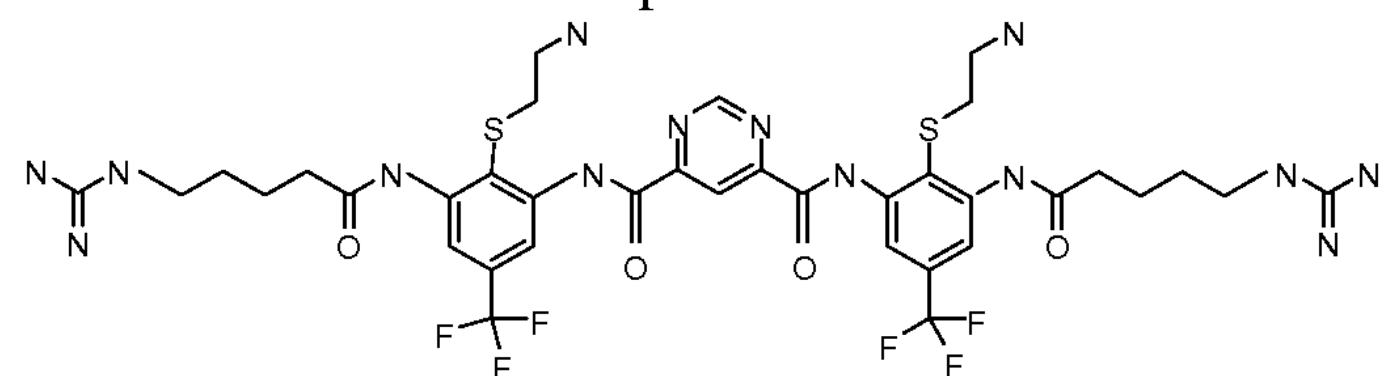
Compound 121
