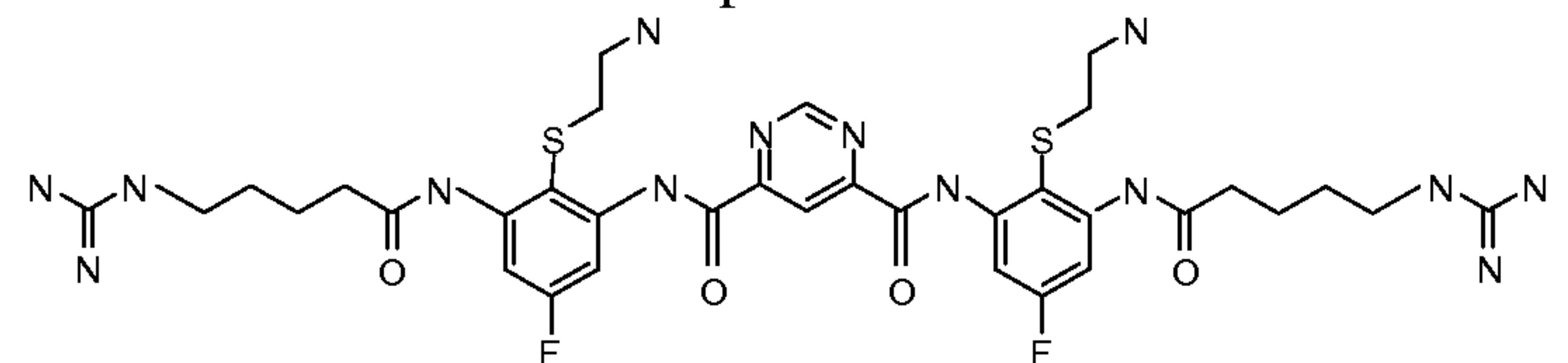
Compound 107
