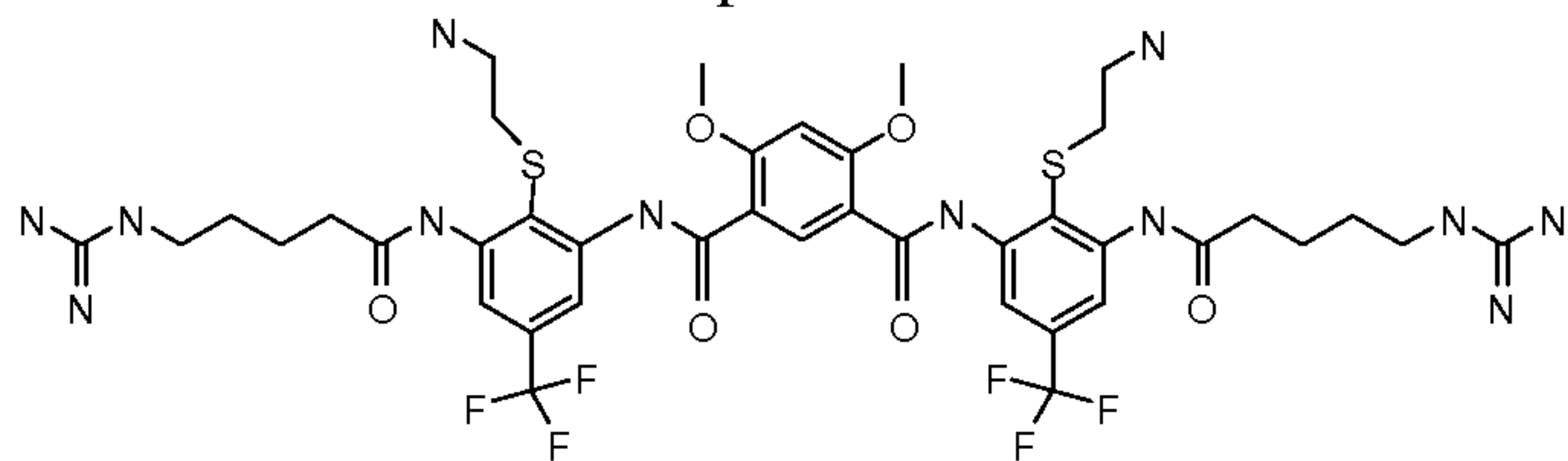
Compound 101
