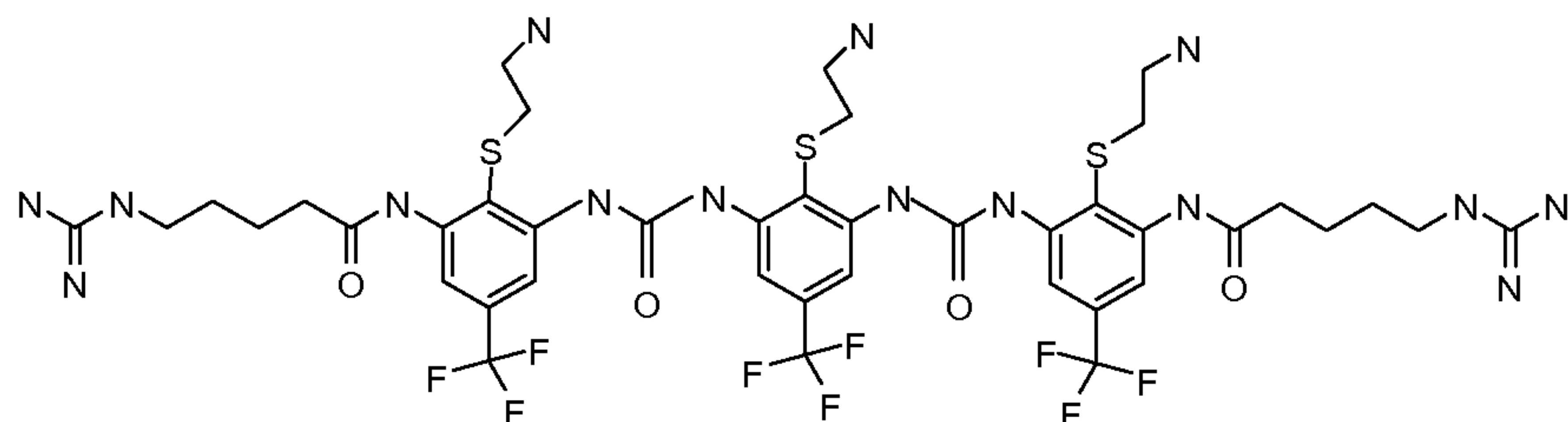
Compound 150
