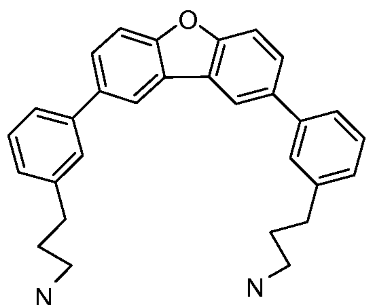
Compound 120
