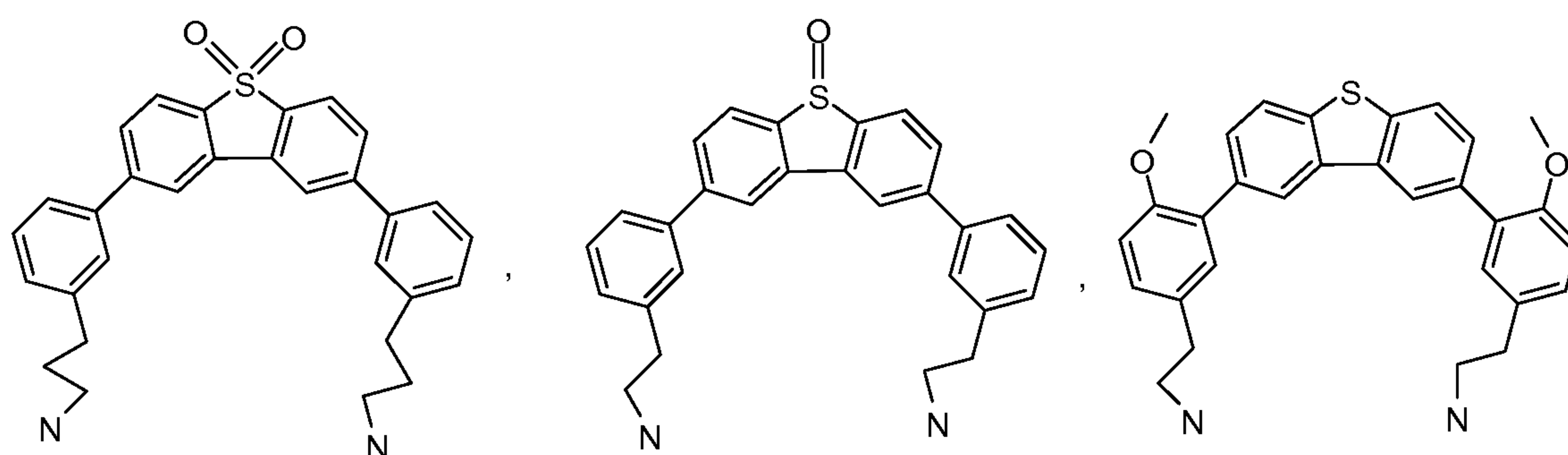
Compound 133
