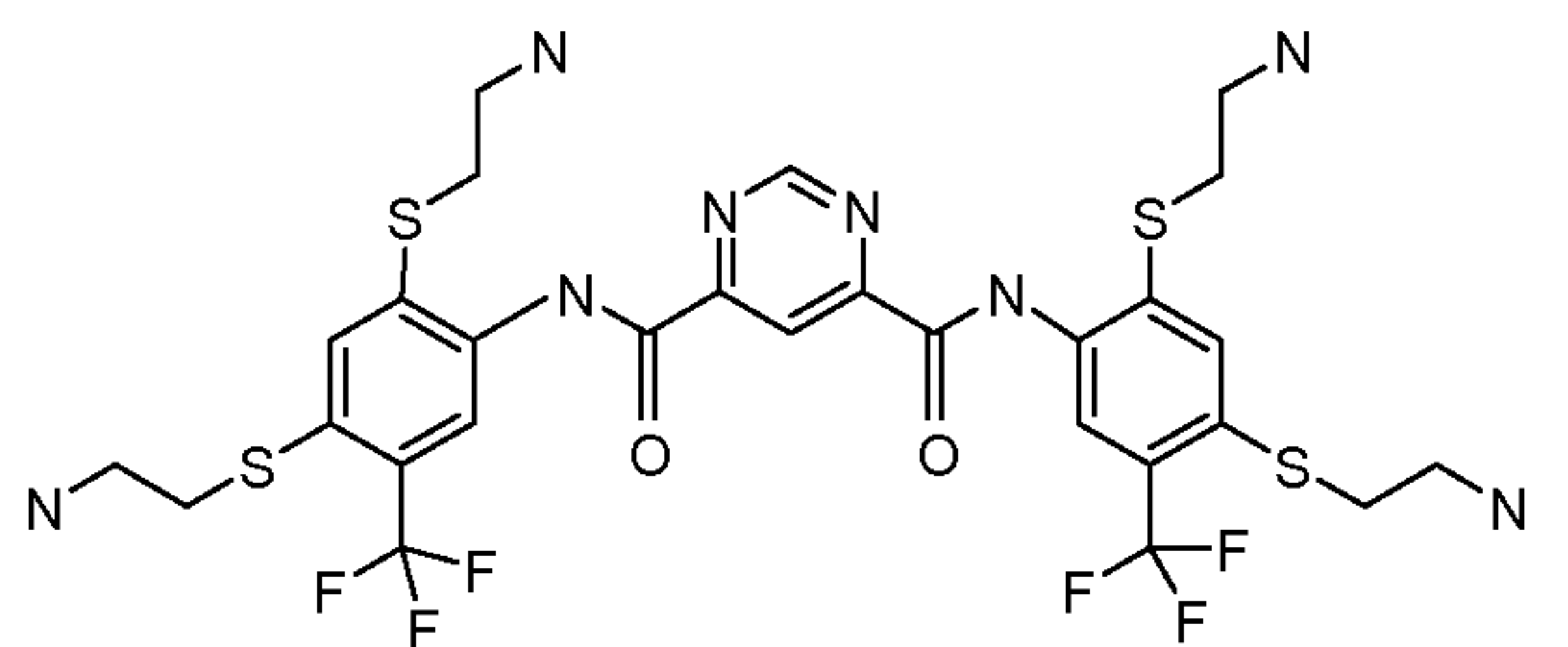
Compound 112
