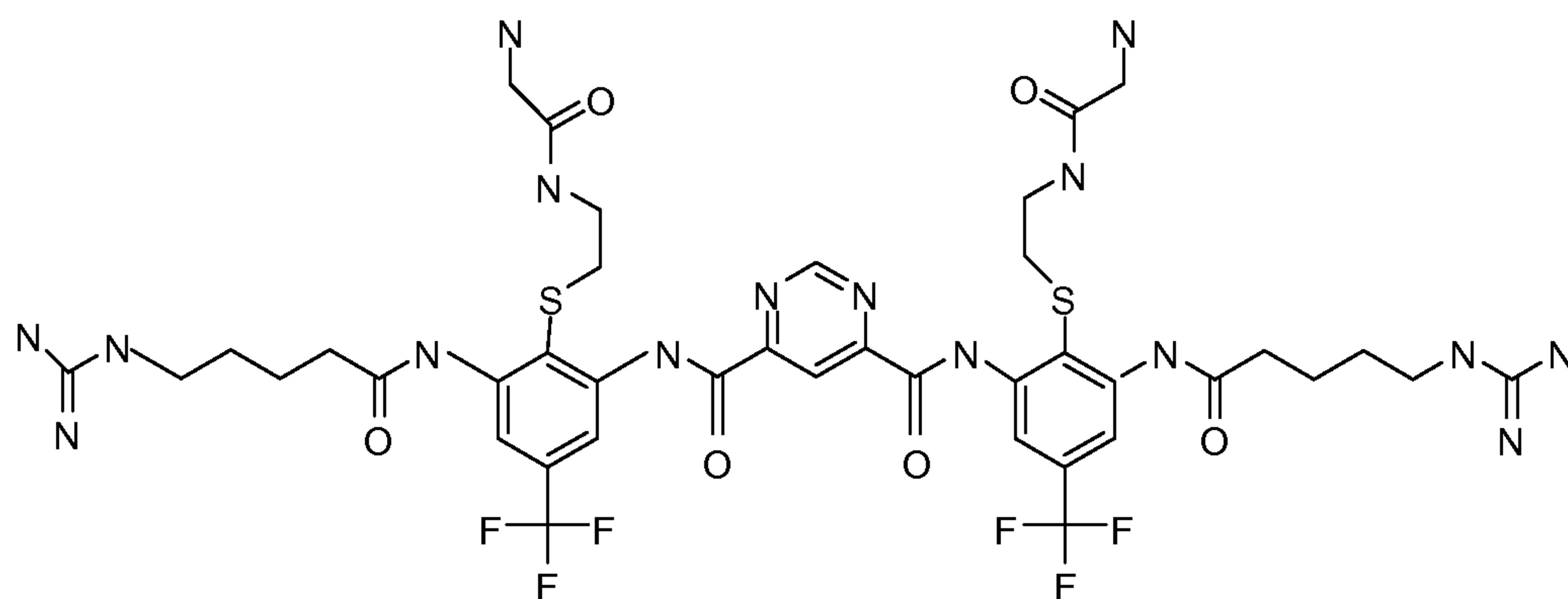
Compound 153
