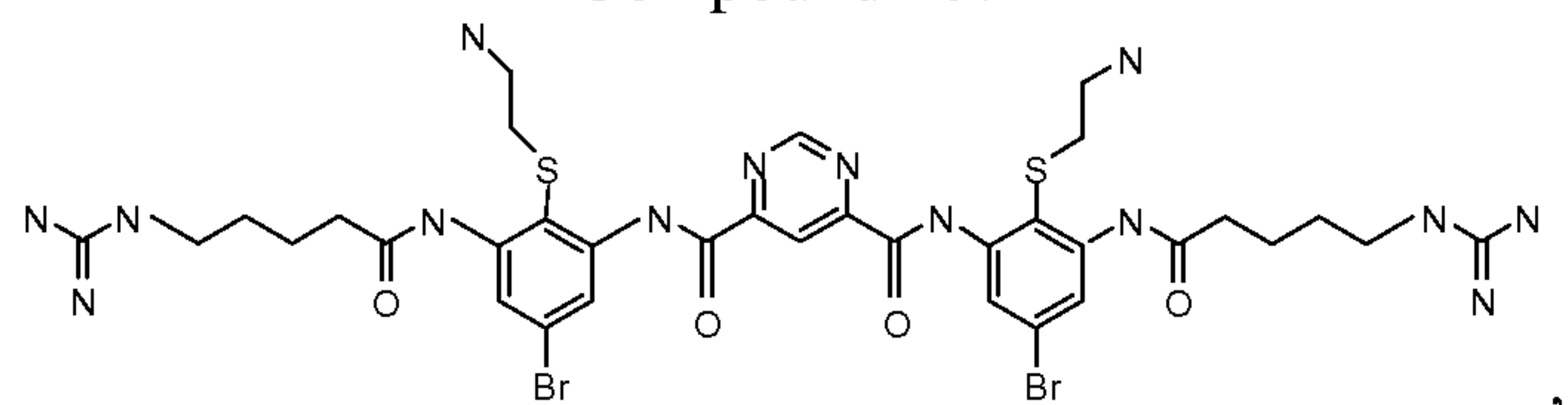
Compound 123
