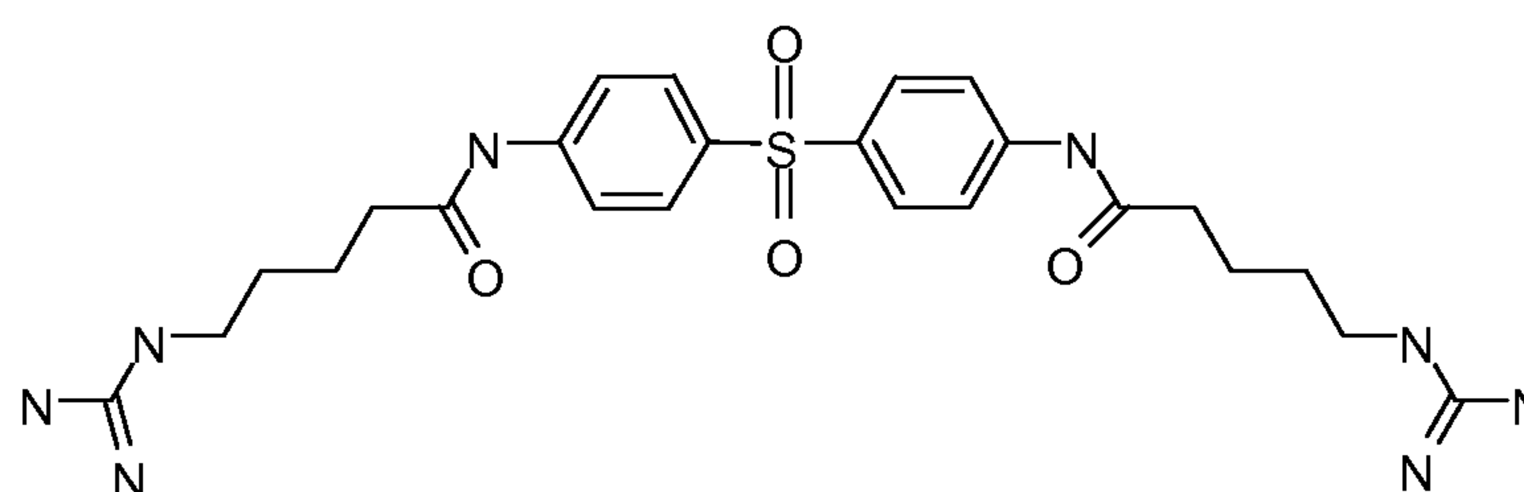
Compound 149
