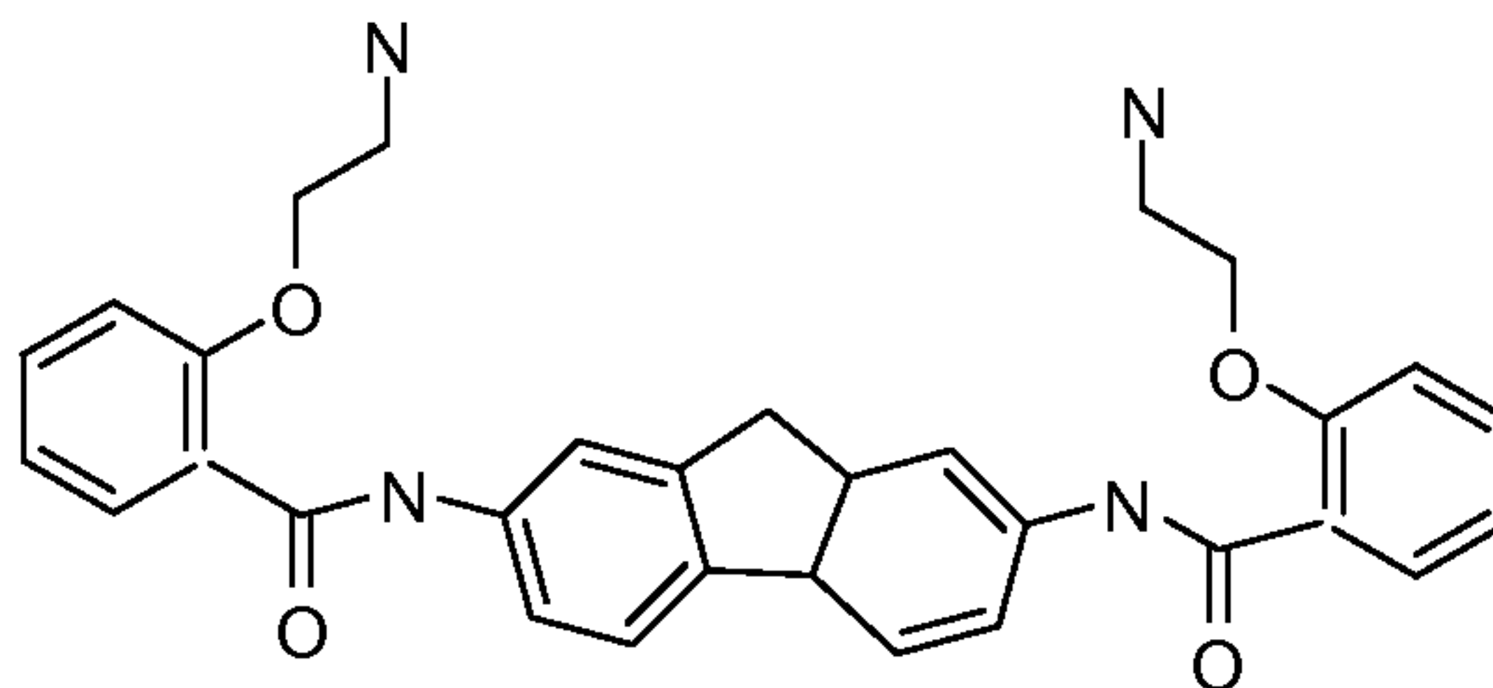
Compound 156
