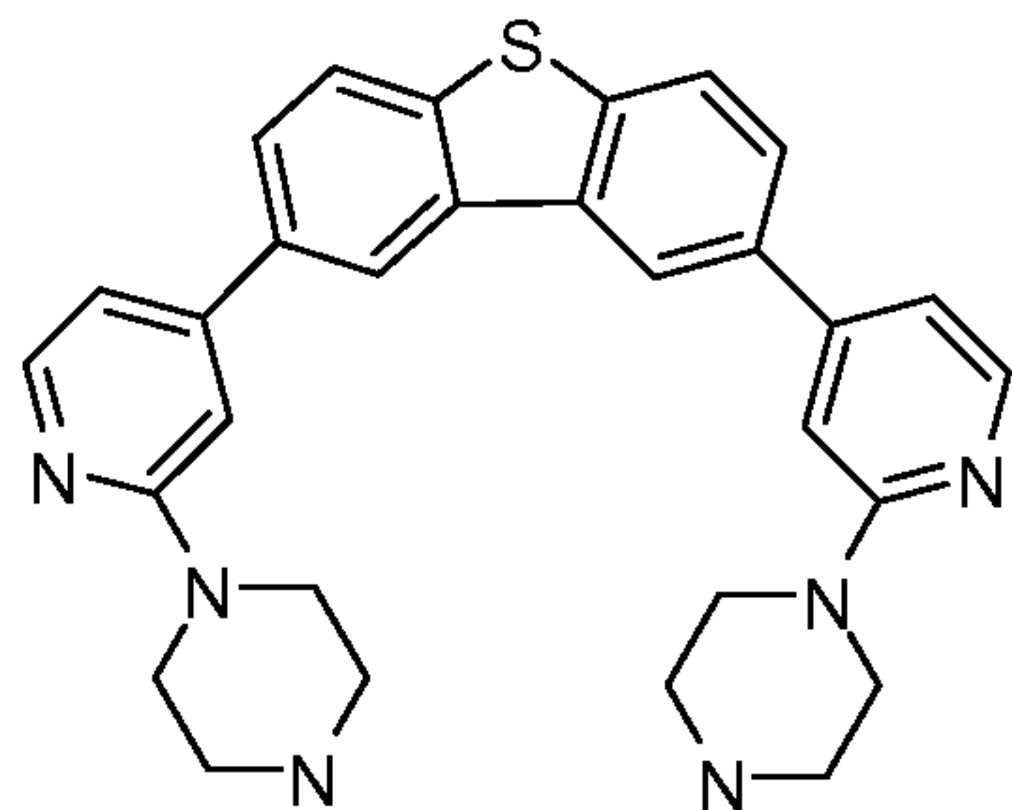
Compound 110
