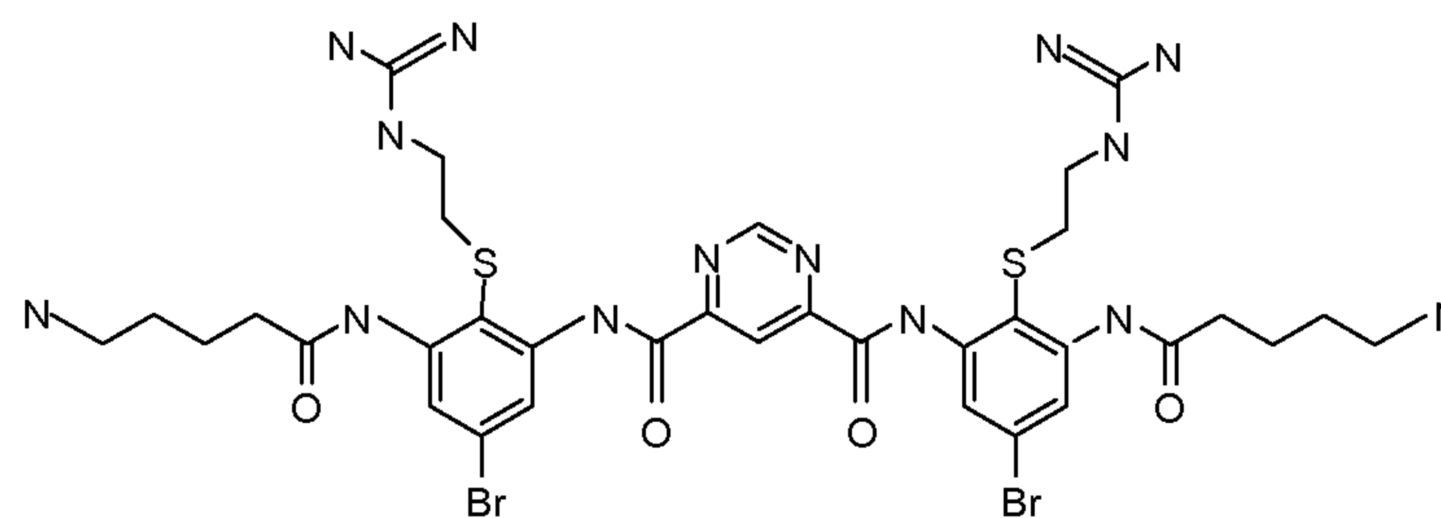
Compound 127
