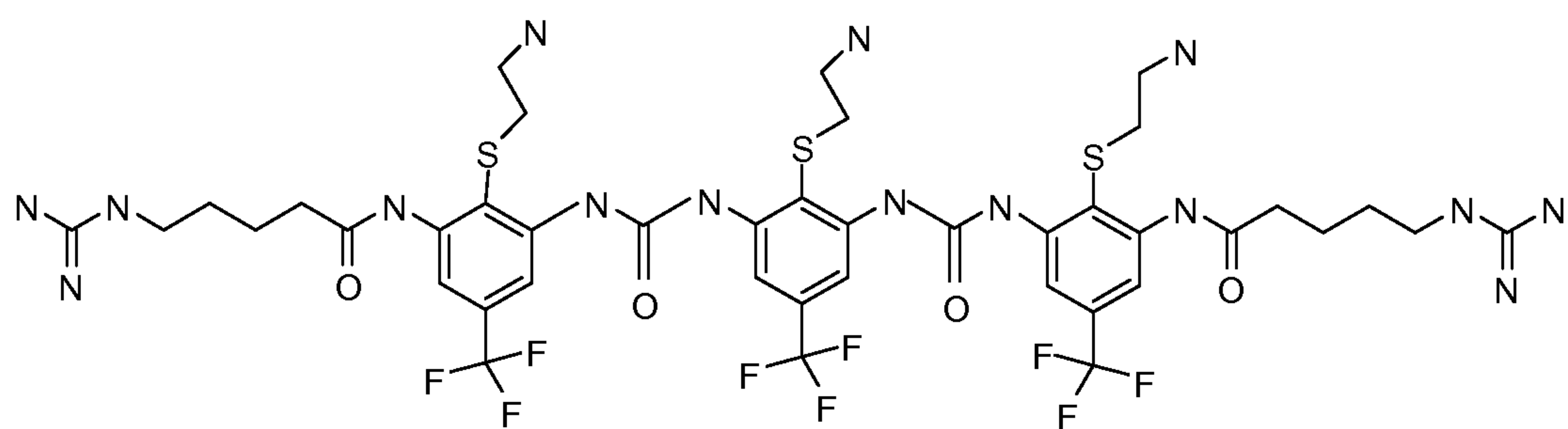
Compound 150
