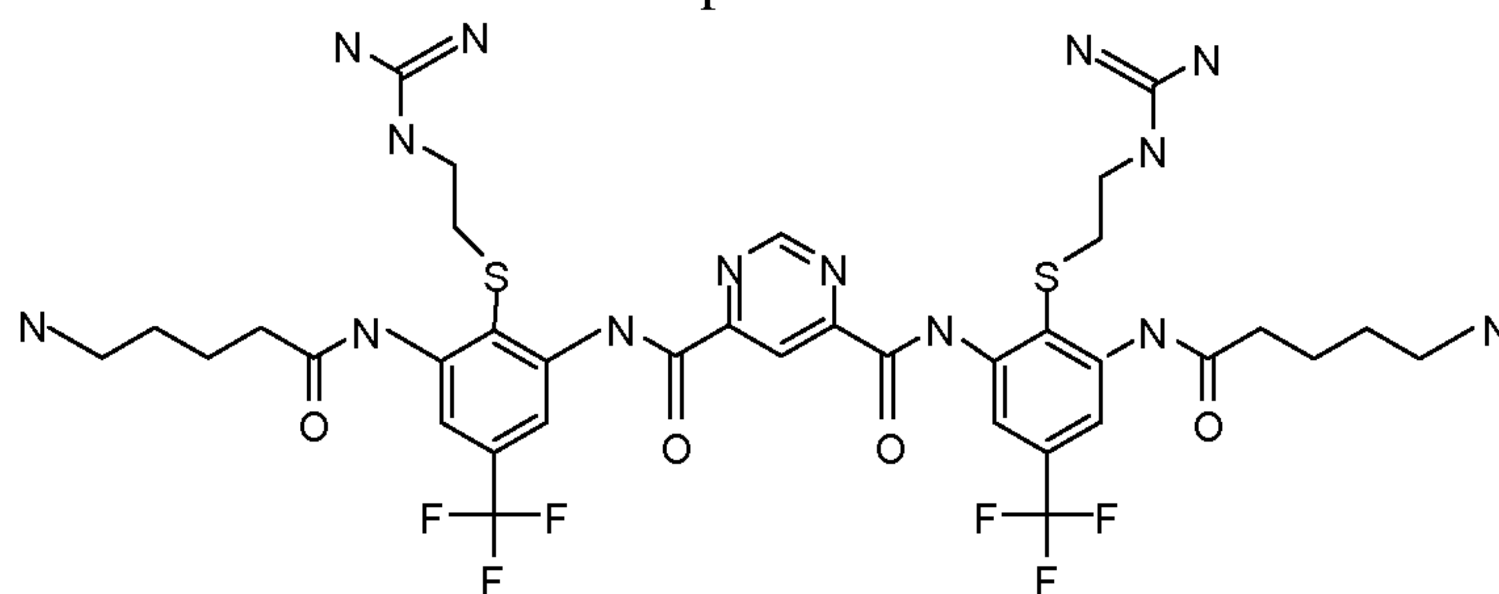
Compound 128
