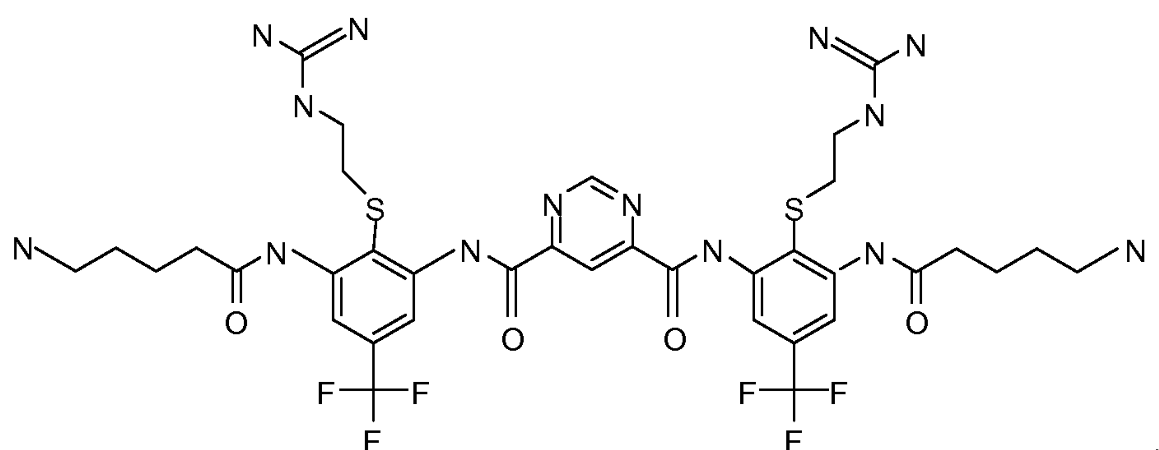
Compound 128
