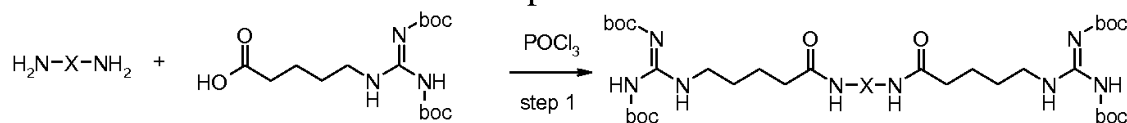
Compound 149
