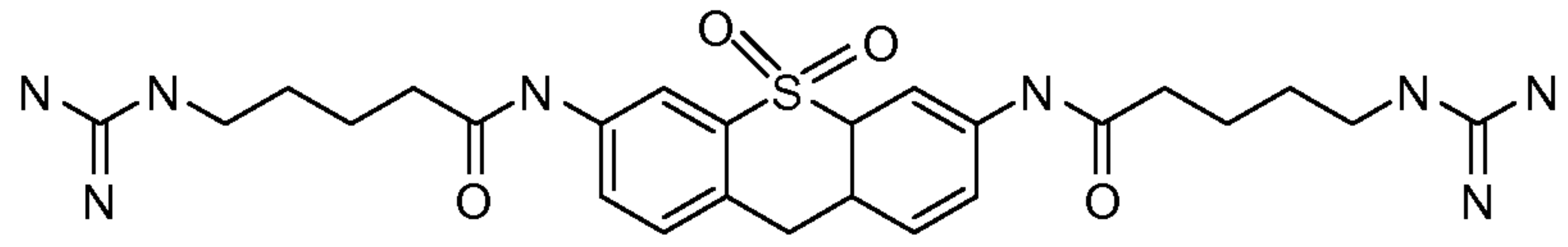
Compound 154
