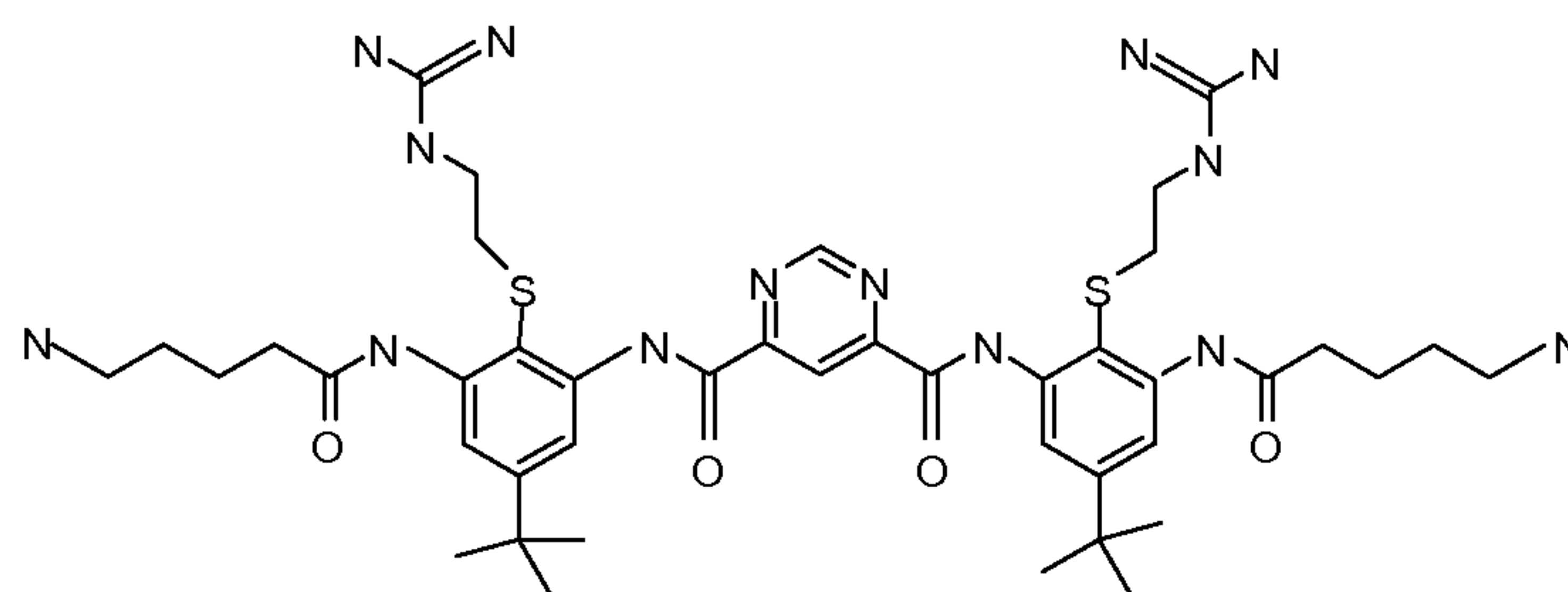
Compound 129
