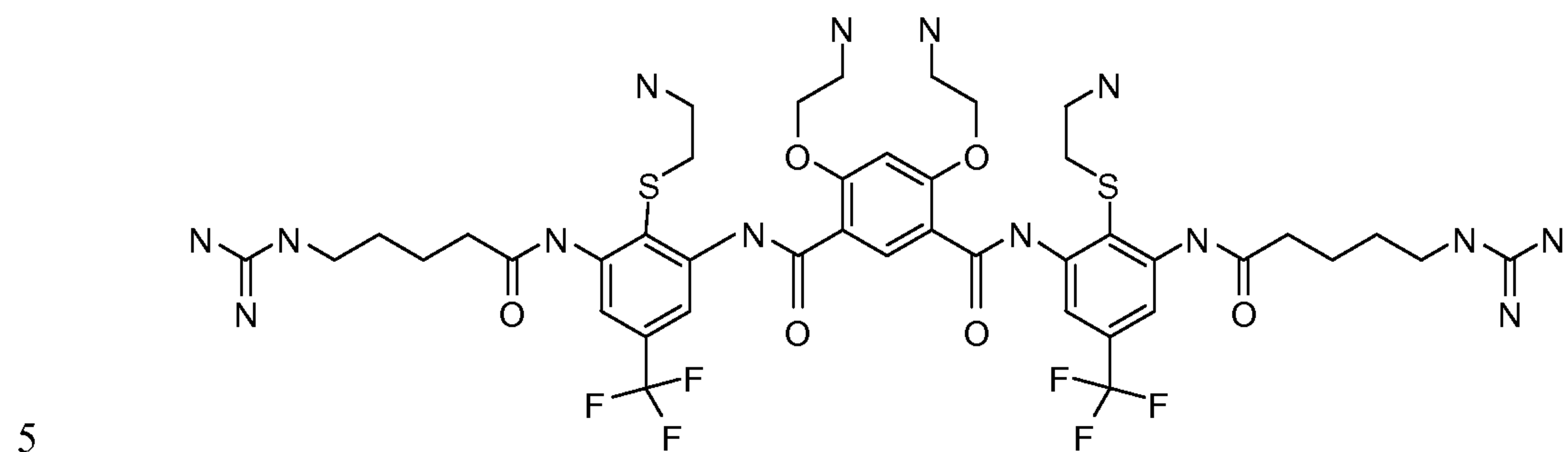
Compound 102
