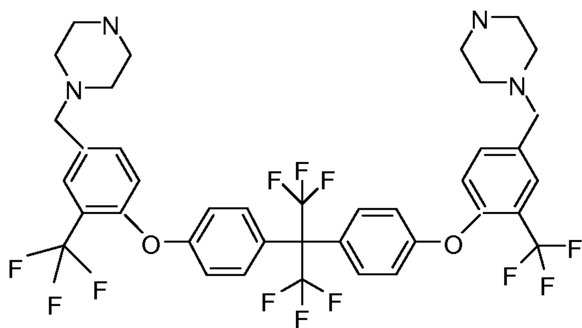
Compound 148
