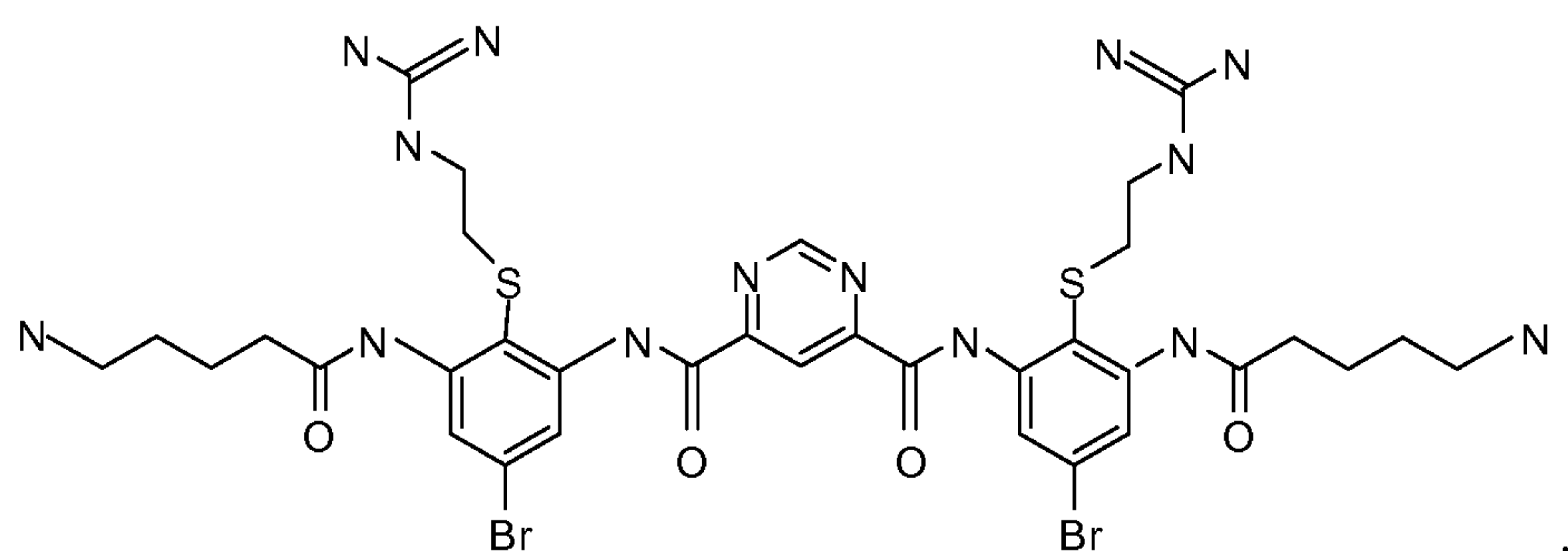
Compound 127
