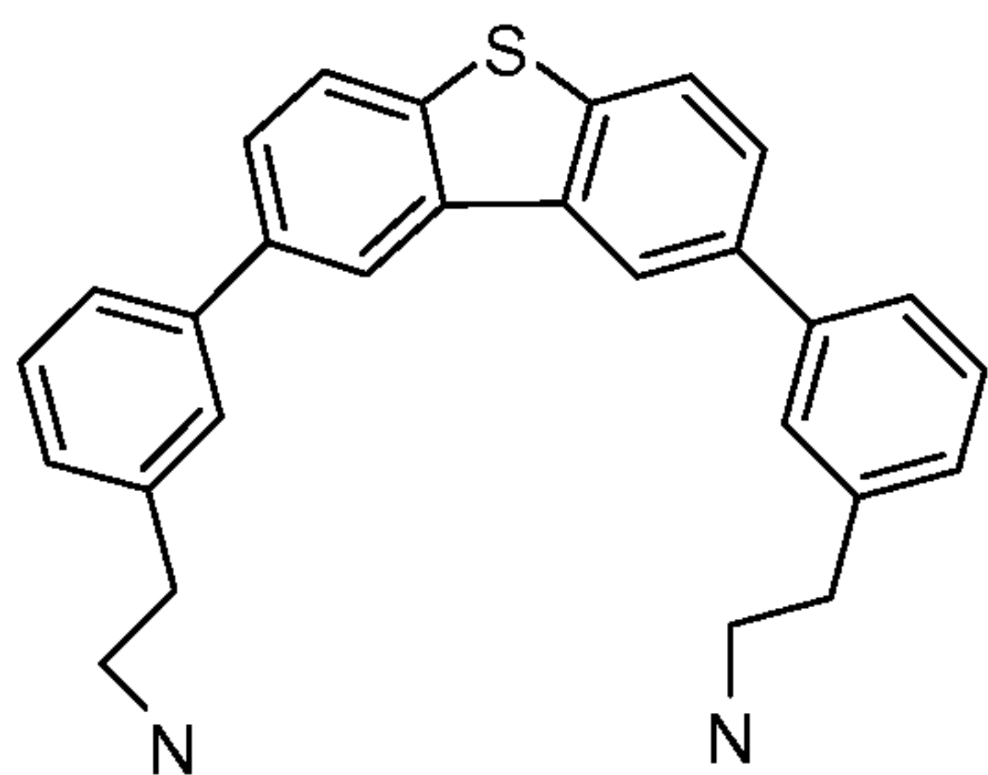
Compound 106
