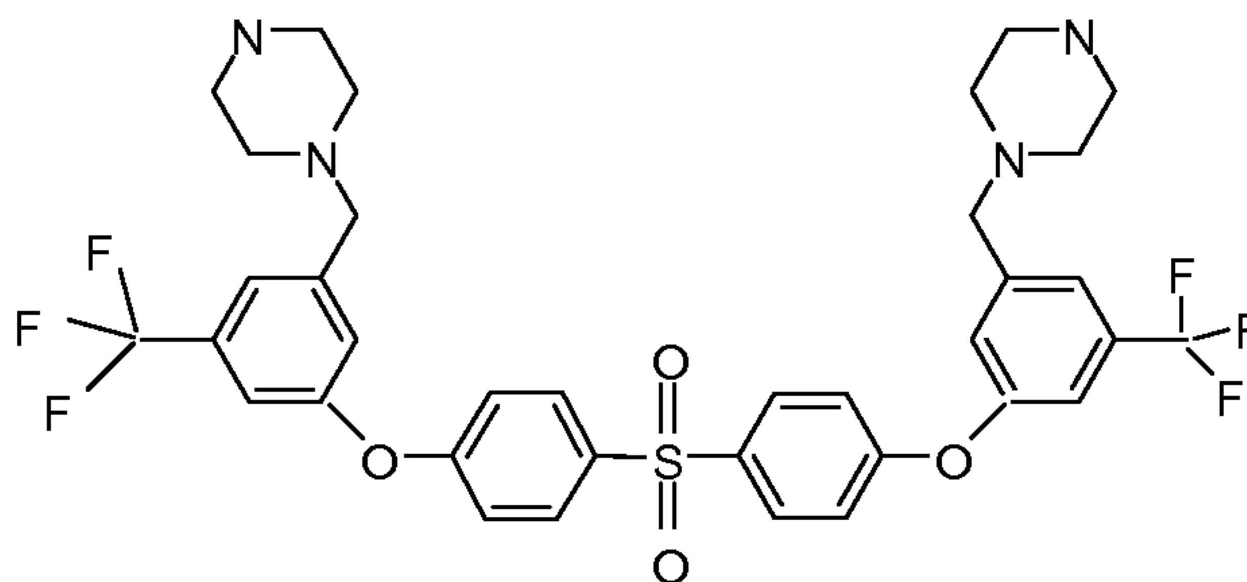
Compound 146
