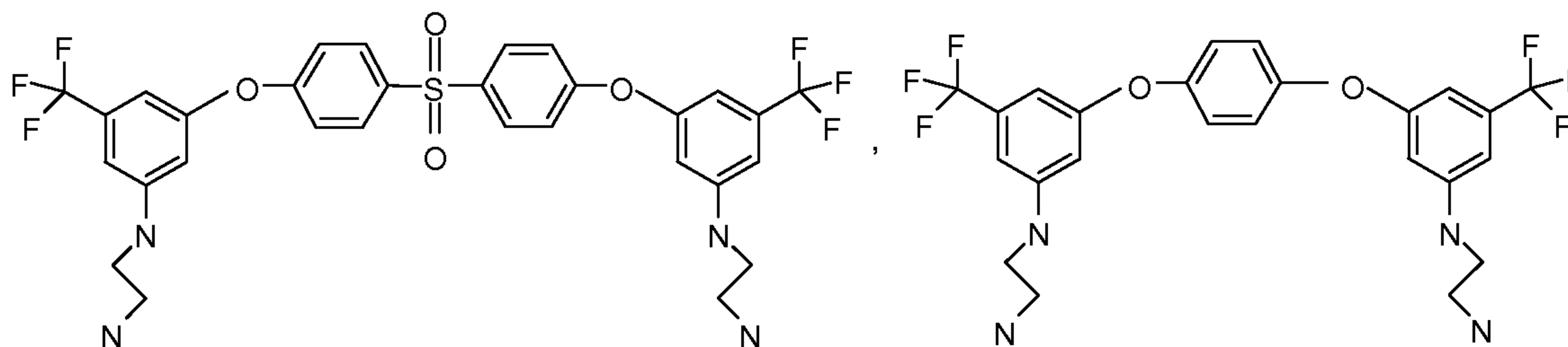
Compound 111
