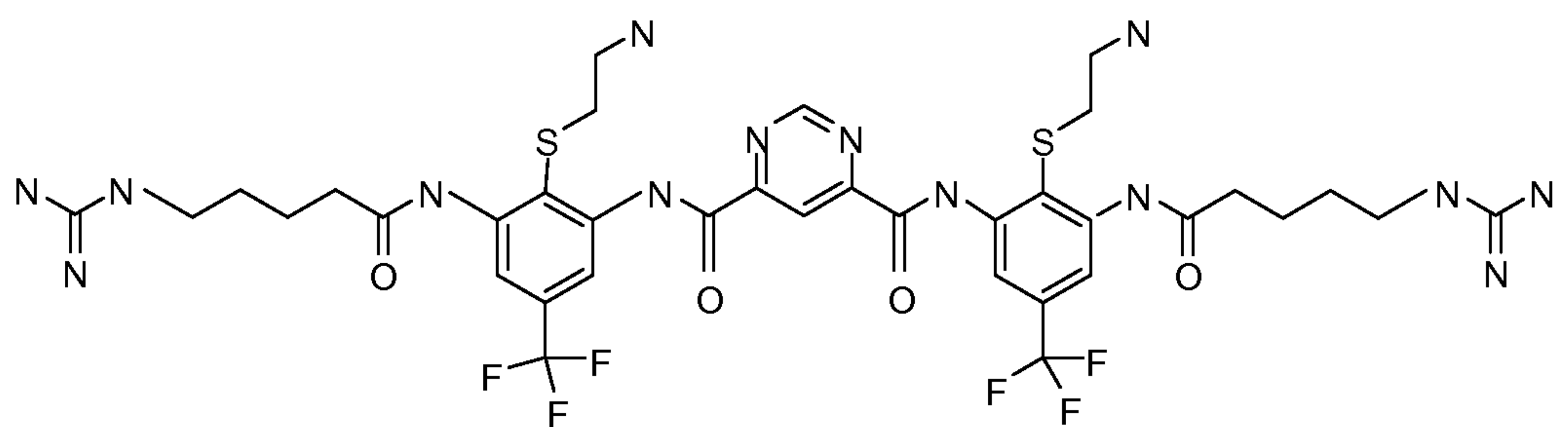
Compound 121
