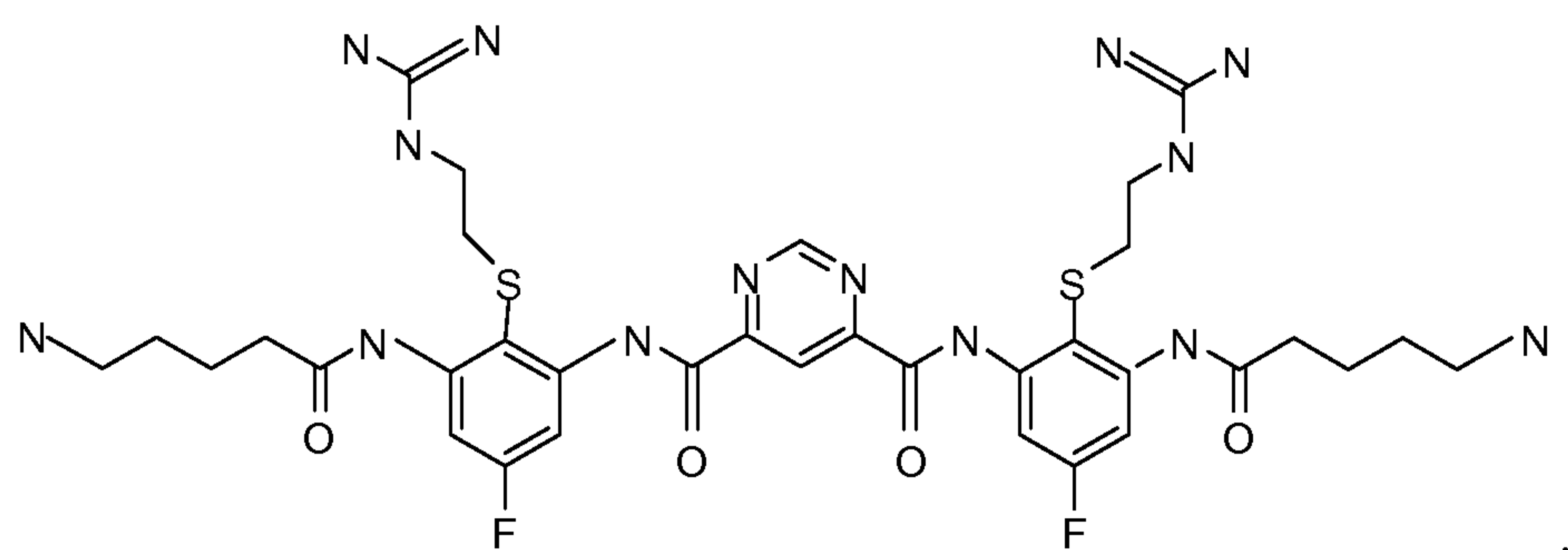
Compound 126
