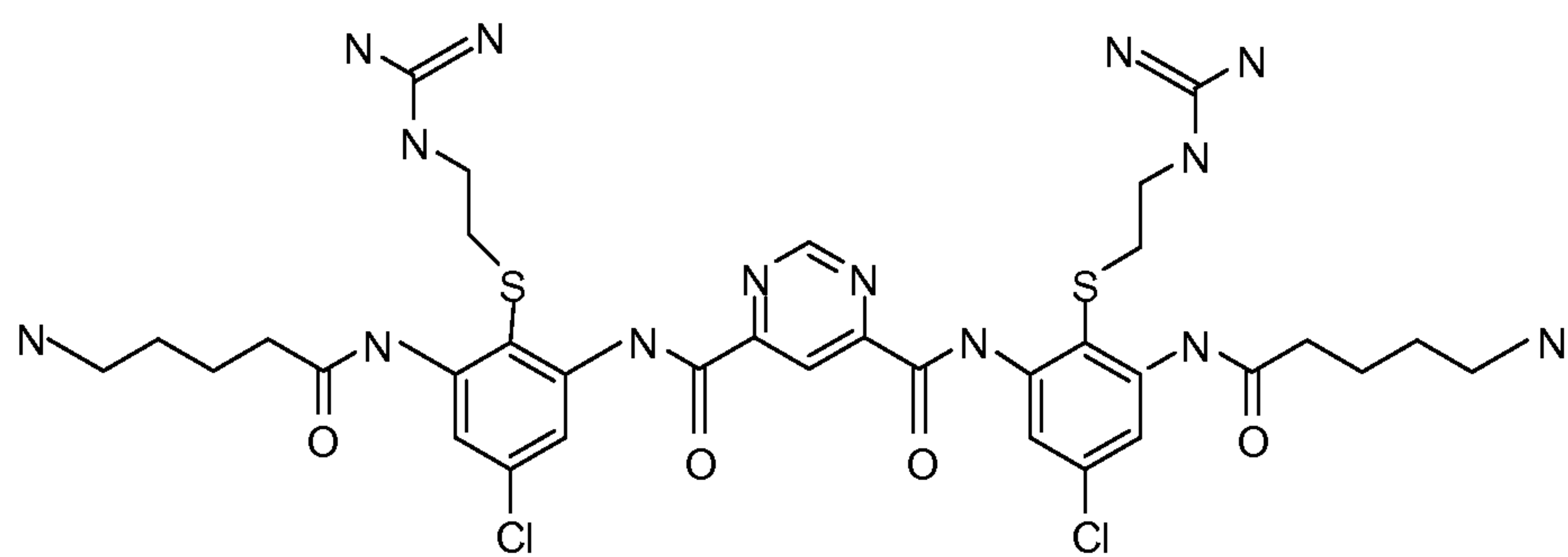
Compound 122
