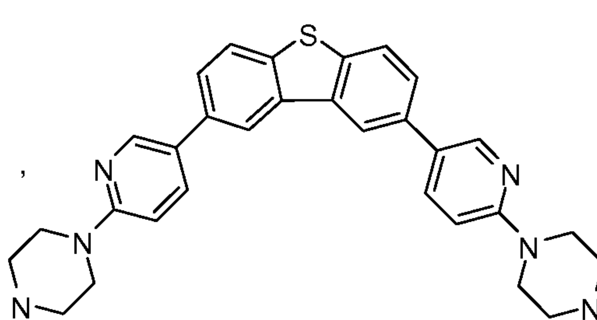
Compound 117
