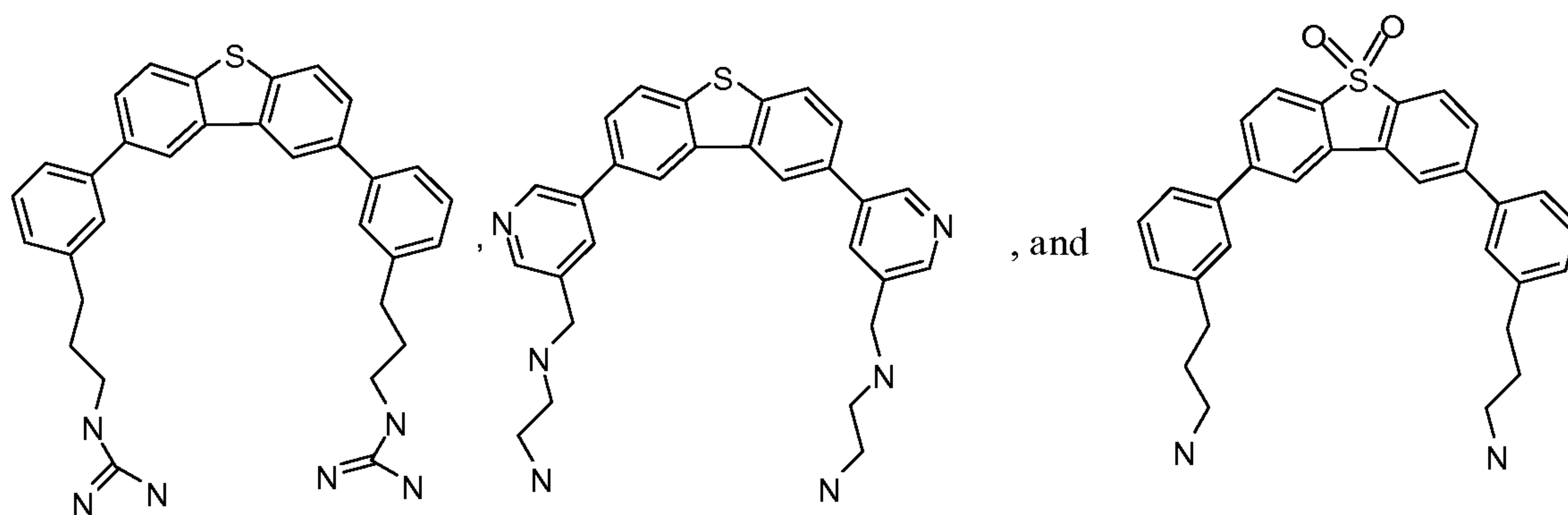
Compound 139
