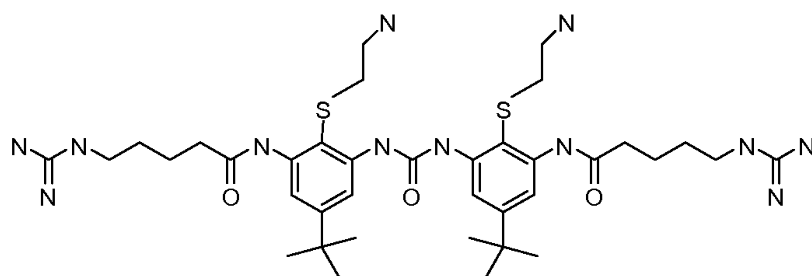
Compound 103
