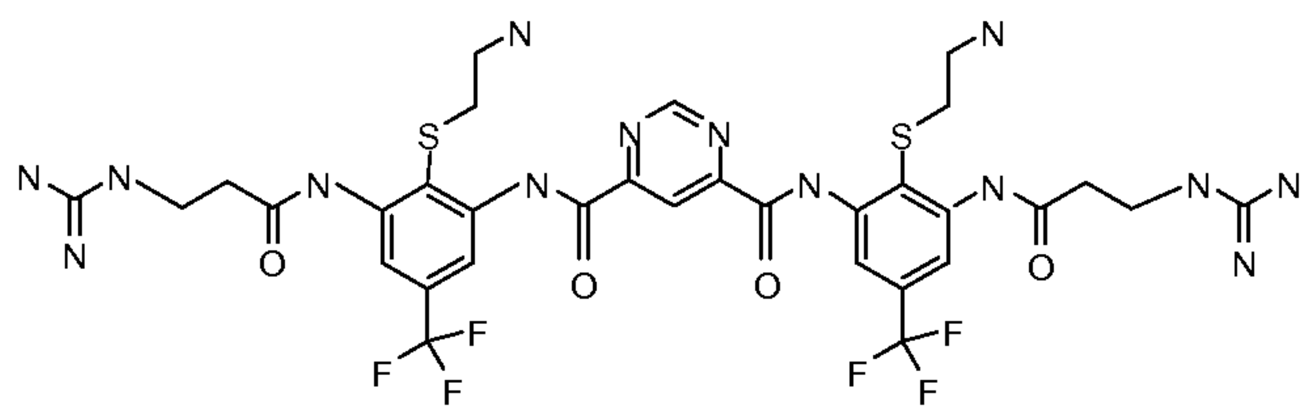
Compound 108
