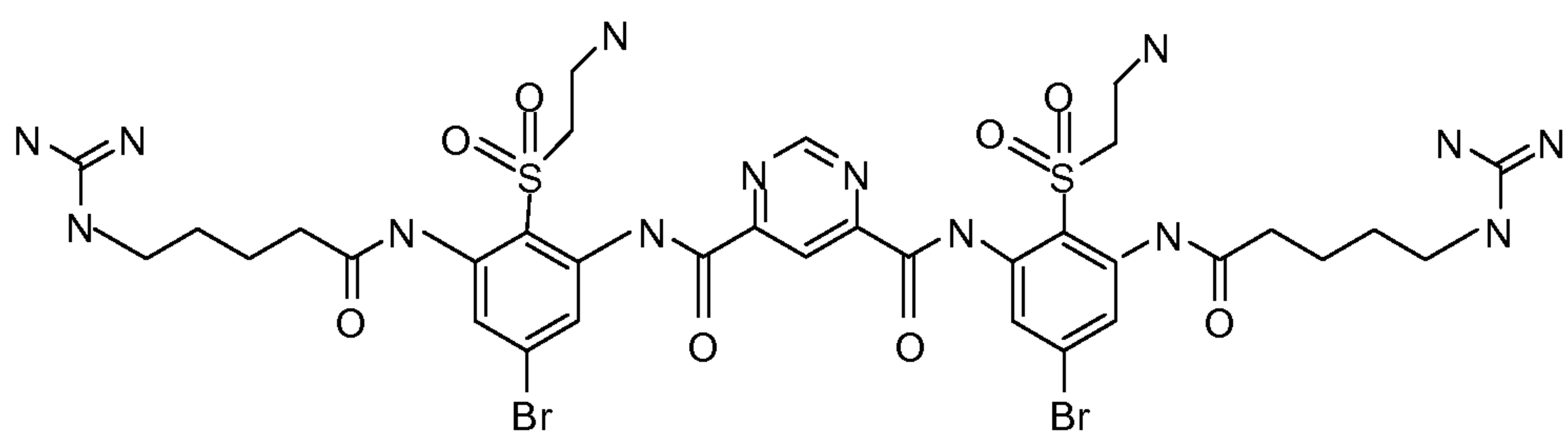
Compound 152, and
