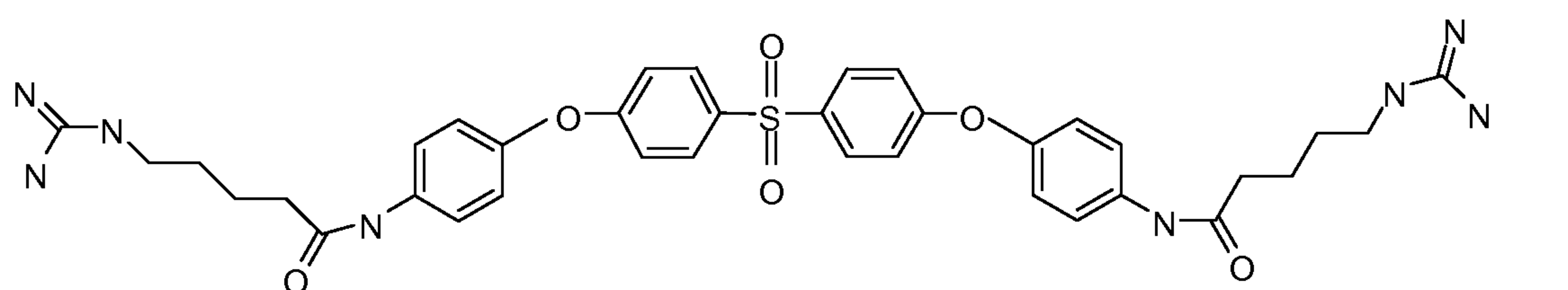
Compound 142
