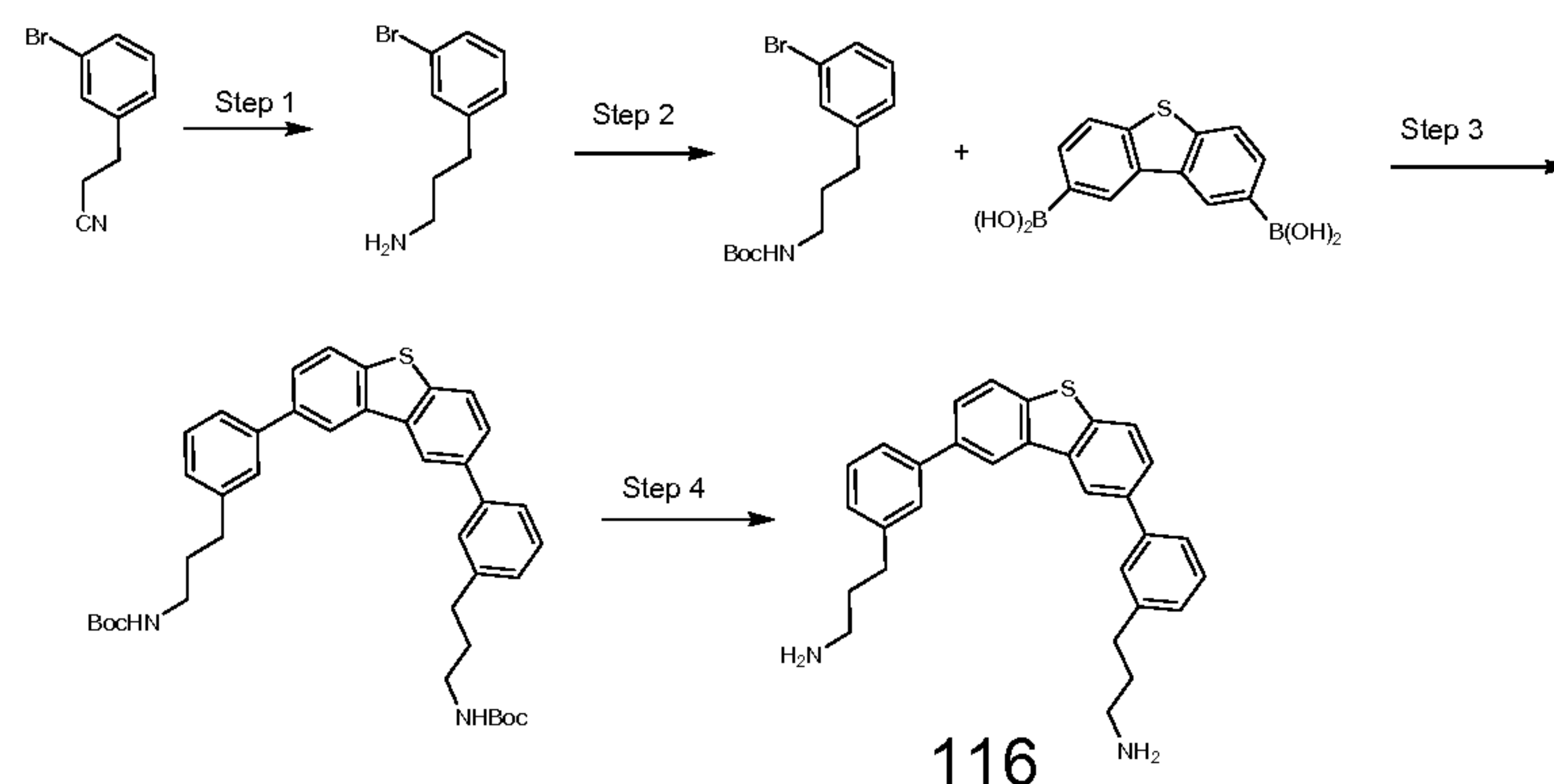
Scheme 2
