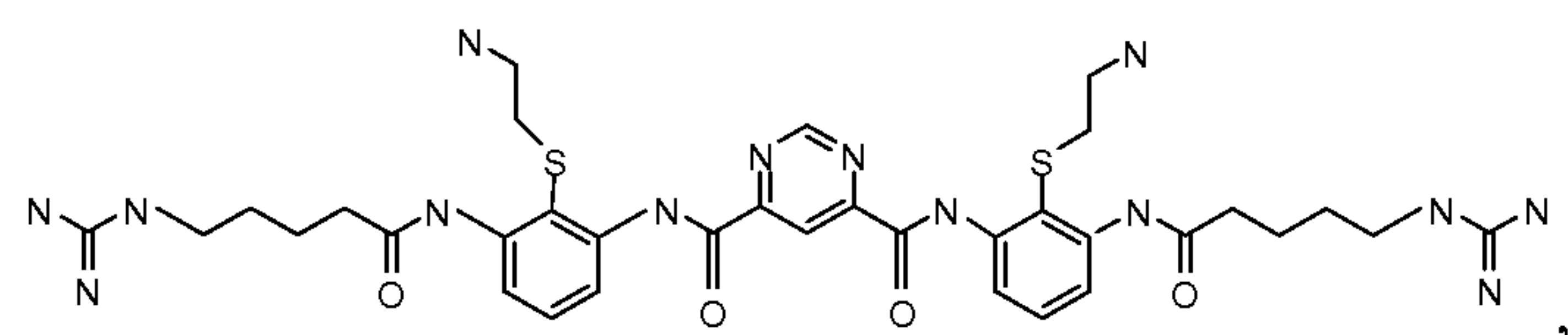
Compound 113
