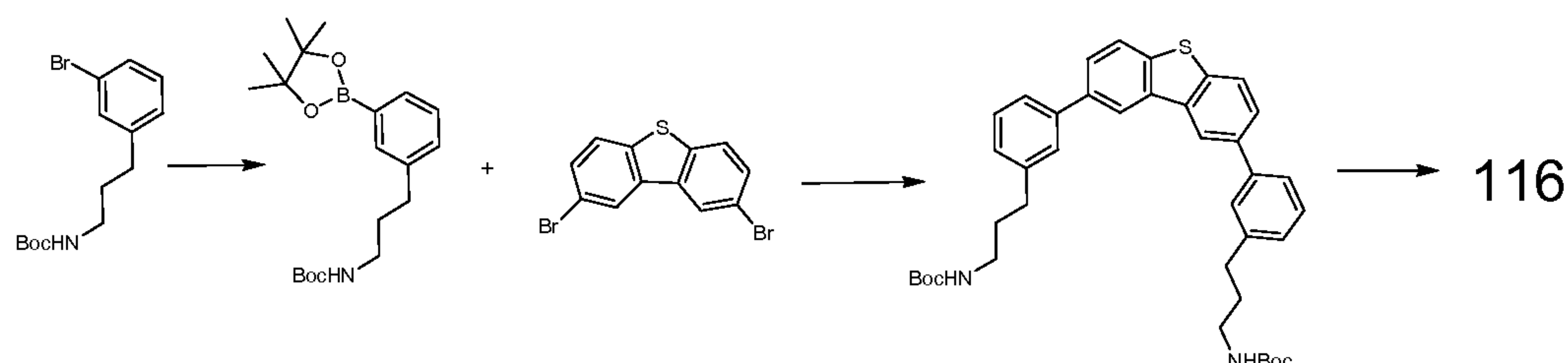
Scheme 3
