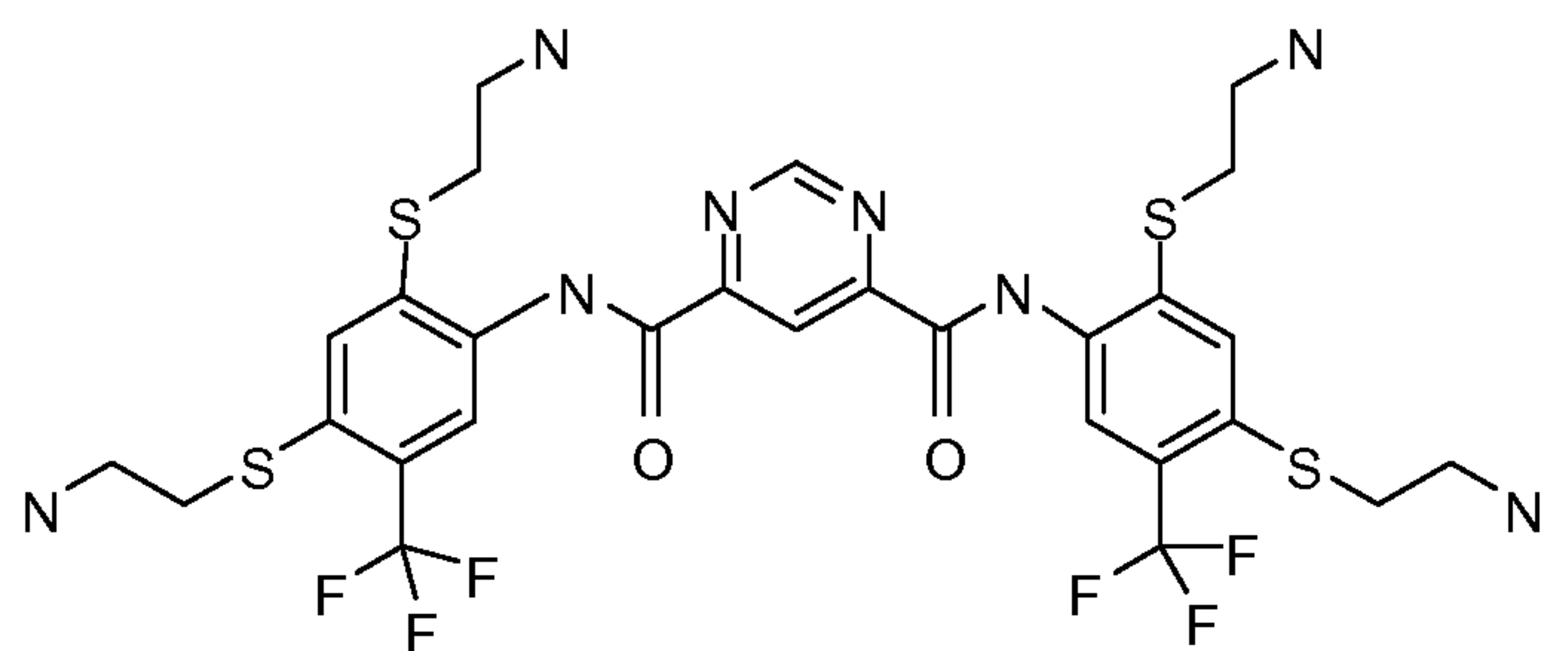
Compound 112
