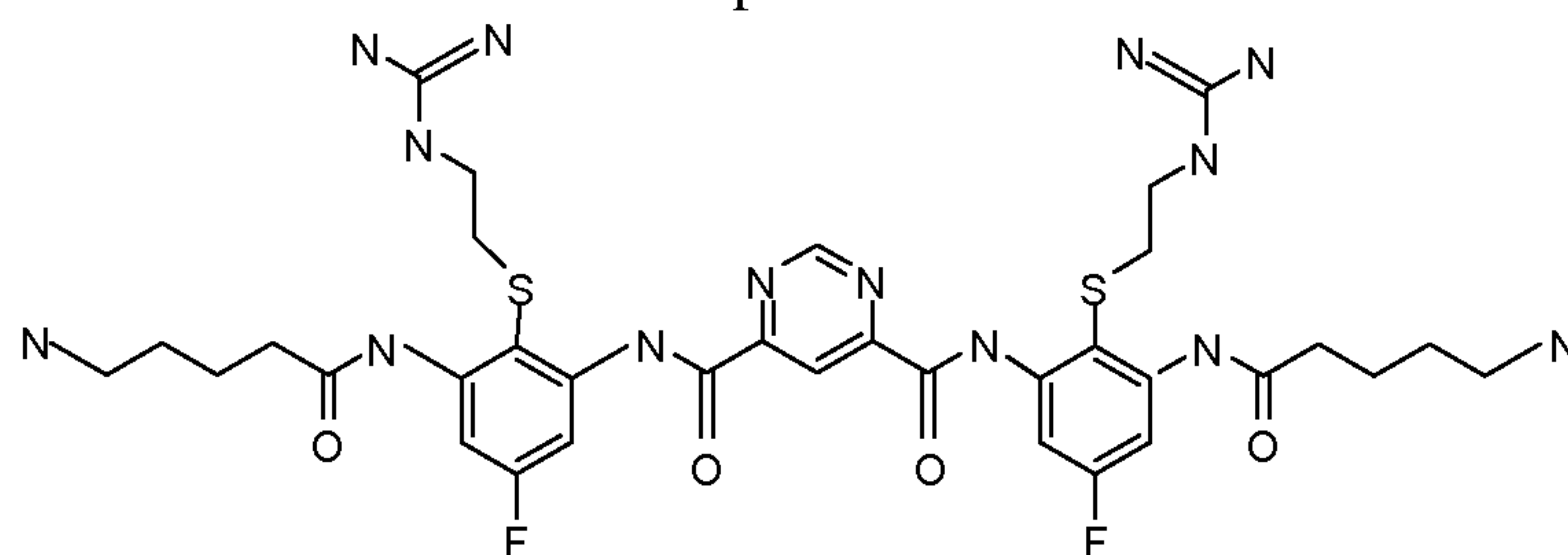
Compound 126
