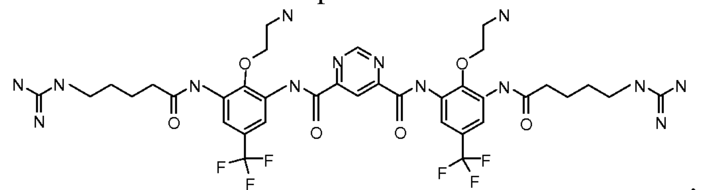
Compound 114
