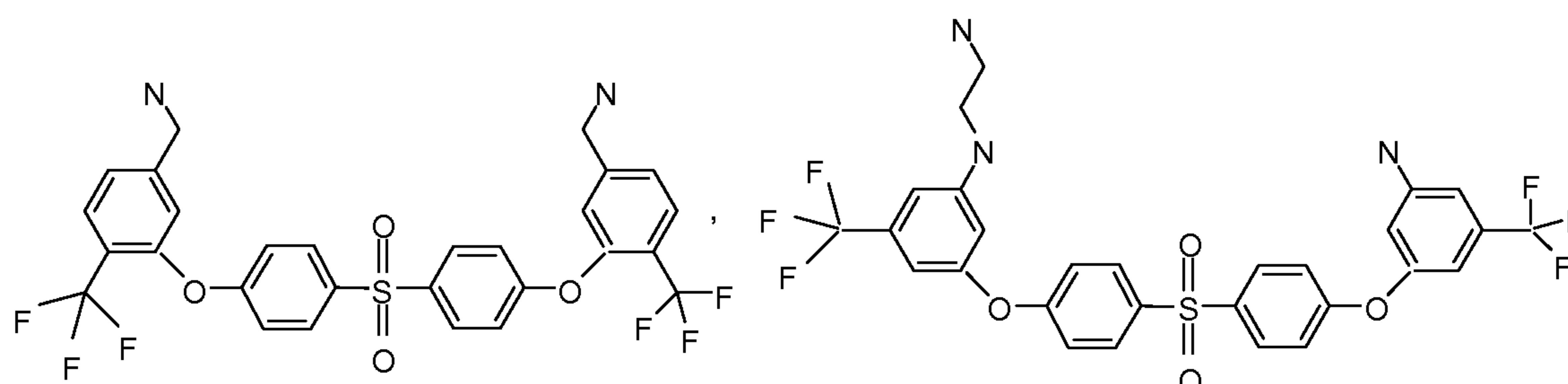
Compound 143
