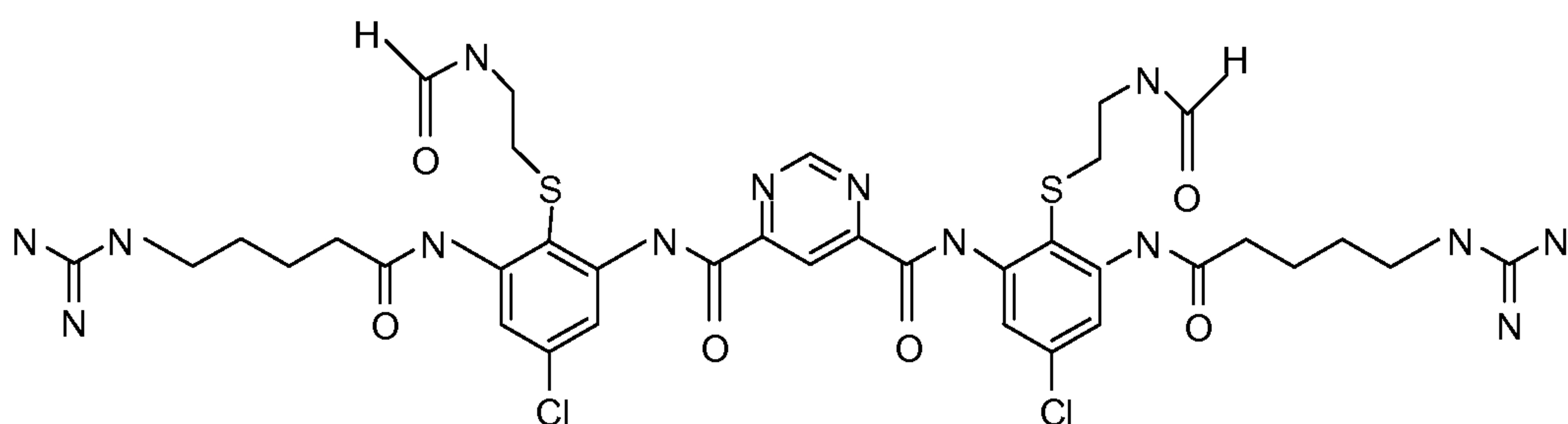
Compound 125
