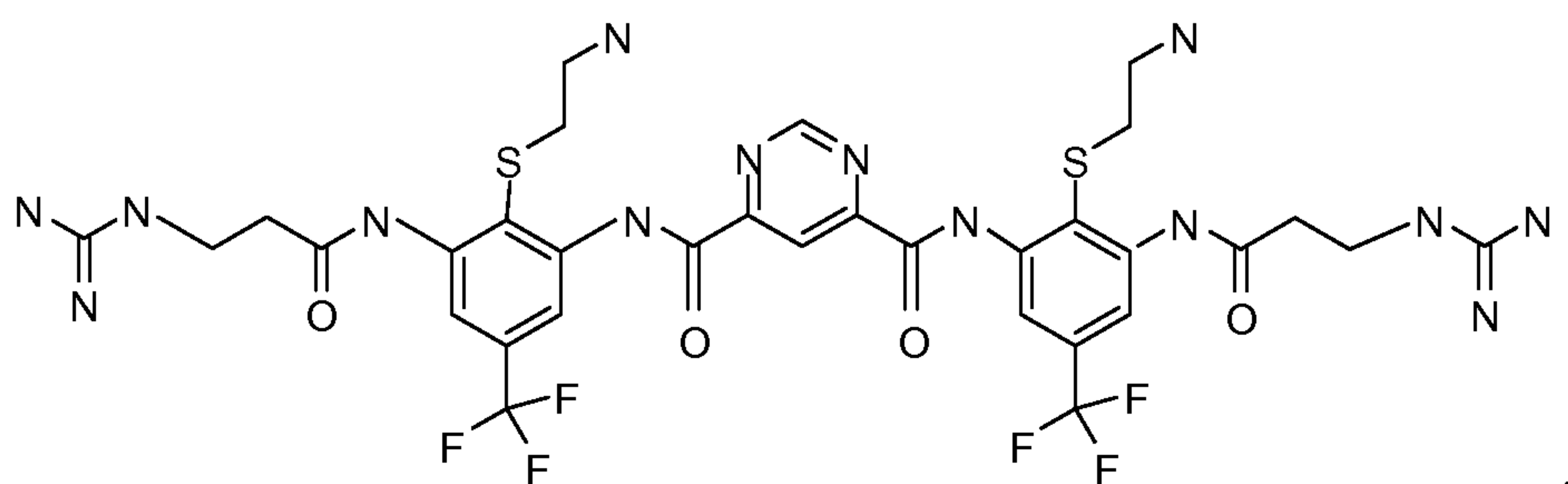
Compound 108
