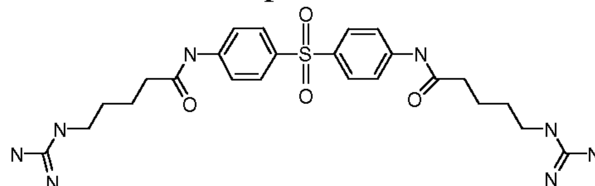
Compound 149
