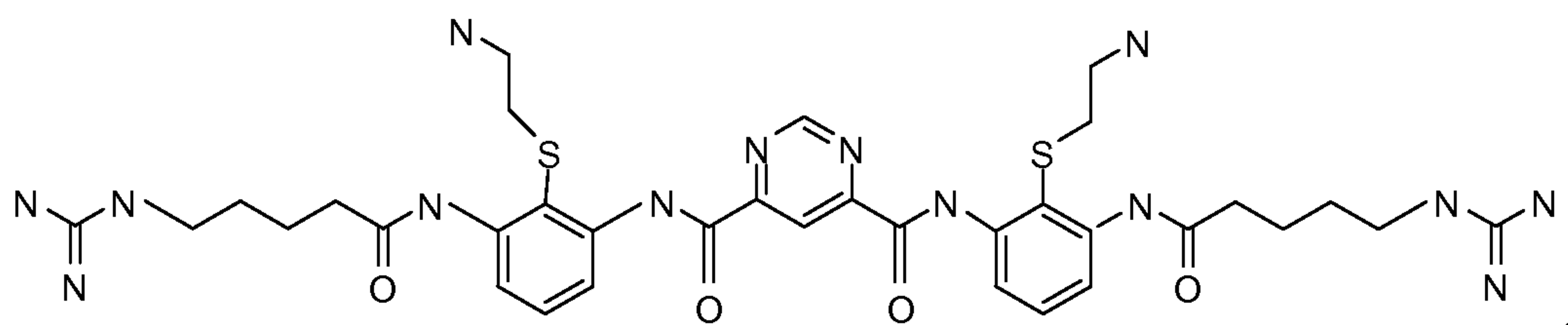
Compound 113
