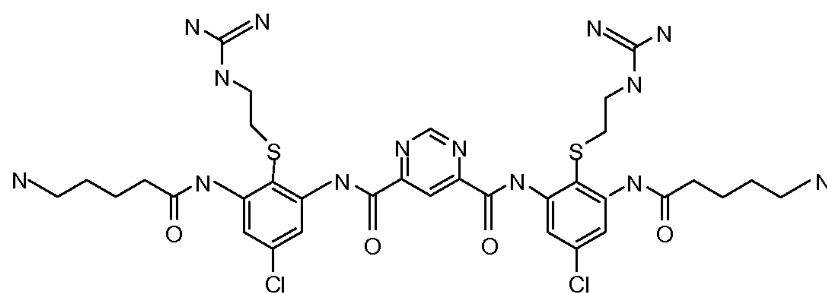
Compound 122
