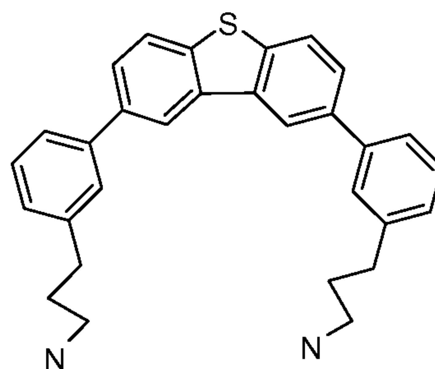
Compound 116
