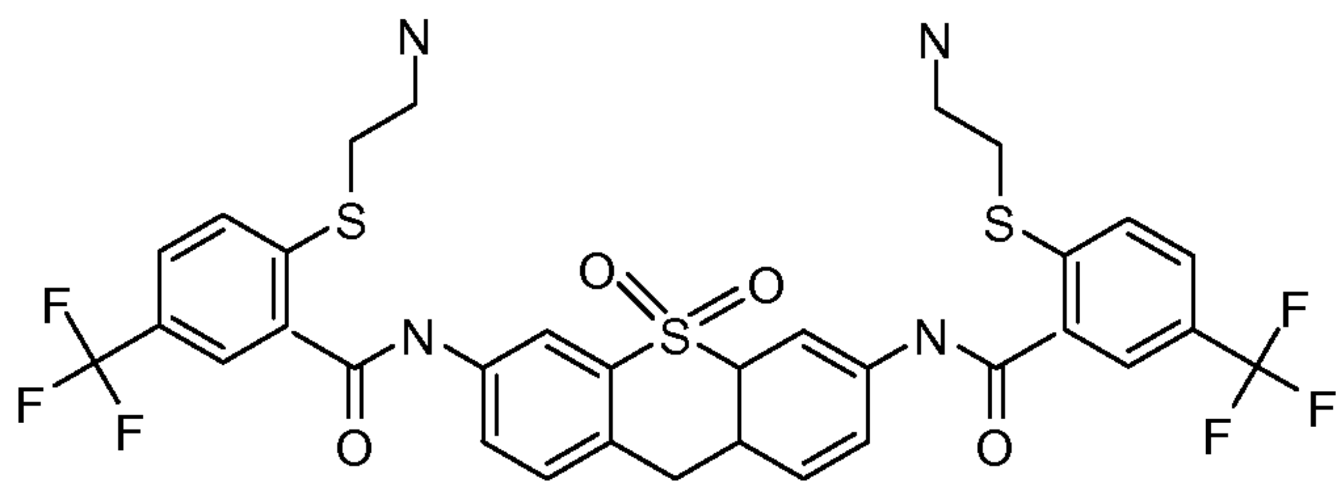
Compound 155 and
