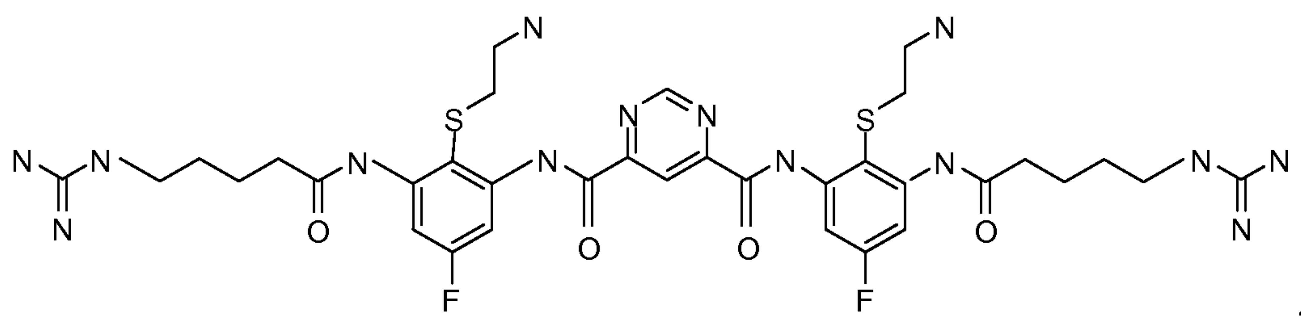
Compound 107
