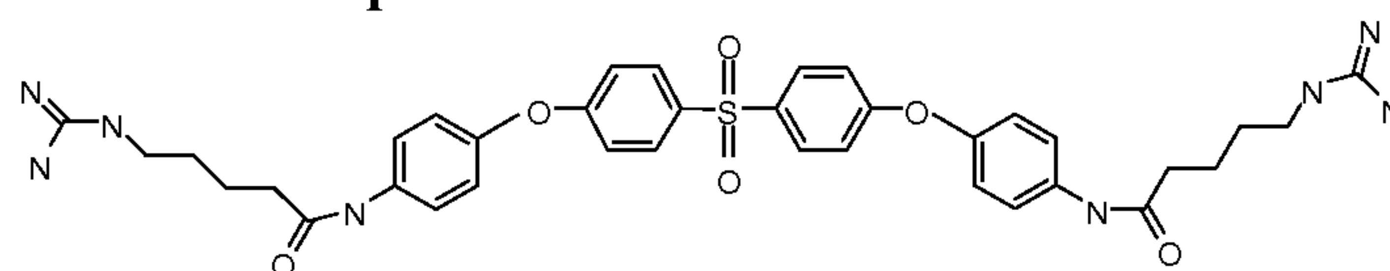
Compound 142
