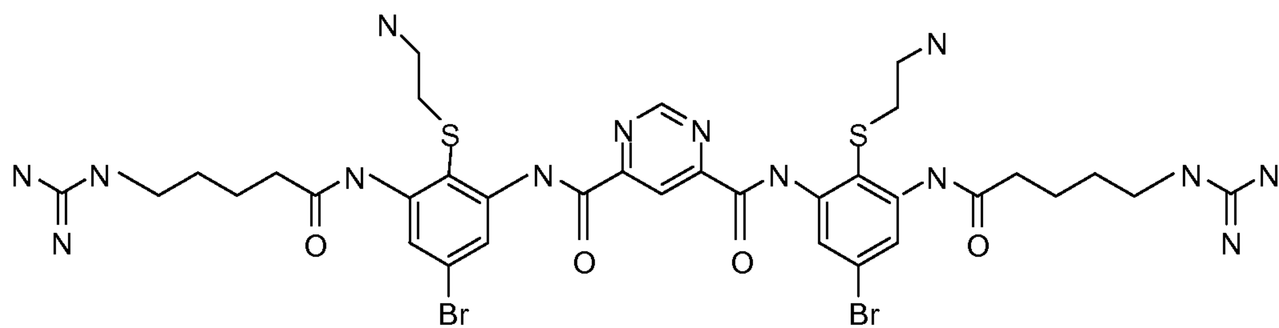
Compound 123
