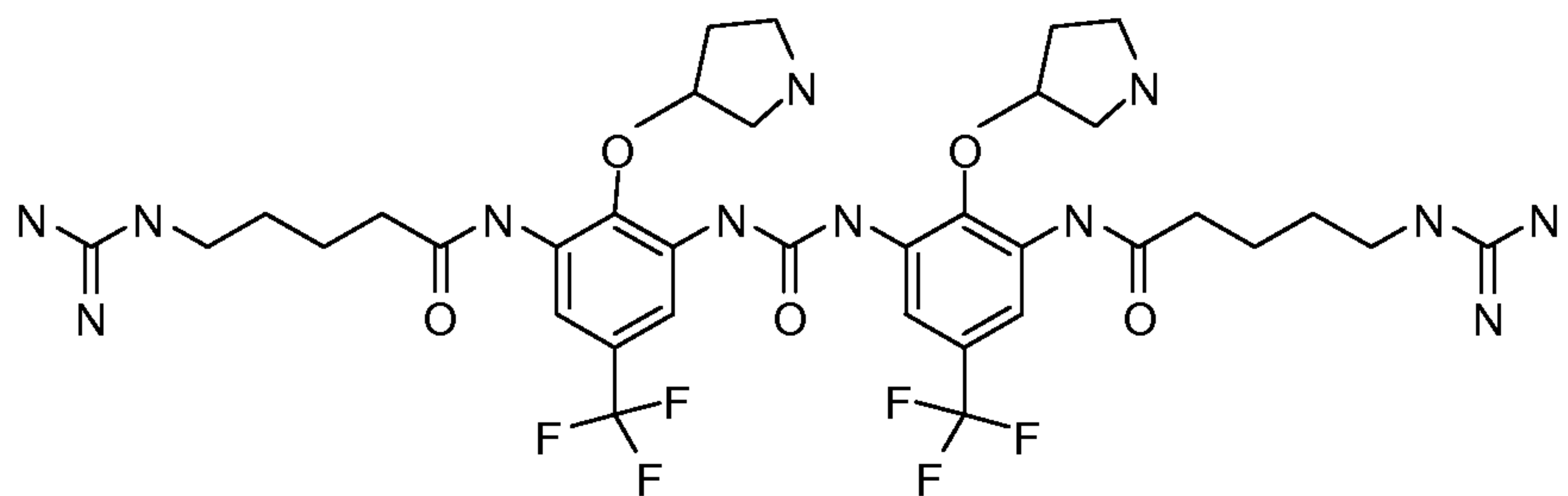
Compound 104
