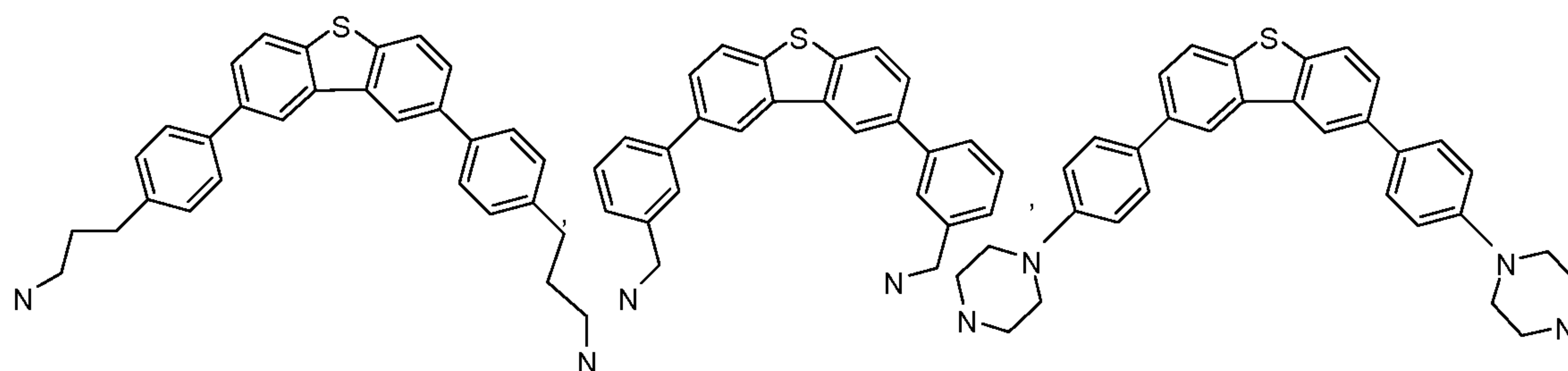
Compound 130
