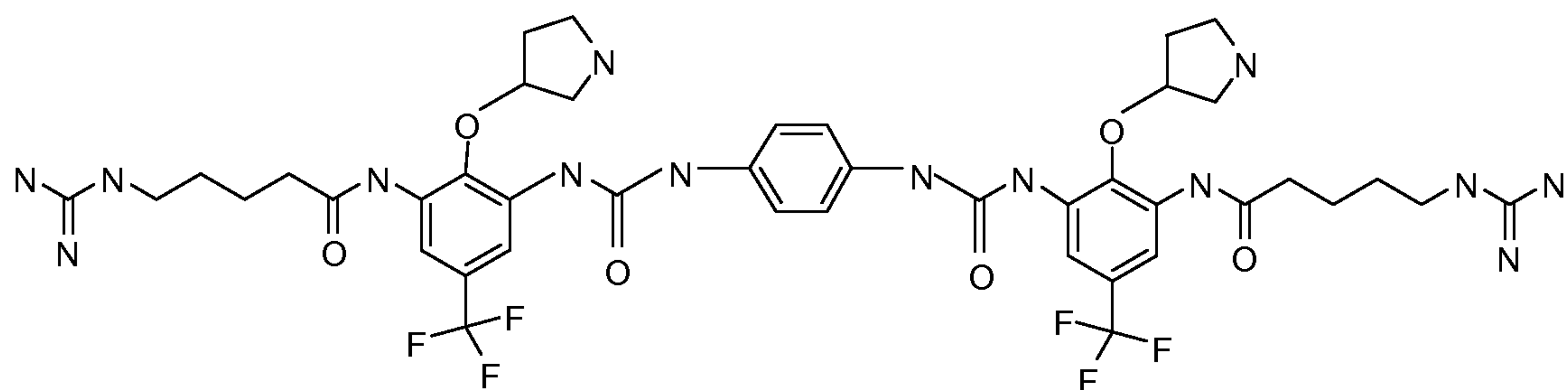
Compound 151
