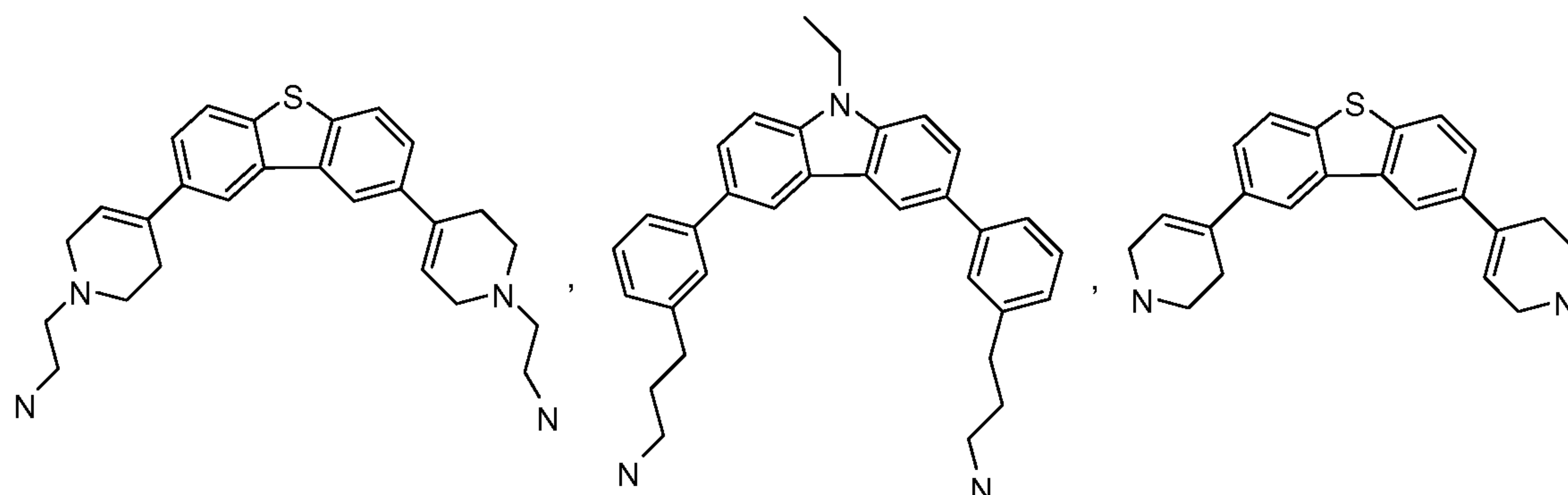
Compound 136
