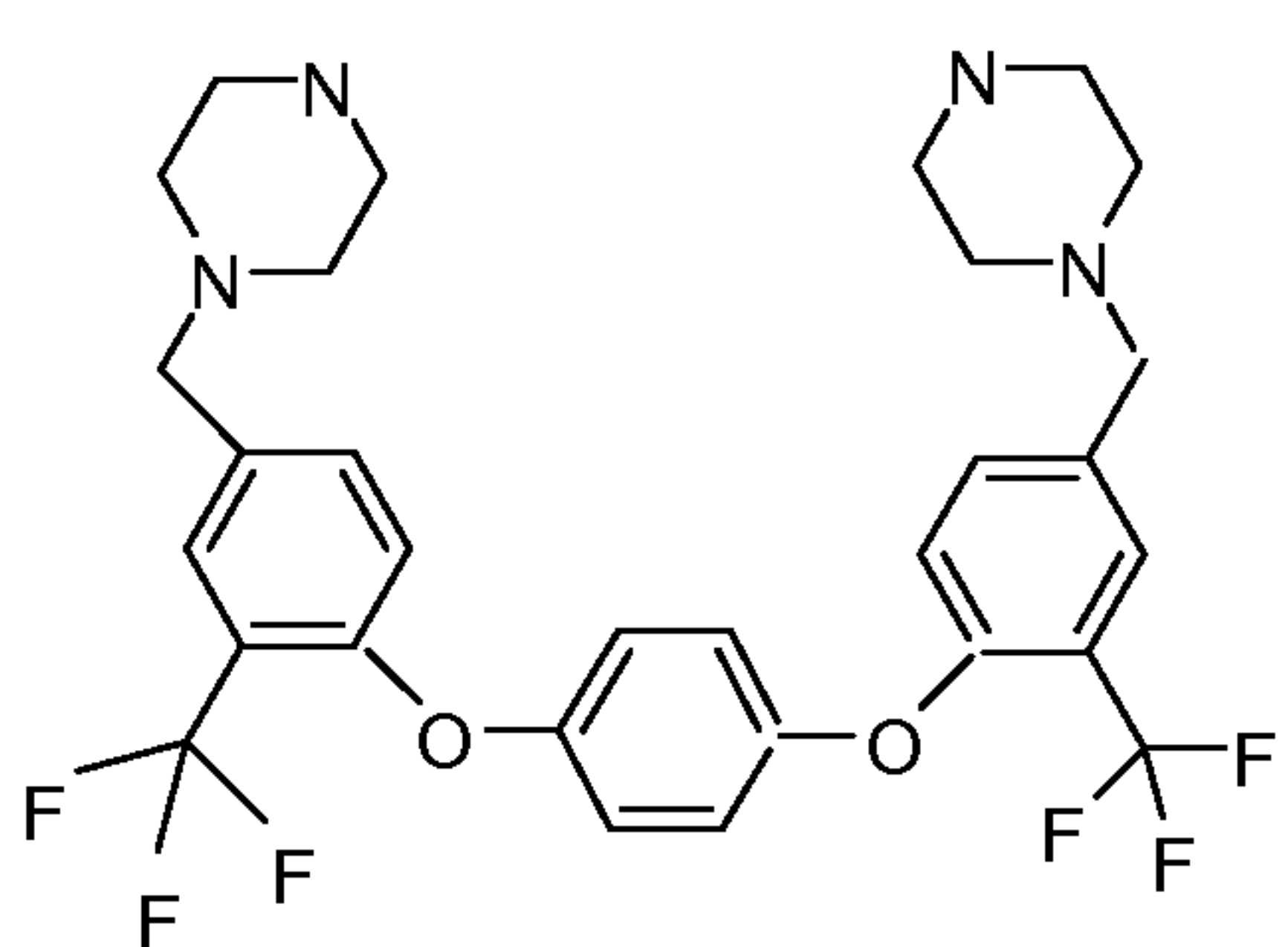
Compound 147
