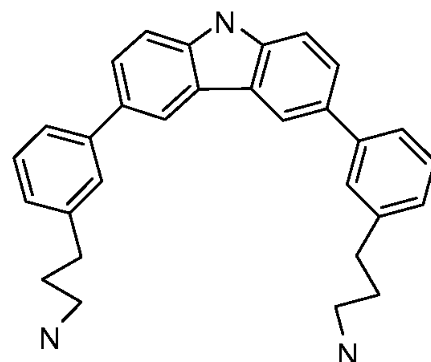
Compound 119
