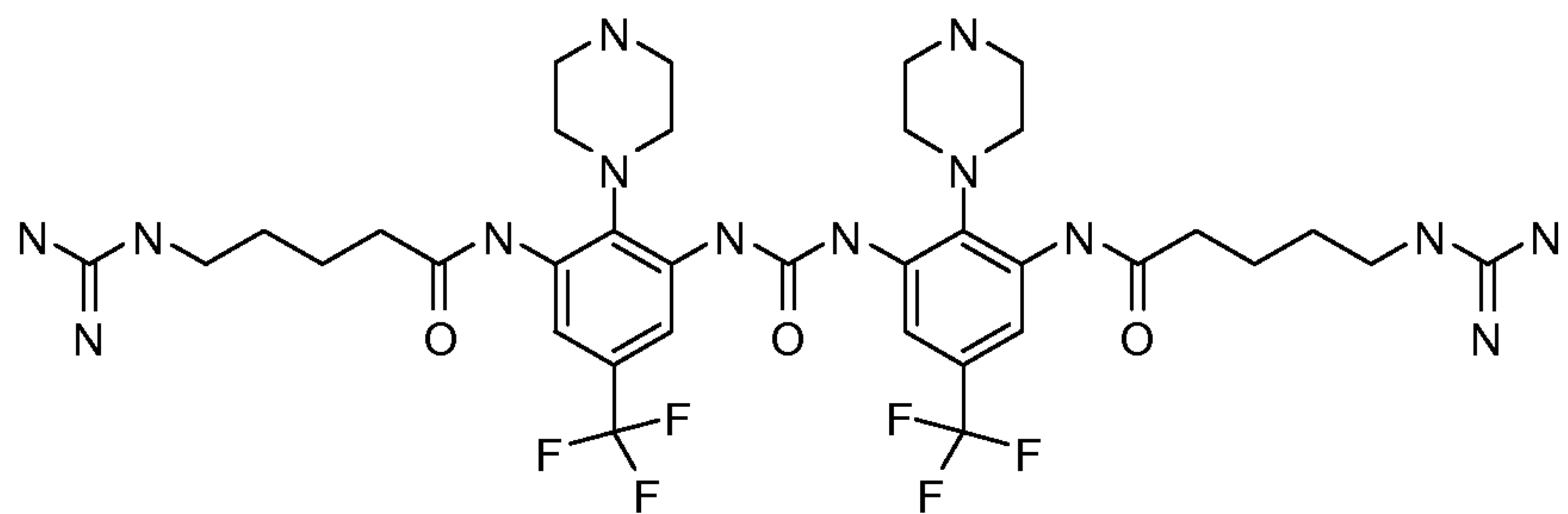
Compound 105
