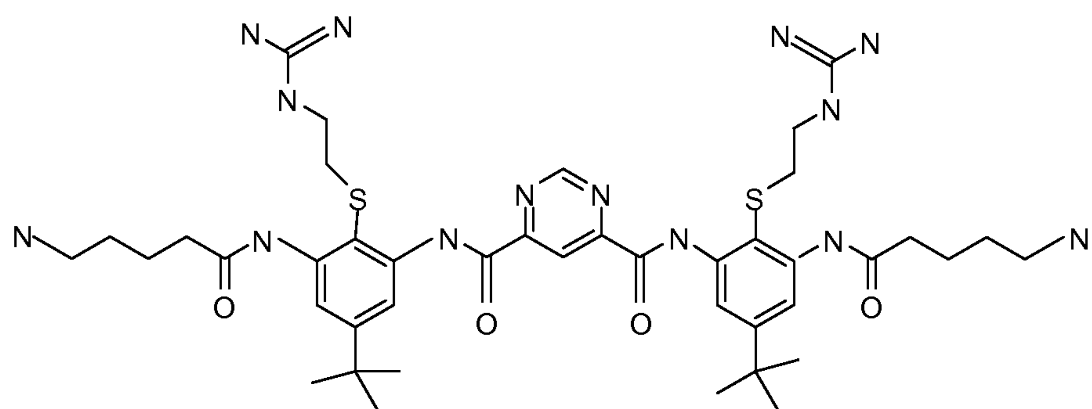
Compound 129
