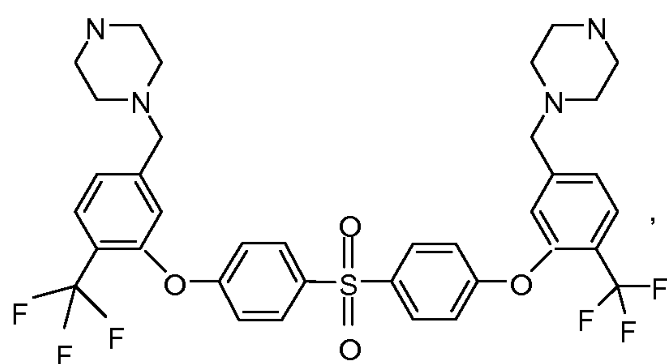
Compound 145
