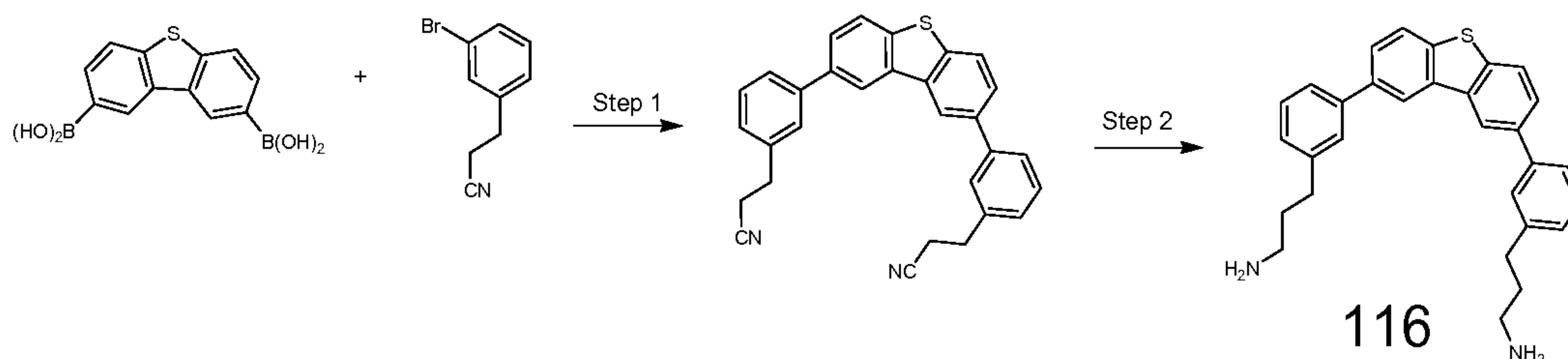
Scheme 1
