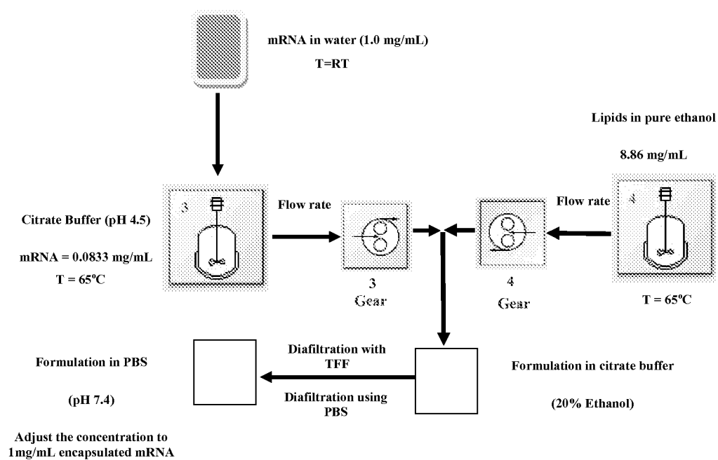
Figure 3. Scaled-Up Formulation Process with Homogenous Flow Pumps.
