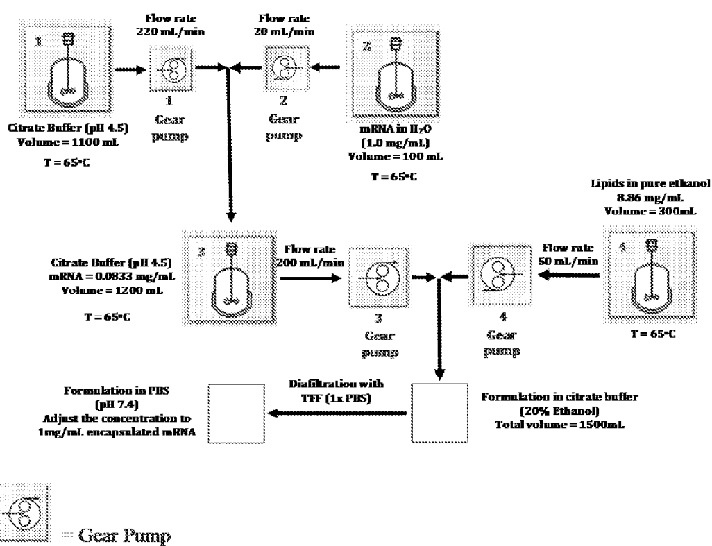
Figure 1. Scaled-Up Formulation Process with Homogenous Flow Pumps
