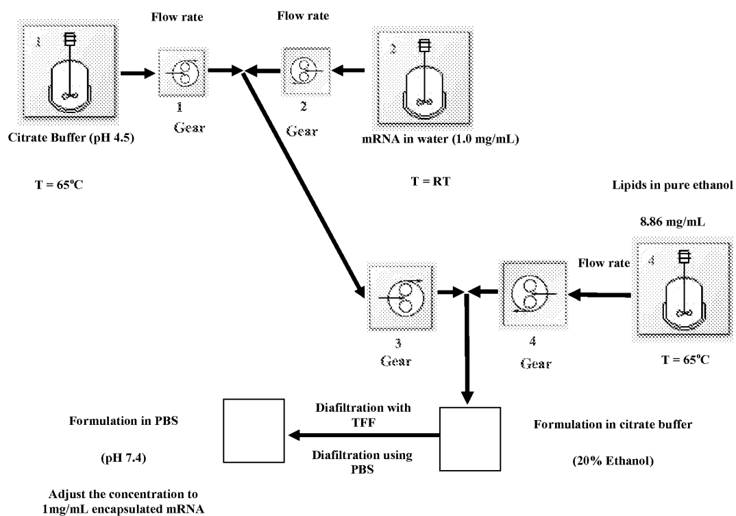
Figure 2. Scaled-Up Formulation Process with Homogenous Flow Pumps
