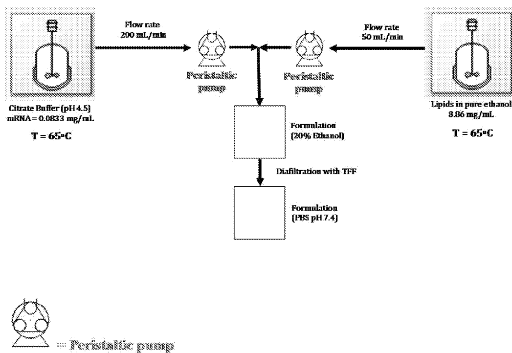
Figure 5 Scaled-Up Formulation Process with Peristaltic Pumps
