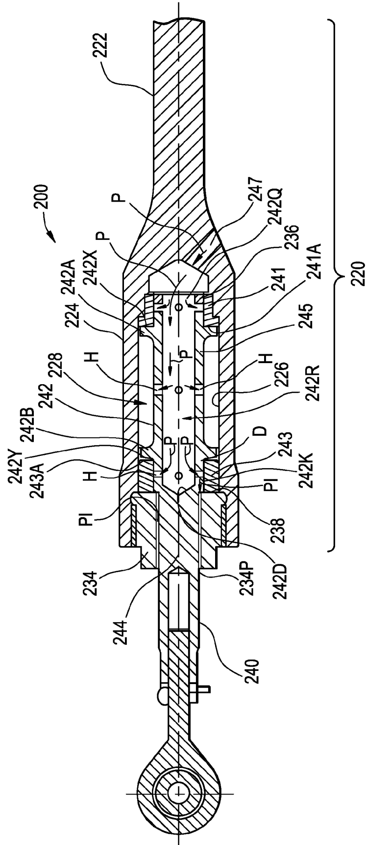
FIG. 12 PRIOR ART
