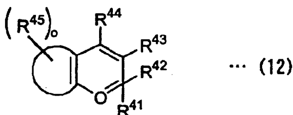
[Chem. 13]
