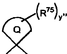
[Chem. 24]
