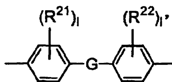
[Chem. 7]
