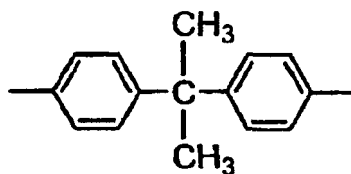
[Chem. 8]
