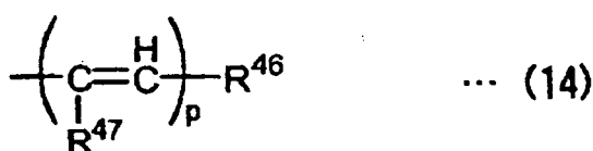
[Chem. 15]
