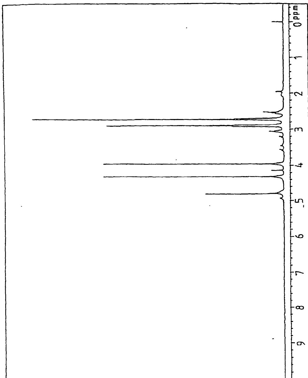
^1\text{H} -NMR SPECTRUM IN PRODUCTION EXAMPLE 4
