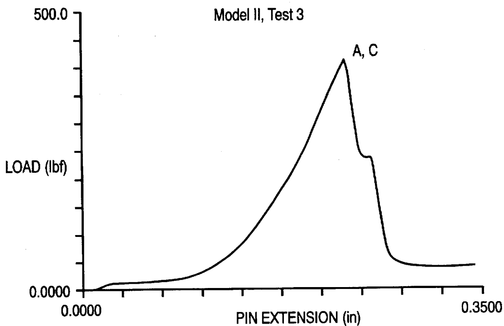
FIG 6c PRIOR ART
