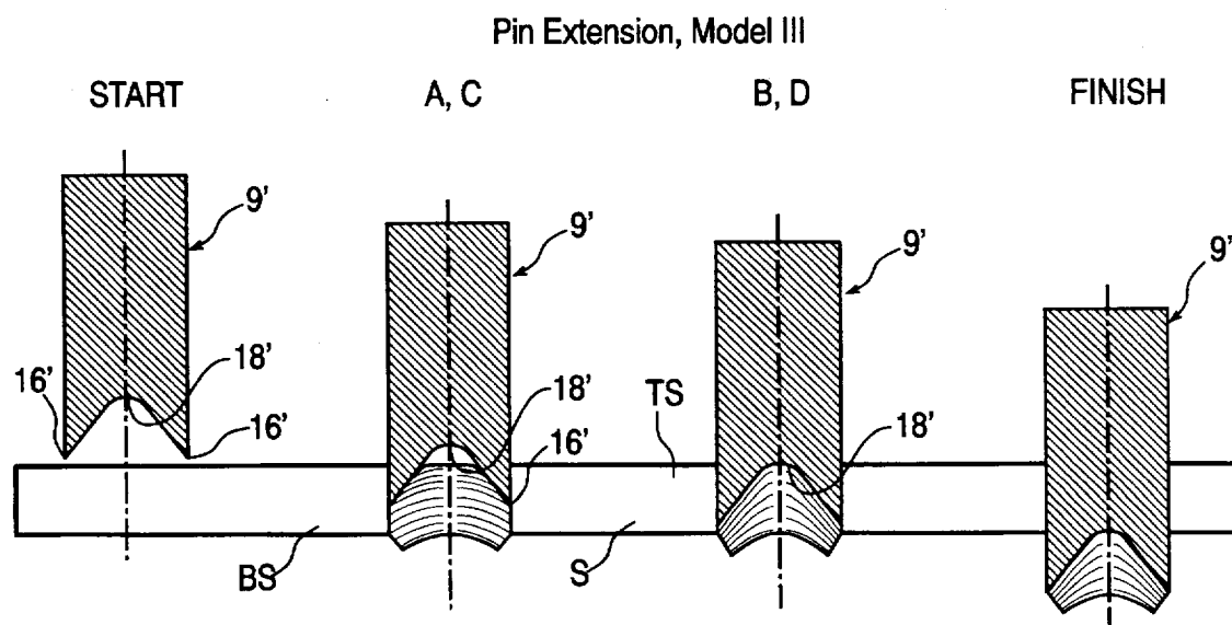
FIG 9 PRIOR ART
