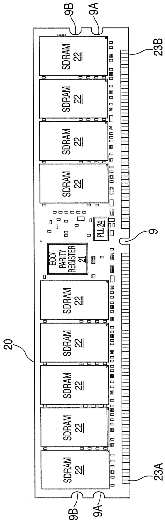
FRONT SIDE OF DIMM - 4 HIGH STACK
