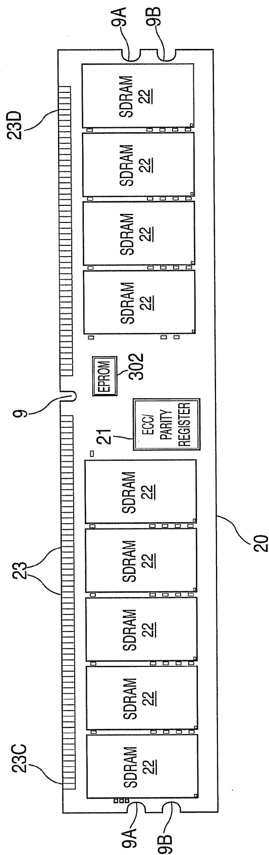
BACK SIDE OF DIMM - 4 HIGH STACK
