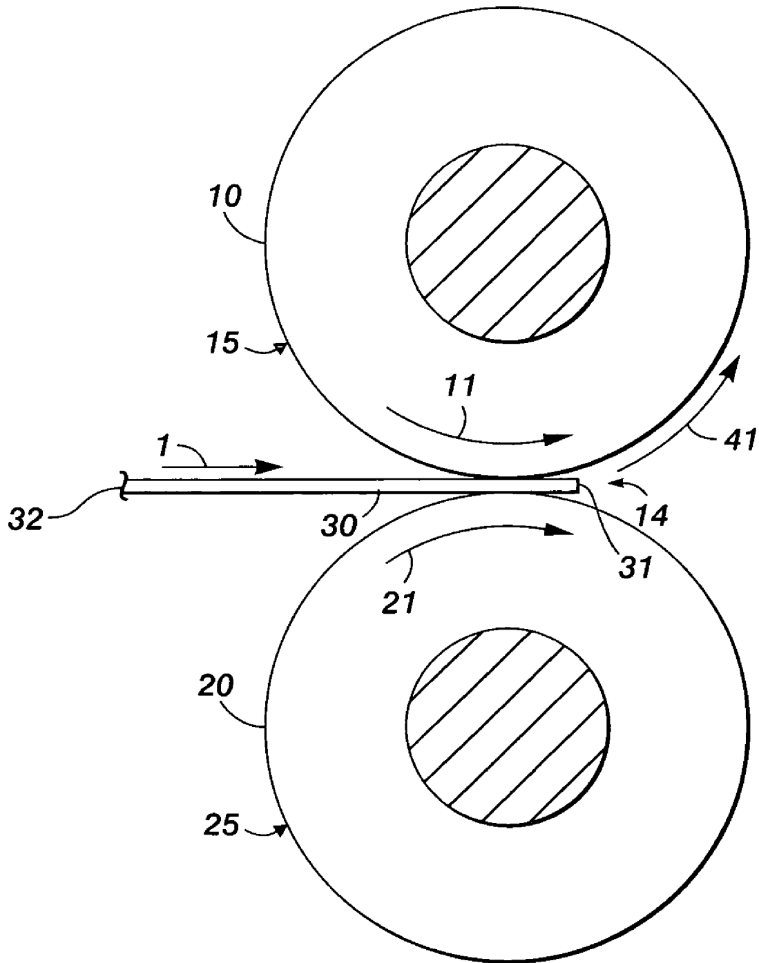
FIG. 1 PRIOR ART
