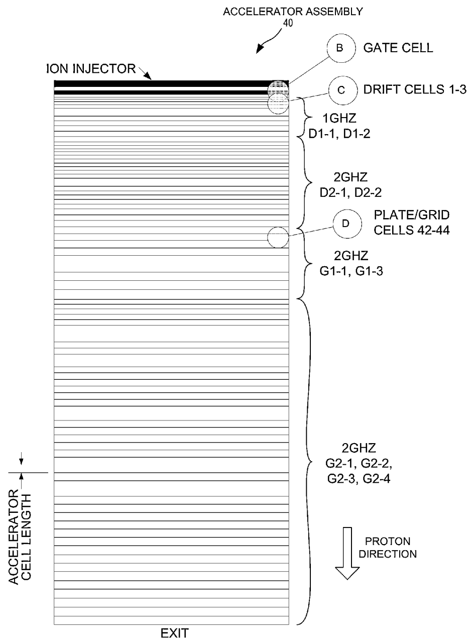
ACCELERATOR CELL LENGTHS
