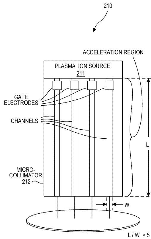
ACCELERATOR HAVING A MULTI- CHANNEL MICRO-COLLIMATOR
