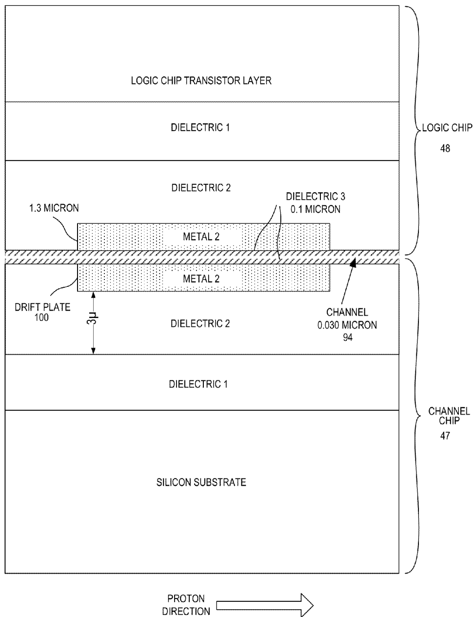
SECTION E-E – DRIFT CELL 2 SIDE VIEW
