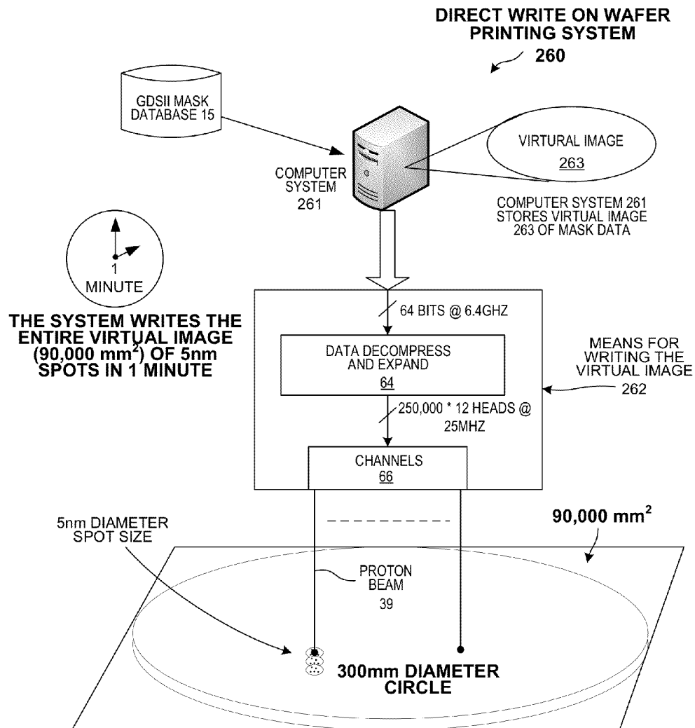
DIRECT WRITE ON WAFER PRINTING SYSTEM
