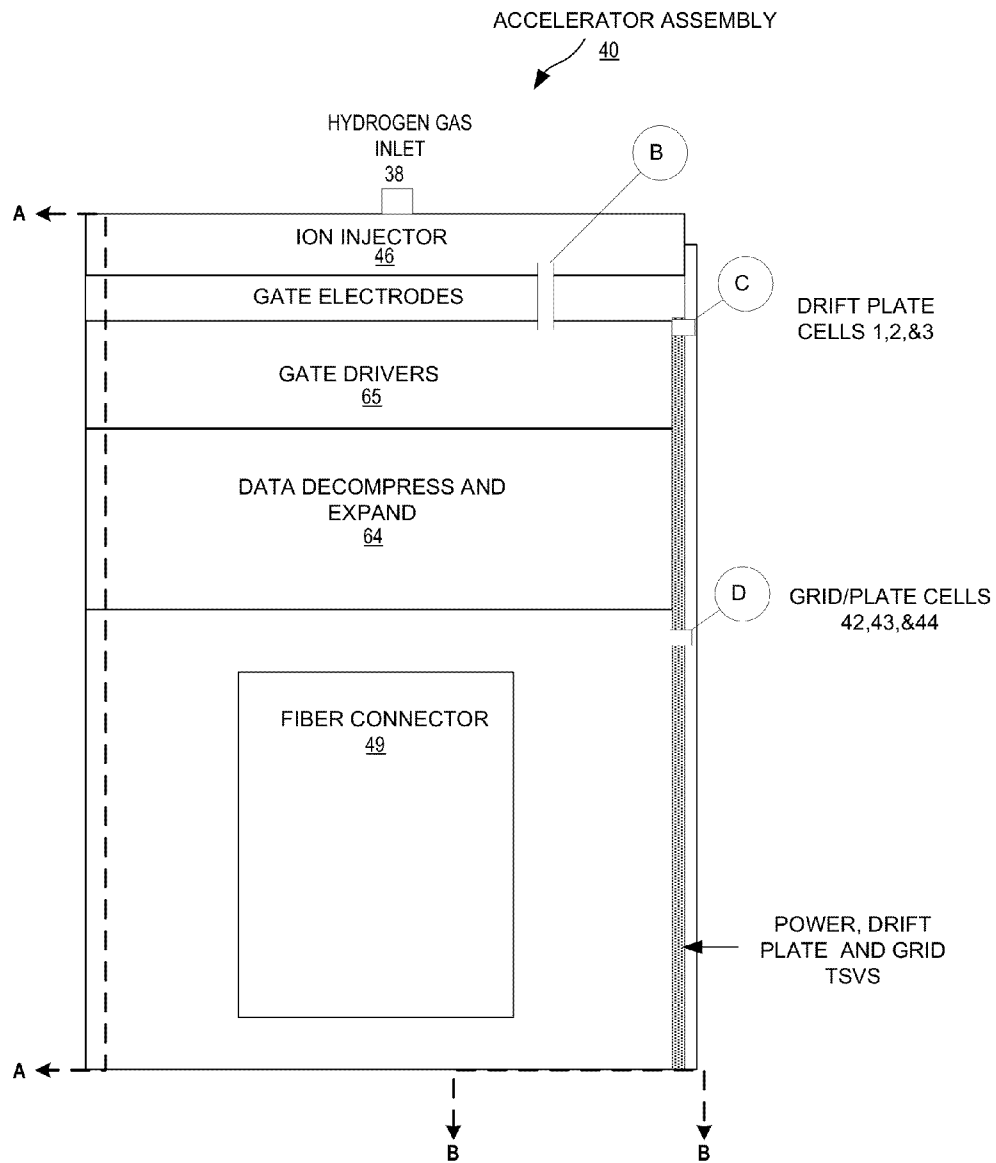
ACCELERATOR ASSEMBLY
