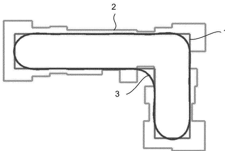
OPTICAL PROXIMITY CORRECTION (Prior Art) FIG. 2
