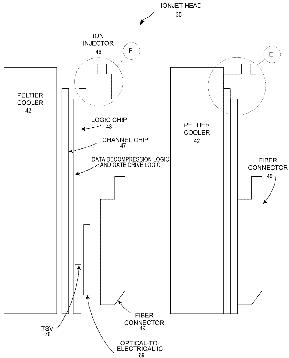
SECTION A-A IONJET HEAD SIDE VIEW
