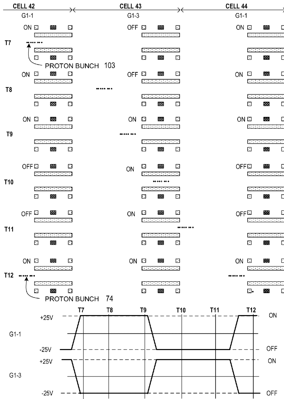
GATE PROTON TIMING SCHEME
