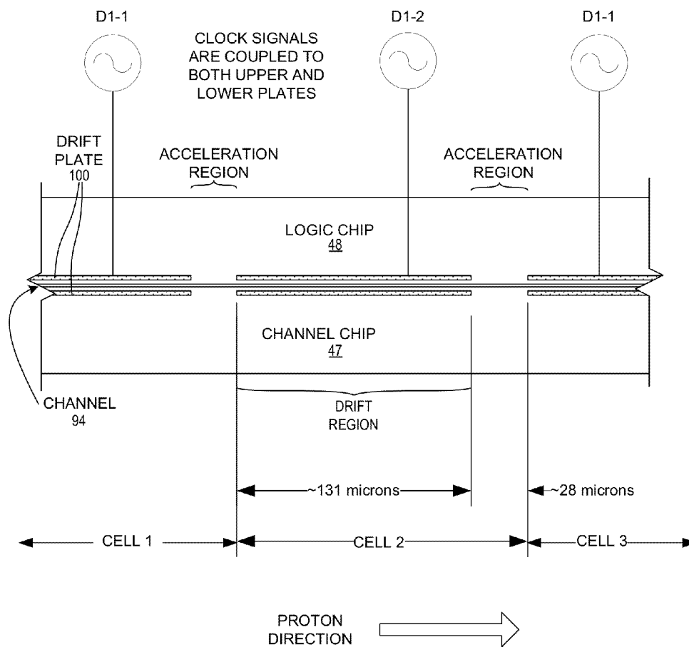
SECTION D-D - DRIFT CELL SIDE VIEW
