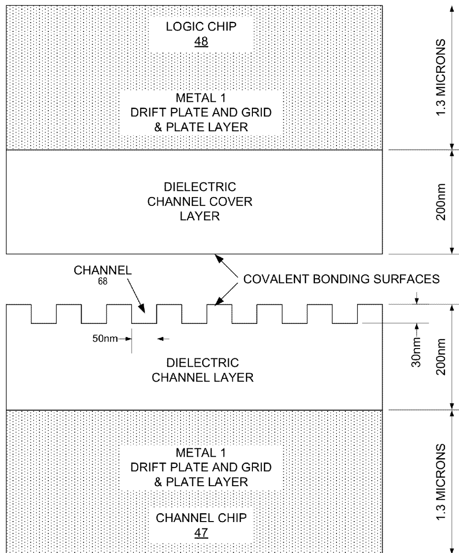
DETAIL H - CHANNEL
