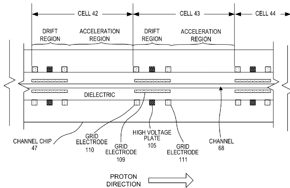
SECTION F-F – PLATE/GRID CELL SIDE VIEW
