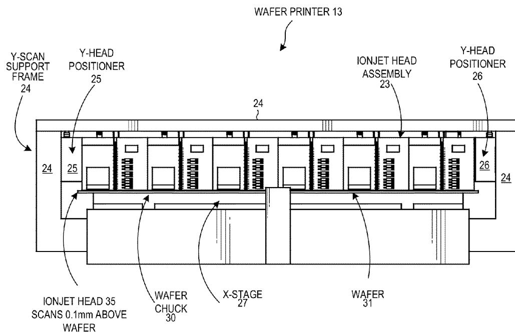
WAFER PRINTER (SIDE VIEW)
