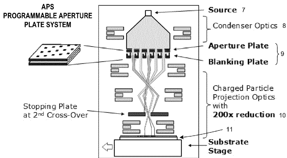
PROTON BEAM STEPPER
