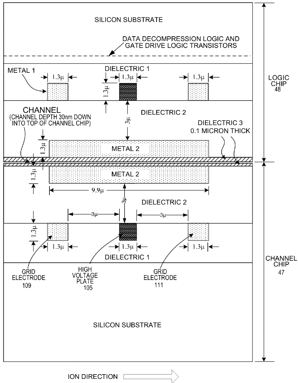
SECTION G-G - PLATE/GRID CELL 43 SIDE VIEW
