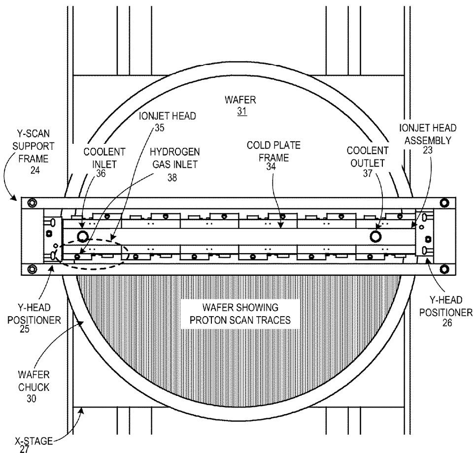
WAFER PRINTER (TOP-DOWN VIEW)
