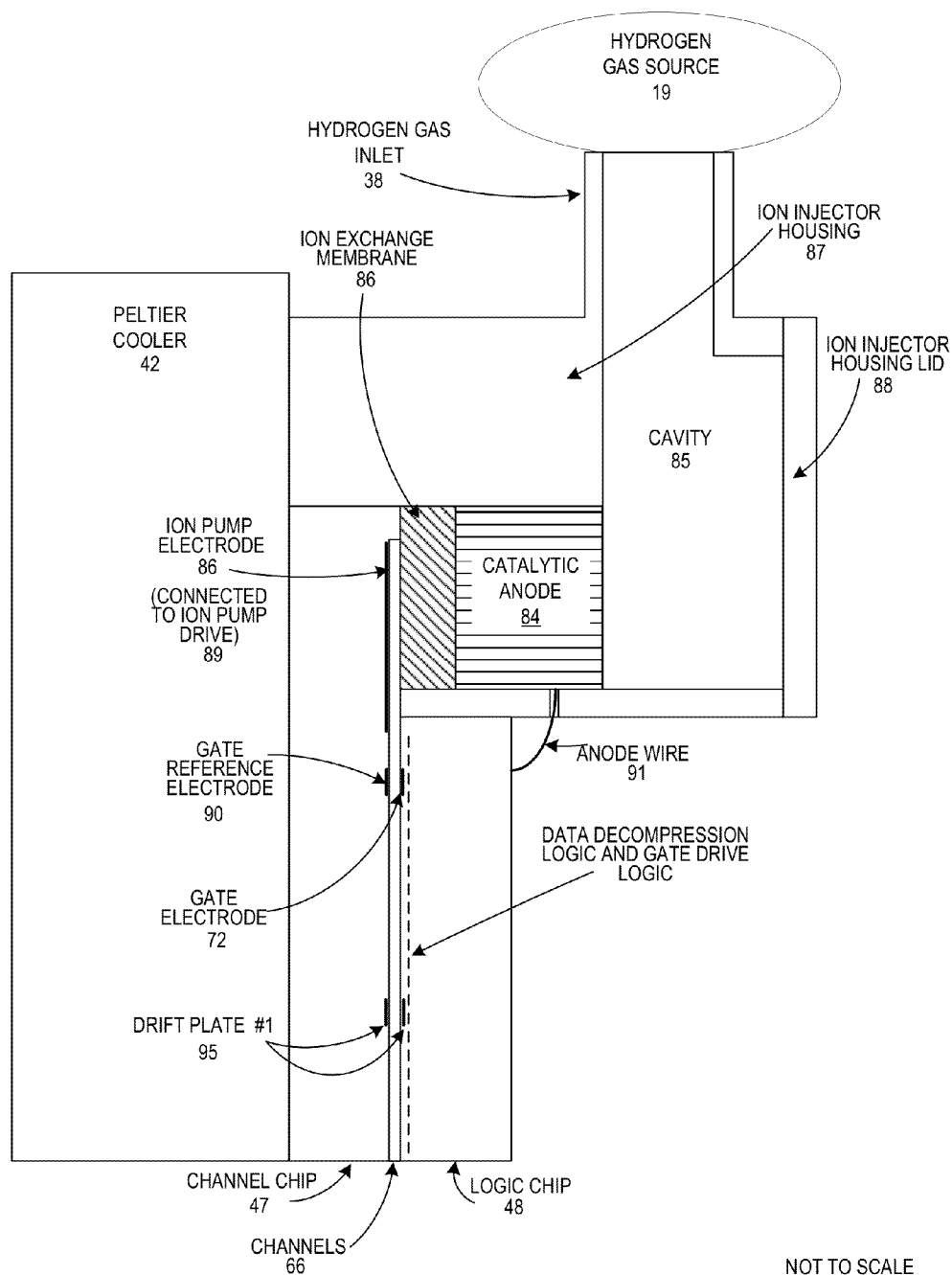
DETAIL E - ION INJECTOR
