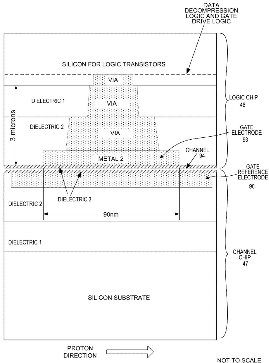
SECTION C-C – GATE CELL SIDE VIEW
