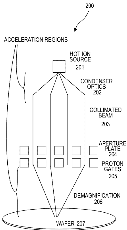
ION SOURCE AND COLLIMATOR (PRIOR ART)
