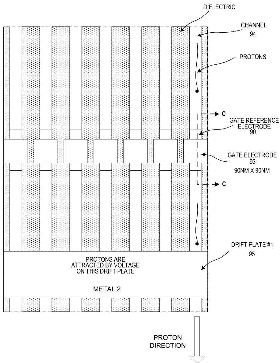
DETAIL B – GATE CELL TOP-DOWN VIEW
