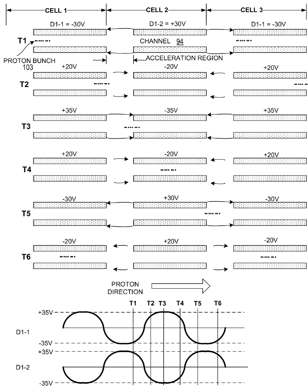
DETAIL E – DRIFT PROTON TIMING SCHEME
