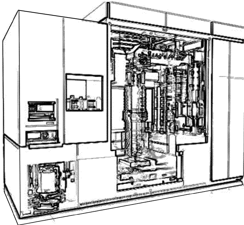
WAFER STEPPER (Prior Art) FIG. 1
