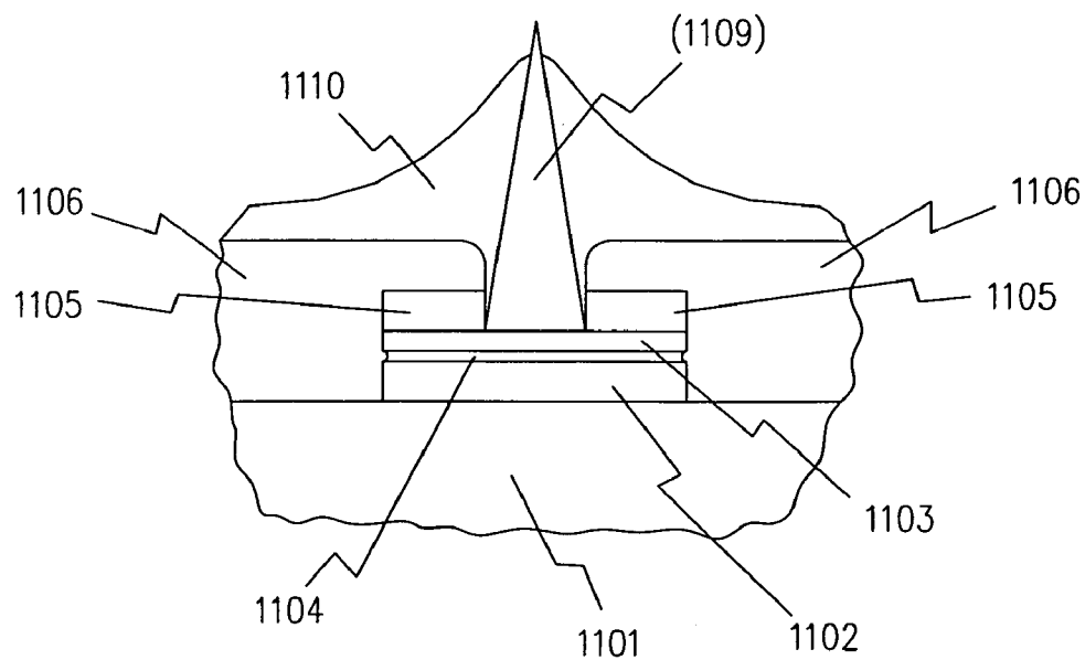
FIGURE 11b ELECTRODES
