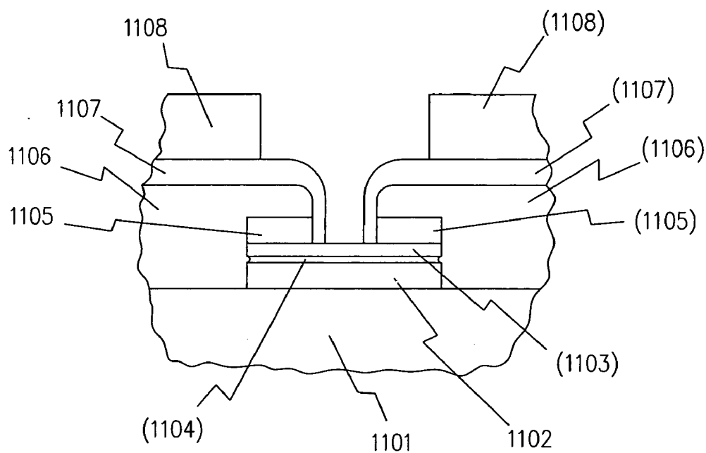
FIGURE 11a ELECTRODES
