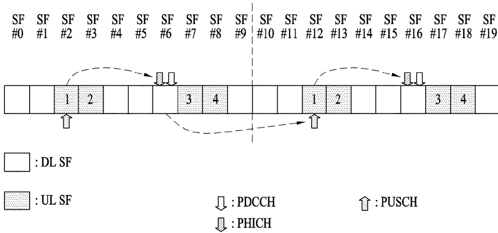
HARQ processes in UL-DL configuration #1
