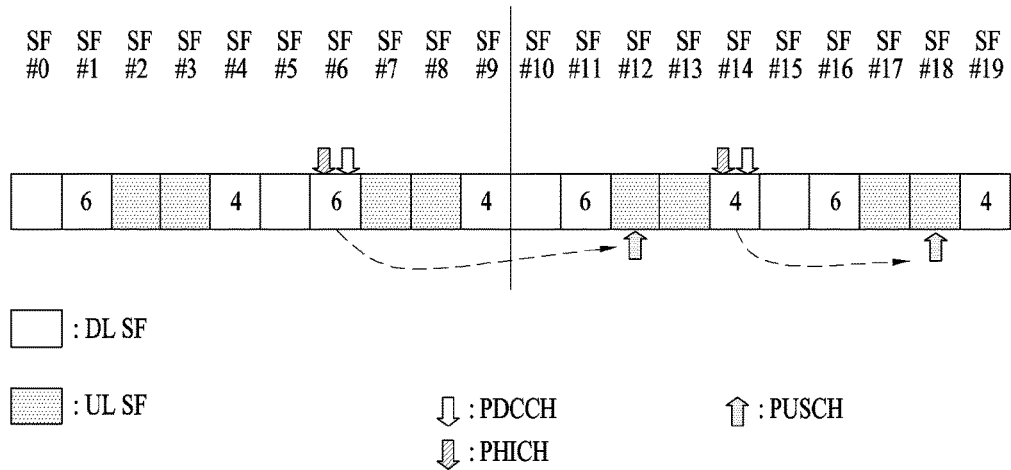
PHICH/UL grant-PUSCH timing (UL-DL configuration #1)
