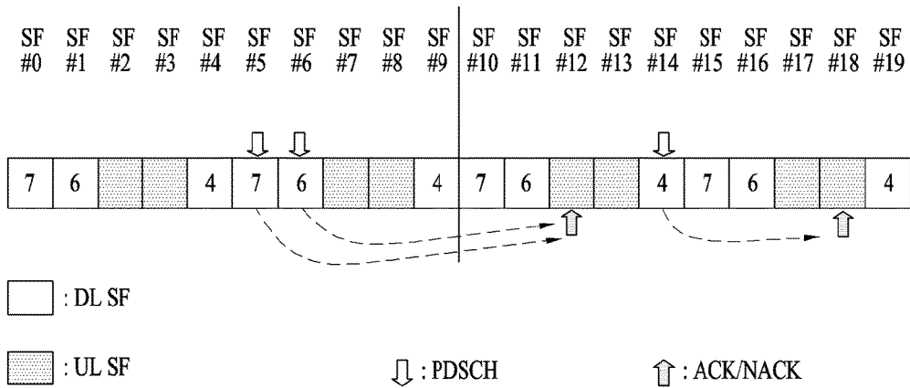
PDSCH-ACK/NACK timing (UL-DL configuration #1)
