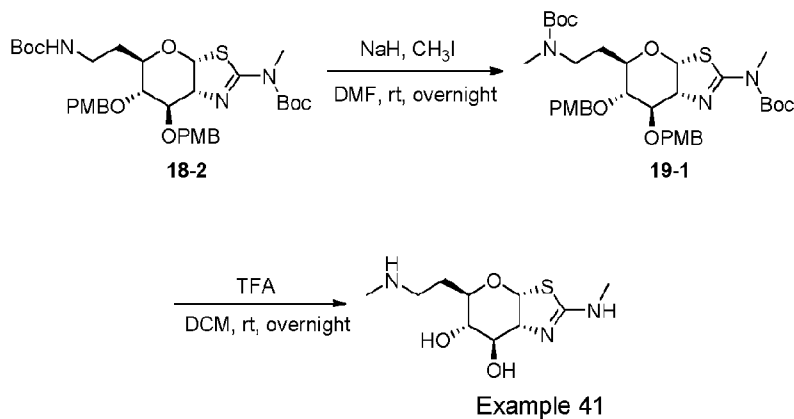
Scheme 19
