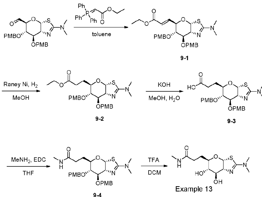
Scheme 9
