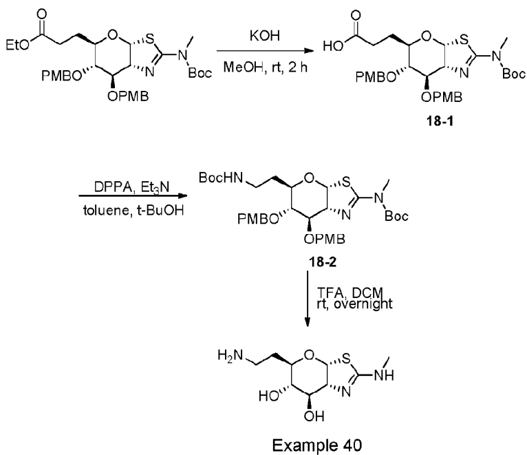
Scheme 18
