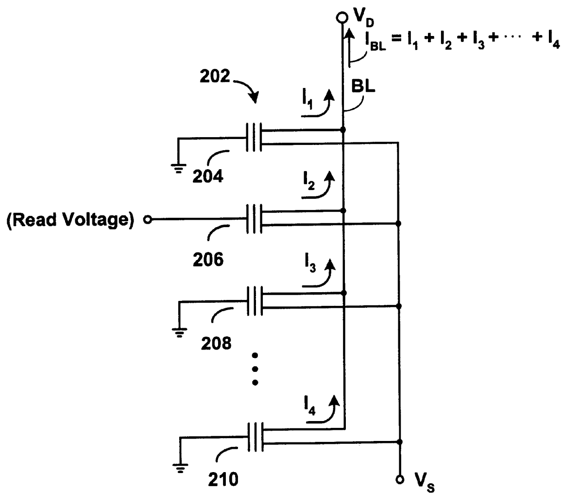
FIGURE 2C (PRIOR ART)
