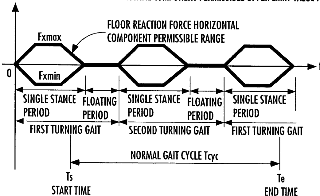
FLOOR REACTION FORCE HORIZONTAL COMPONENT PERMISSIBLE LOWER LIMIT VALUE F_{xmin} AND FLOOR REACTION FORCE HORIZONTAL COMPONENT PERMISSIBLE UPPER LIMIT VALUE F_{xmax}
