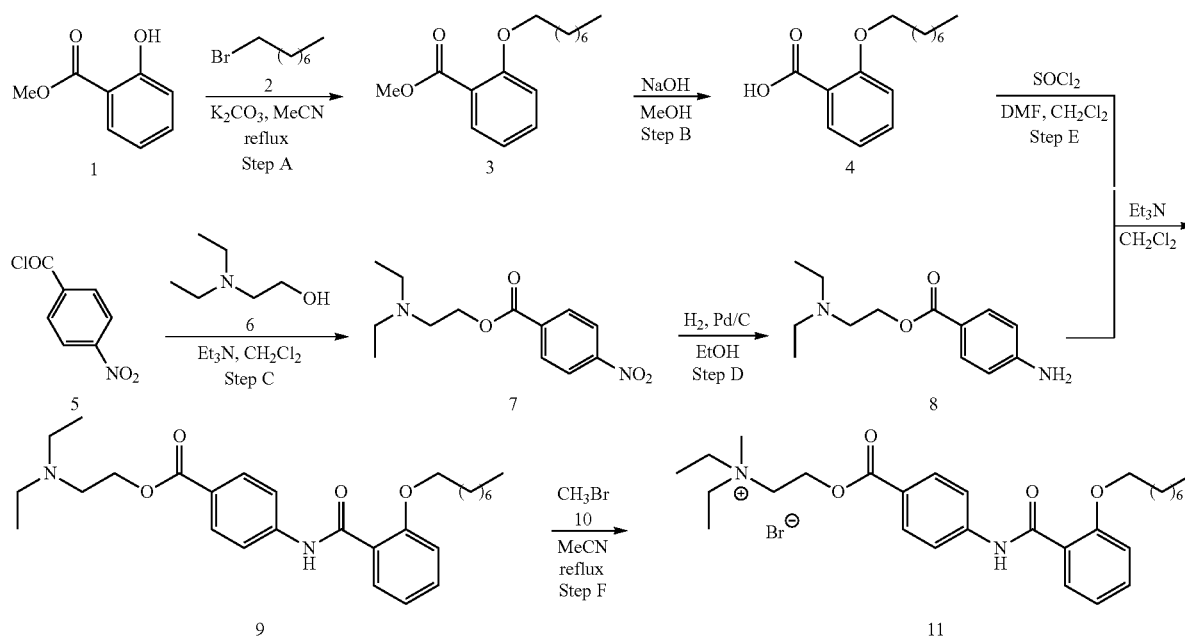
Scheme 2. Representative example for the synthesis of otilonium bromide
