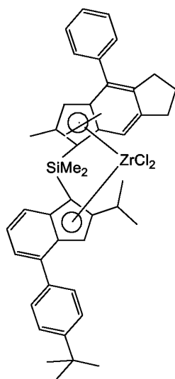
Pseudo rac Dimethylsilanediyl-(6-methyl-4-phenyl-1,2,3,5-tetrahydro-s-indacen-7-yl)-(2-isopropyl-4-(4'-tert-butylphenyl)-1-indenyl)-zirconium dichloride (C-2)
