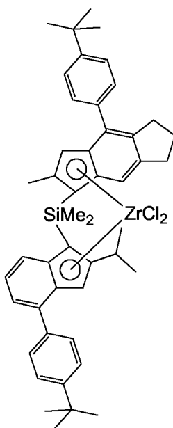
Pseudo rac Dimethylsilanediyl-(6-methyl-4-phenyl-1,2,3,5-tetrahydro-s-indacen-7-yl)-(2-isopropyl-4-(4'-tert-butylphenyl)-1-indenyl)-zirconium dichloride (C-2)
