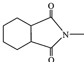
1,2-cyclohexanedicarboximido
