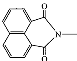
1,8-naphthalimido
