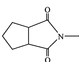
1,2-cyclopentanedicarboximido
