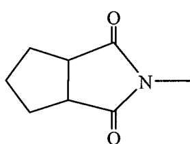
1,2-cyclopentanedicarboximido
