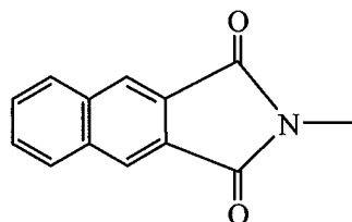
2,3-naphthalimido
