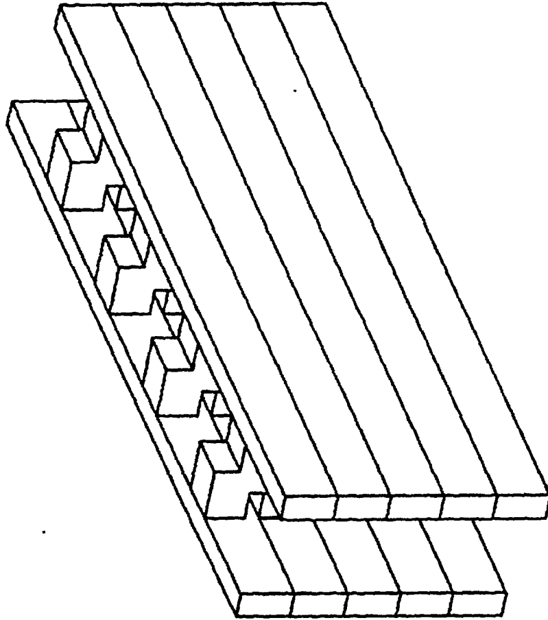
RAIL WITH NO ADHESION EXCEPT FOR THE ATTACHING STRUCTURE
