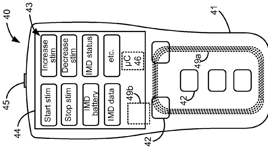
Figure 3 (prior art)
