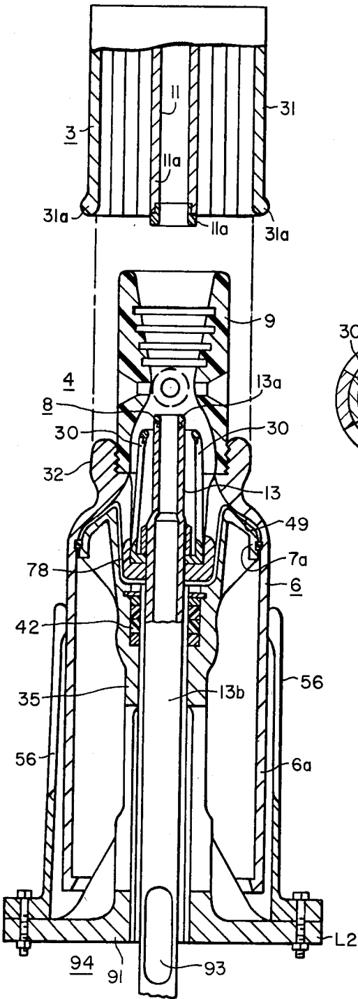
OPEN POSITION
