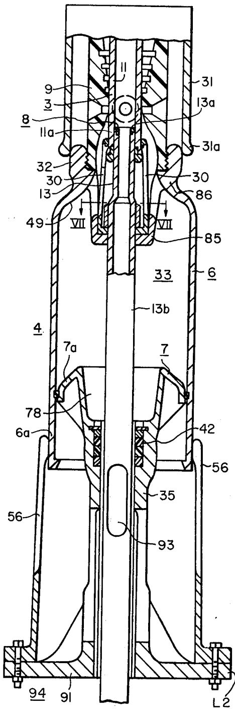
CLOSED POSITION
