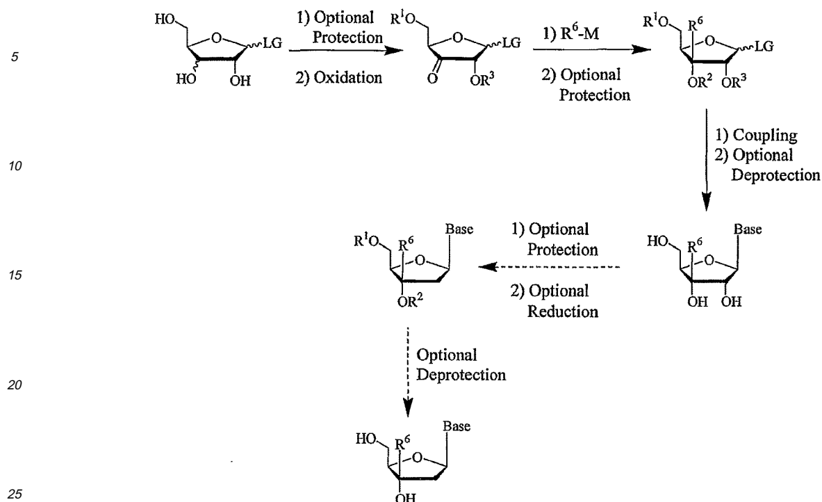
Scheme 5
