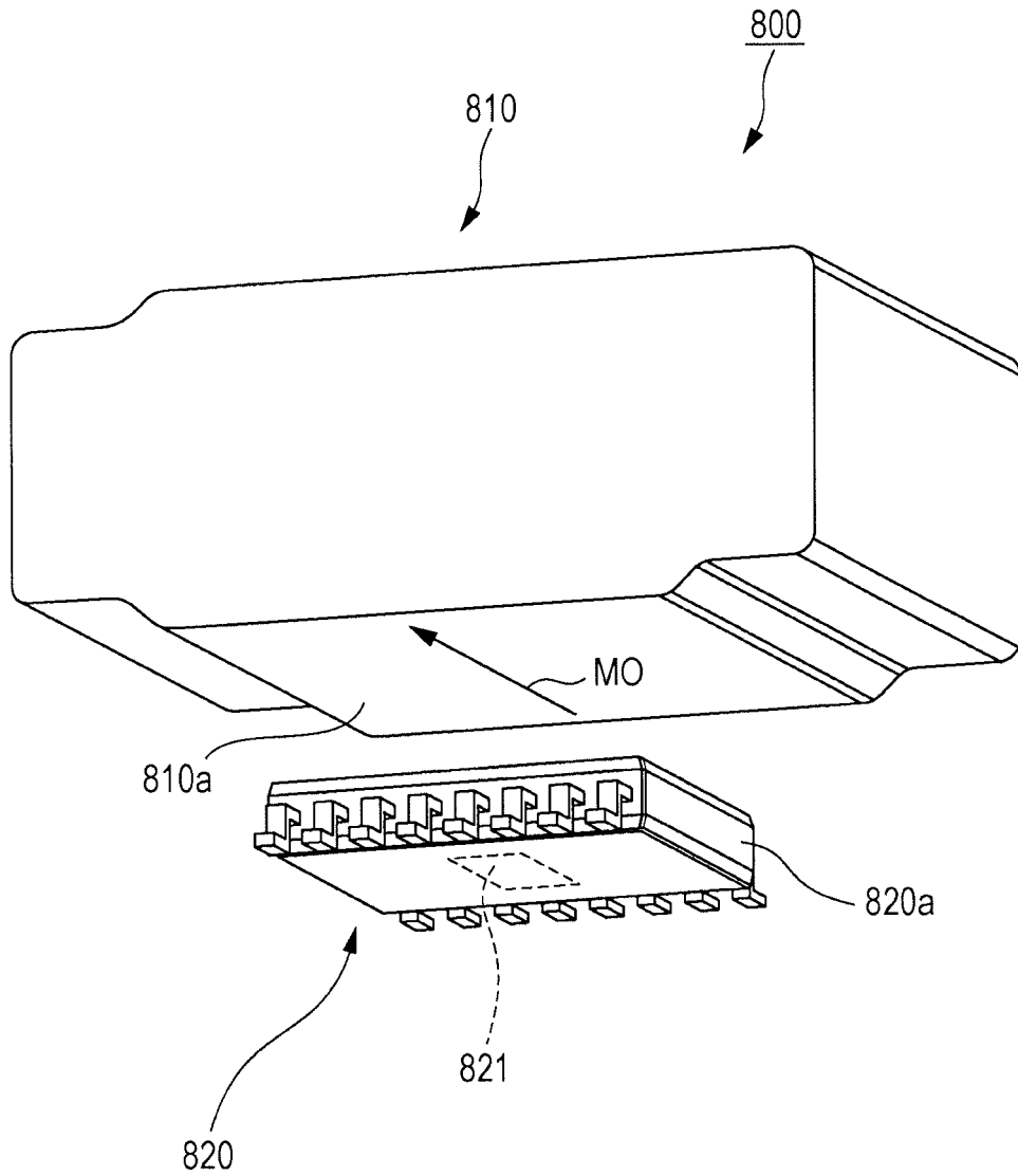
FIG. 7 PRIOR ART
