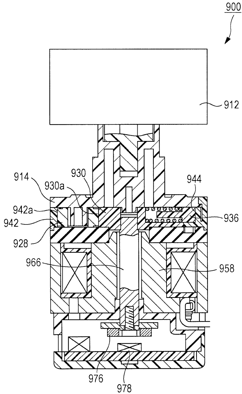
FIG. 6 PRIOR ART
