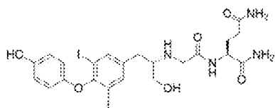
T2AA-Gln
