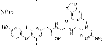
T2AA-NPip-NLys
