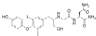
T2AA-Asn
