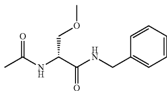
Structure of Lacosamide
