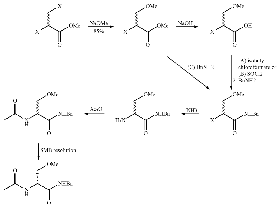
Scheme 5: Method for production of Lacosamide in WO2010052011
