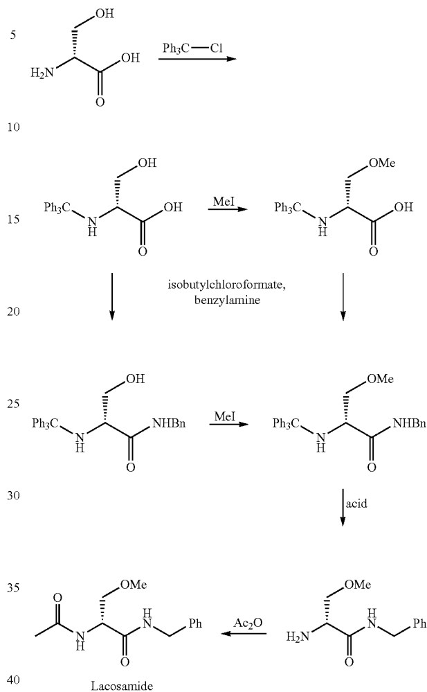
Scheme 4: Method for production of Lacosamide in EP2067765 A1
