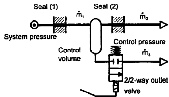
Figure 7: Equivalent circuit diagram for a control system with two seals and a 2/2-way outlet valve
