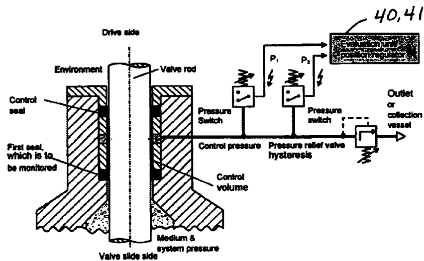
Figure 3: Monitoring of a seal by observing the control pressure, venting from time to time via a pressure relief valve with hysteresis
