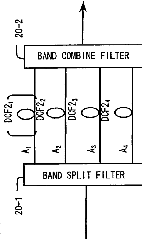
FIG. 25B CASE WHERE ONLY DISPERSION COMPENSATORS FOR MAKING ADJUSTMENT FOR BANDS ARE USED
