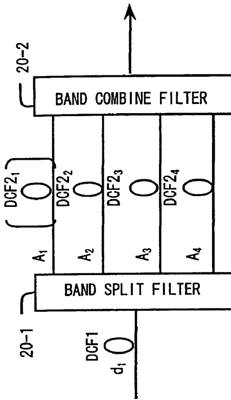
FIG. 25B CASE WHERE ONLY DISPERSION COMPENSATORS FOR MAKING ADJUSTMENT FOR BANDS ARE USED
