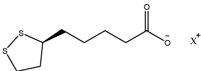
Formula Ib
