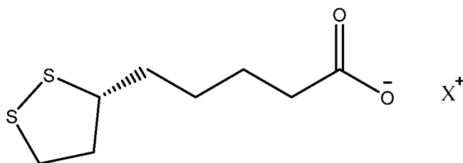
Formula Ia
