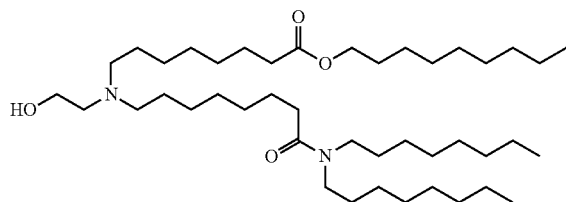
Chemical Formula: C 43 H 86 N 2 O 4 Molecular Weight: 695.17
