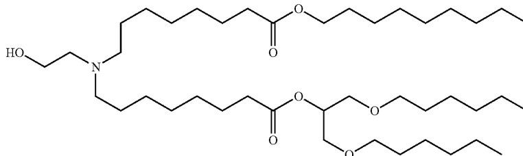
1,3-Bis(hexyloxy)propan-2-yl 8-((2-hydroxyethyl)(8-(nonyloxy)-8-oxooctyl)amino)octanoate
