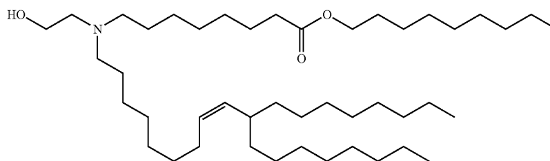
Nonyl (Z)-8-((2-hydroxyethyl)(10-octyloctadec-8-en-1-yl)amino)octanoate
