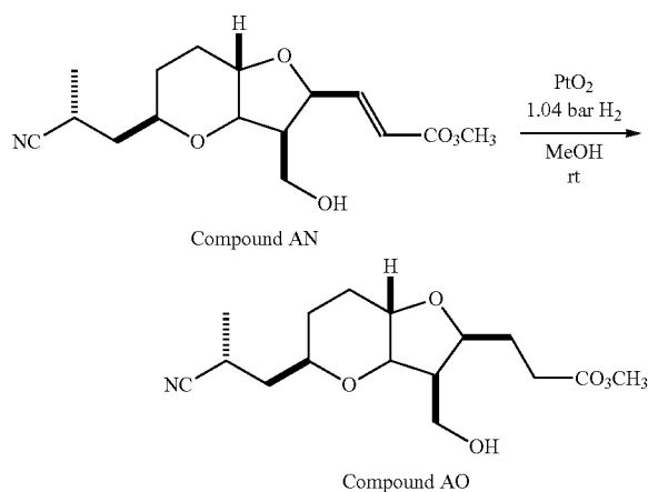
Scheme 19
