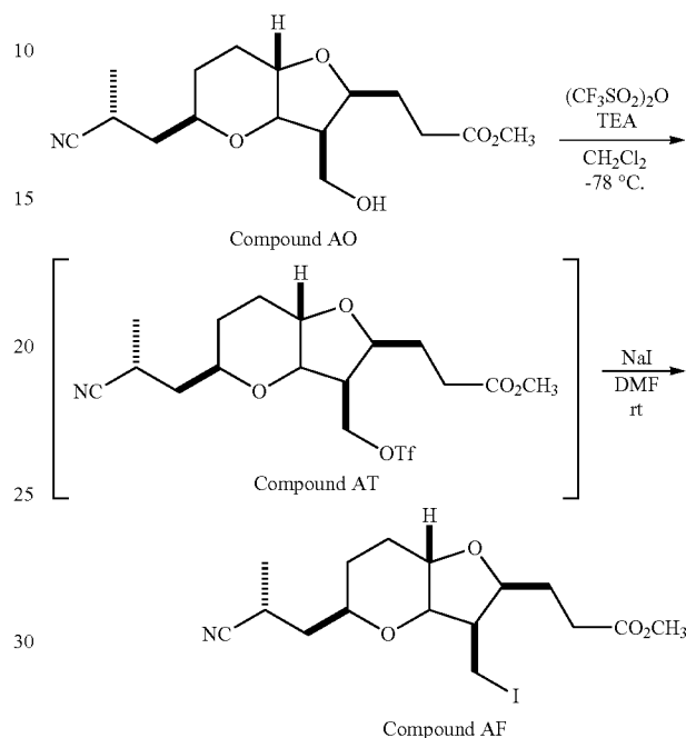
Scheme 20
