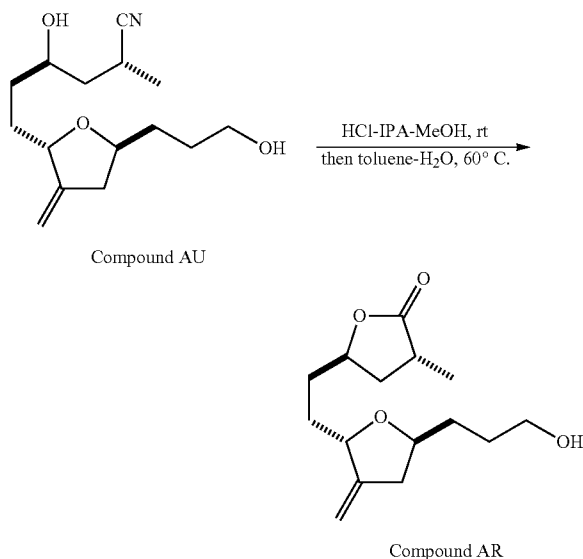
Scheme 23
