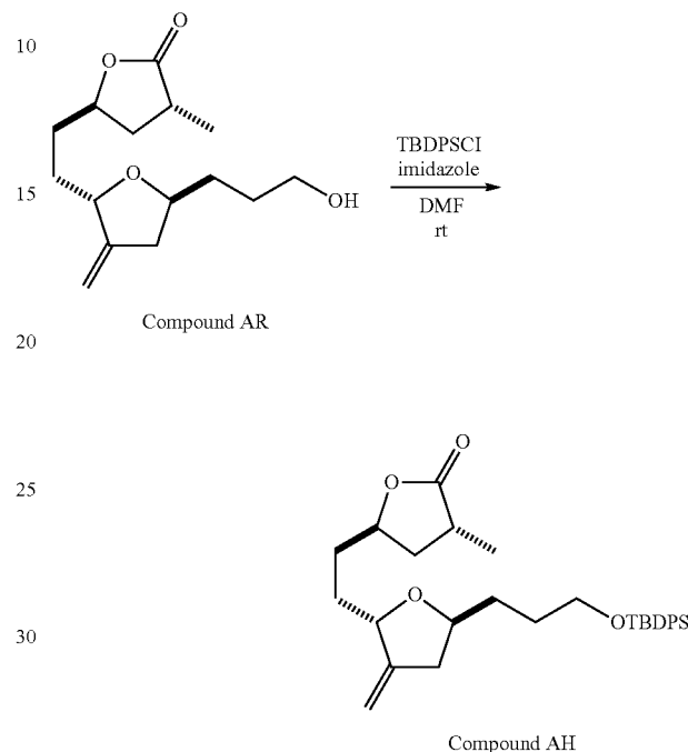
Scheme 24
