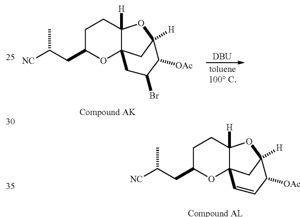
Scheme 16
