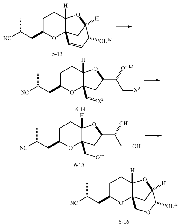
Scheme 6
