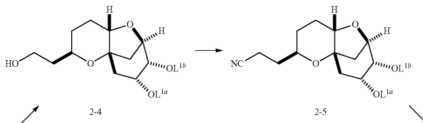
Scheme 2
