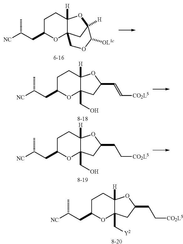
Scheme 8
