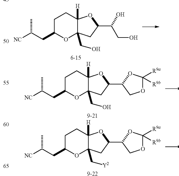
Scheme 9
