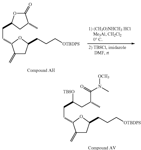
Scheme 25
