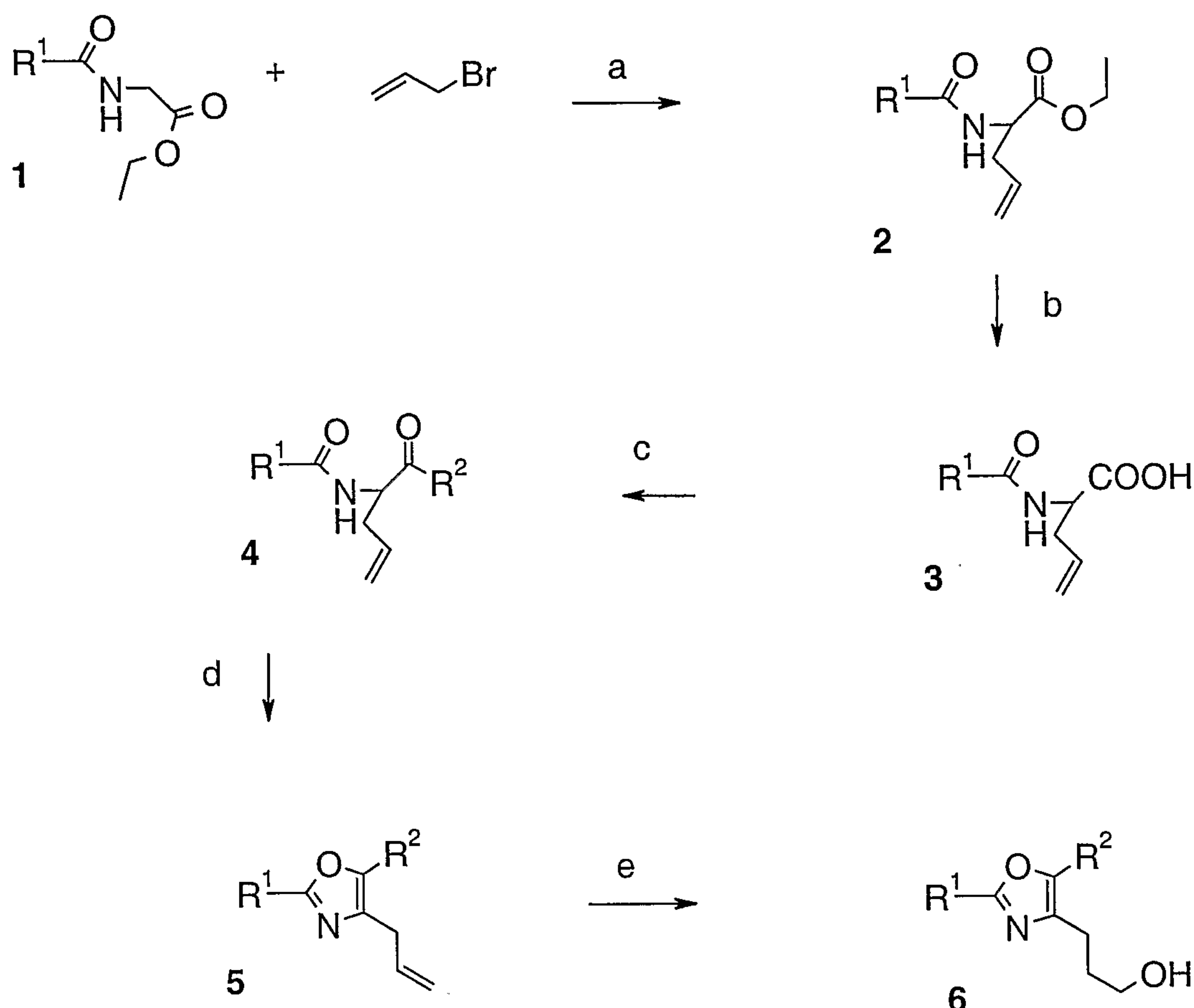
Scheme 7
