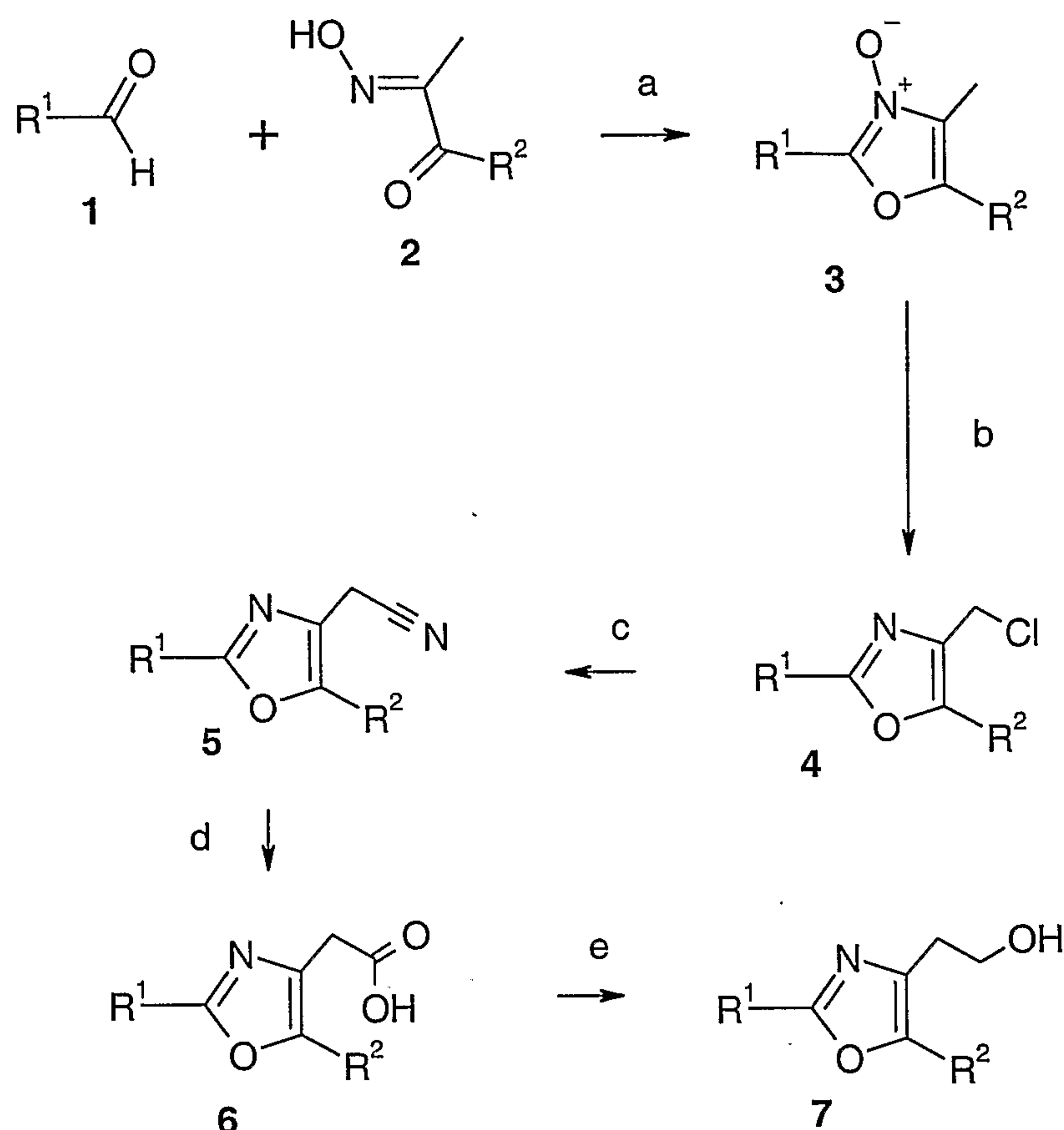
Scheme 6
