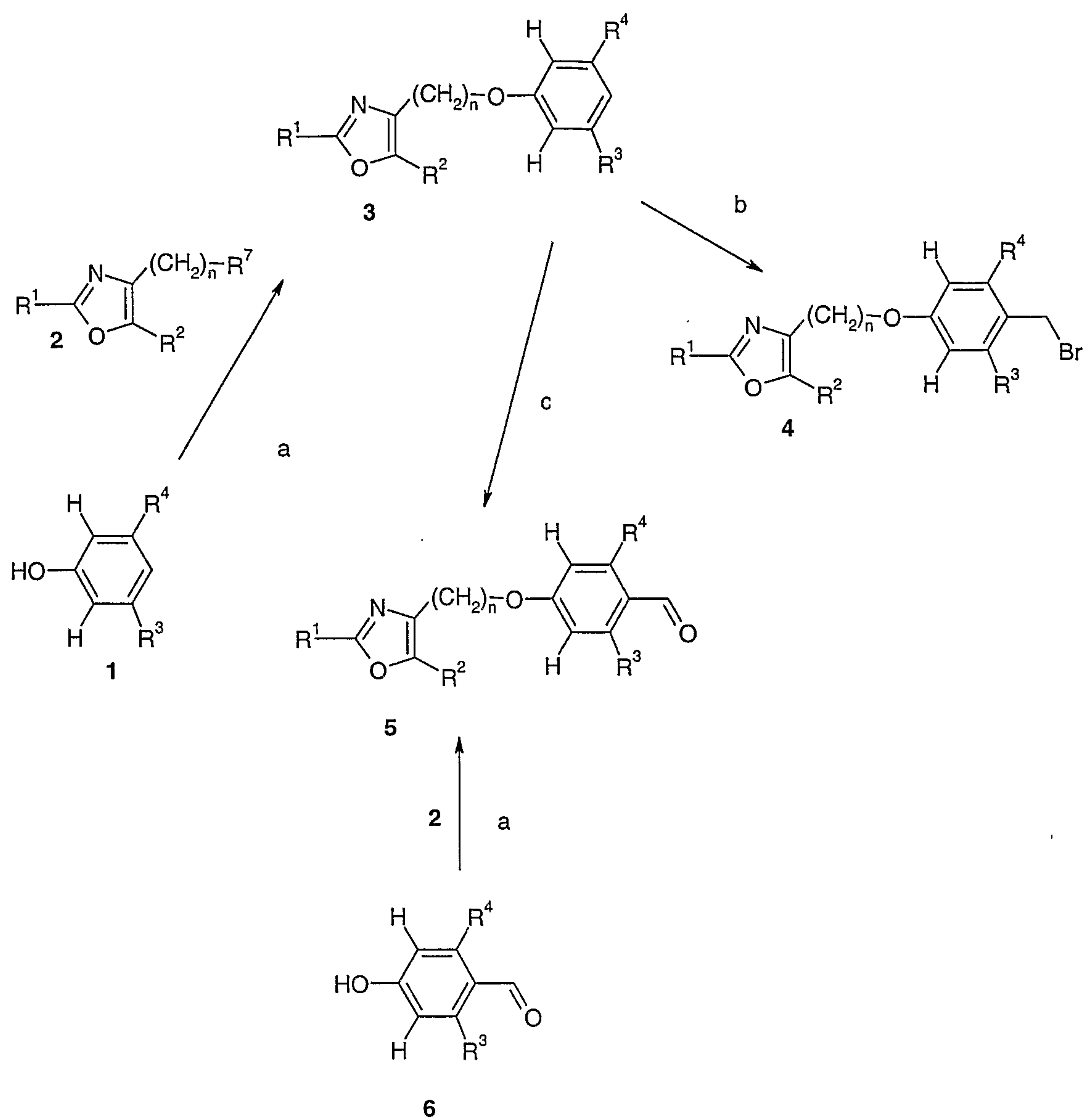
Scheme 4, Part I
