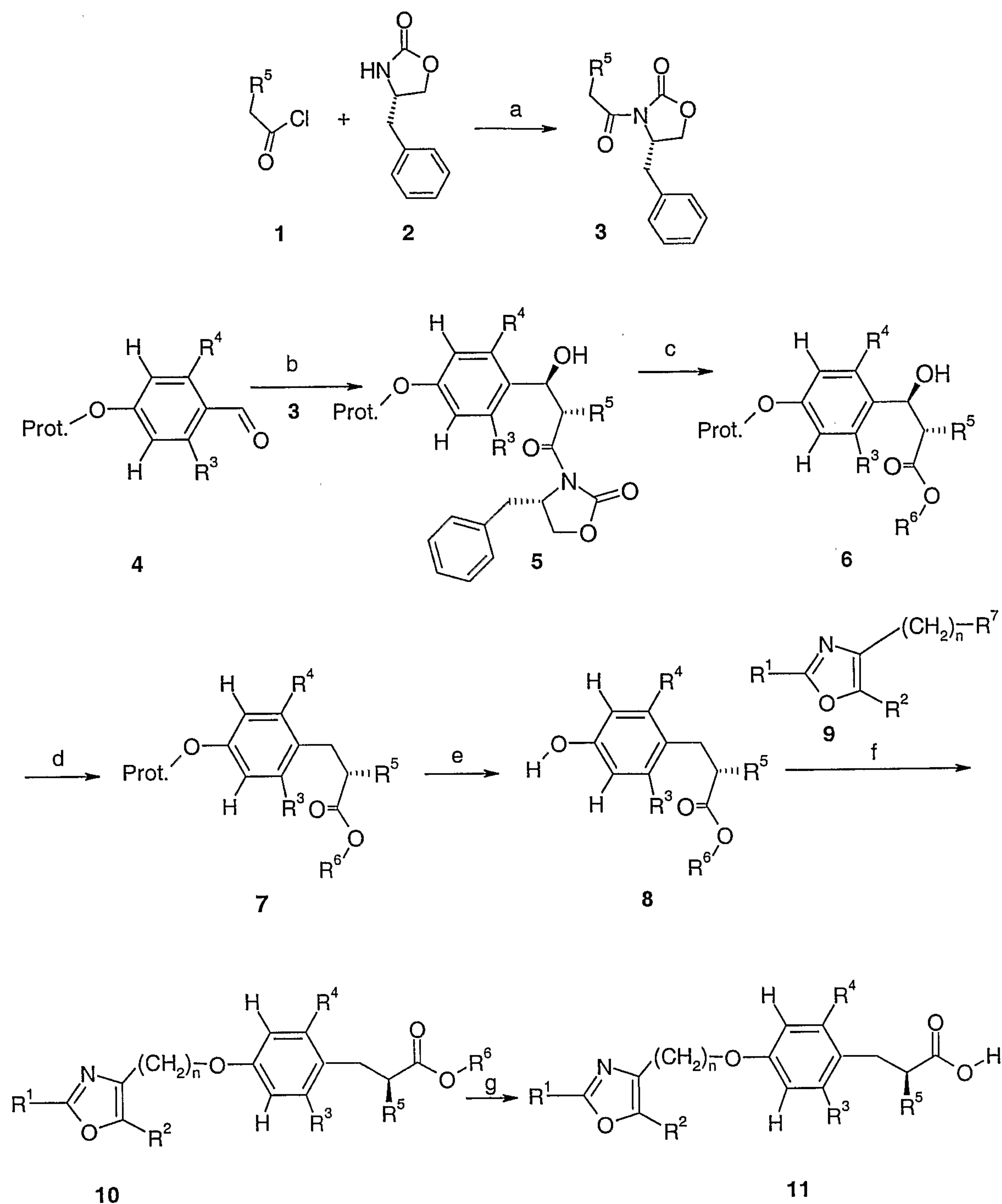
Scheme 1
