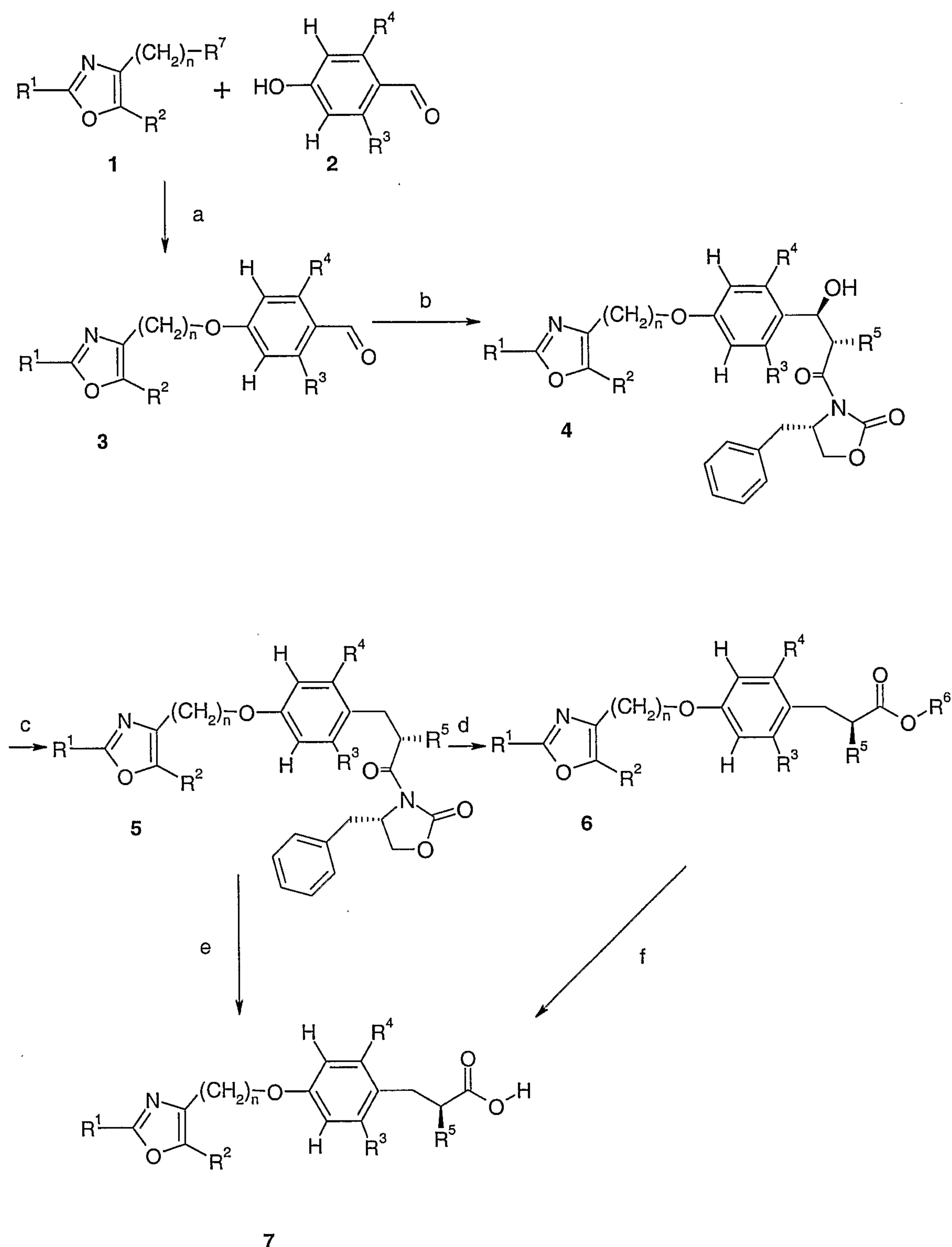
Scheme 3
