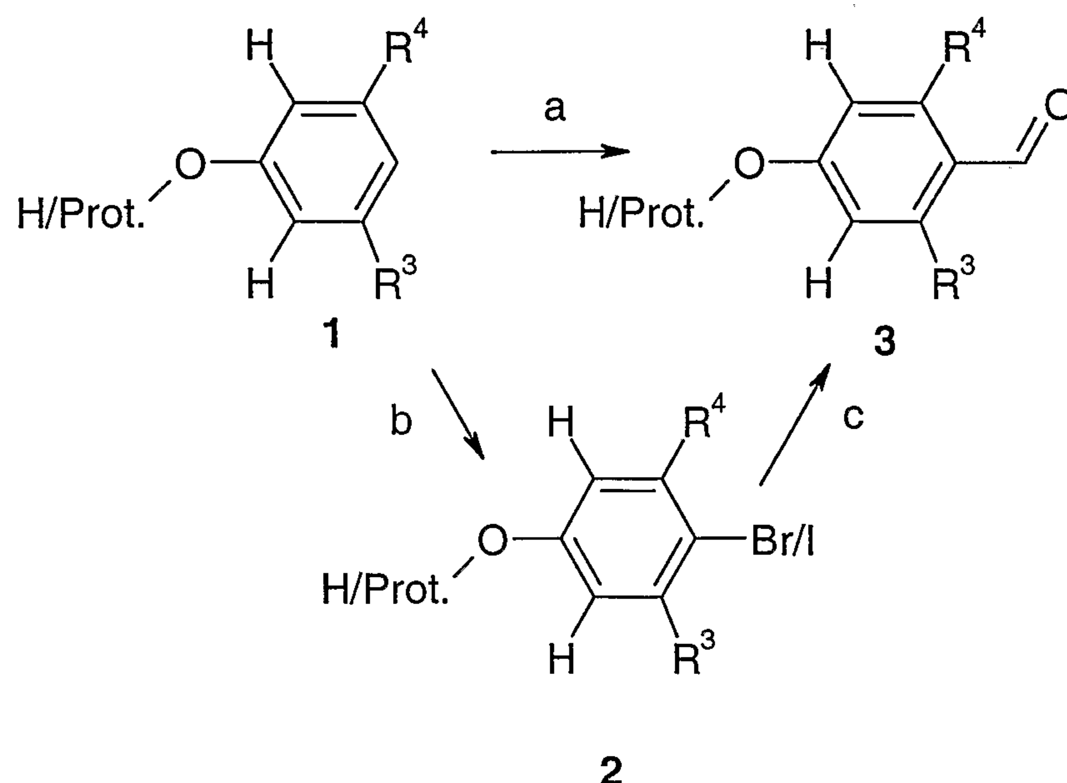
Scheme 5
