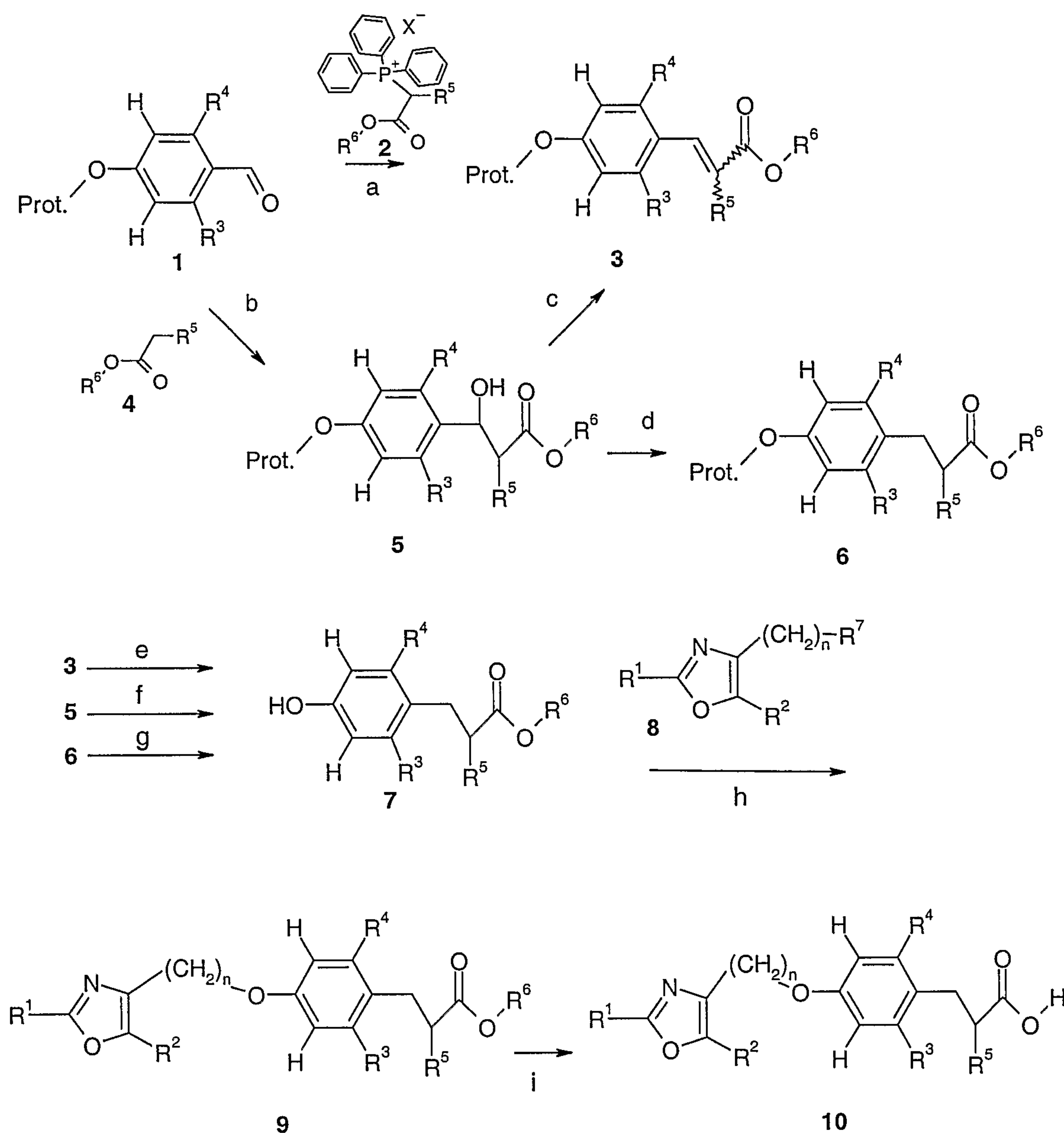
Scheme 2
