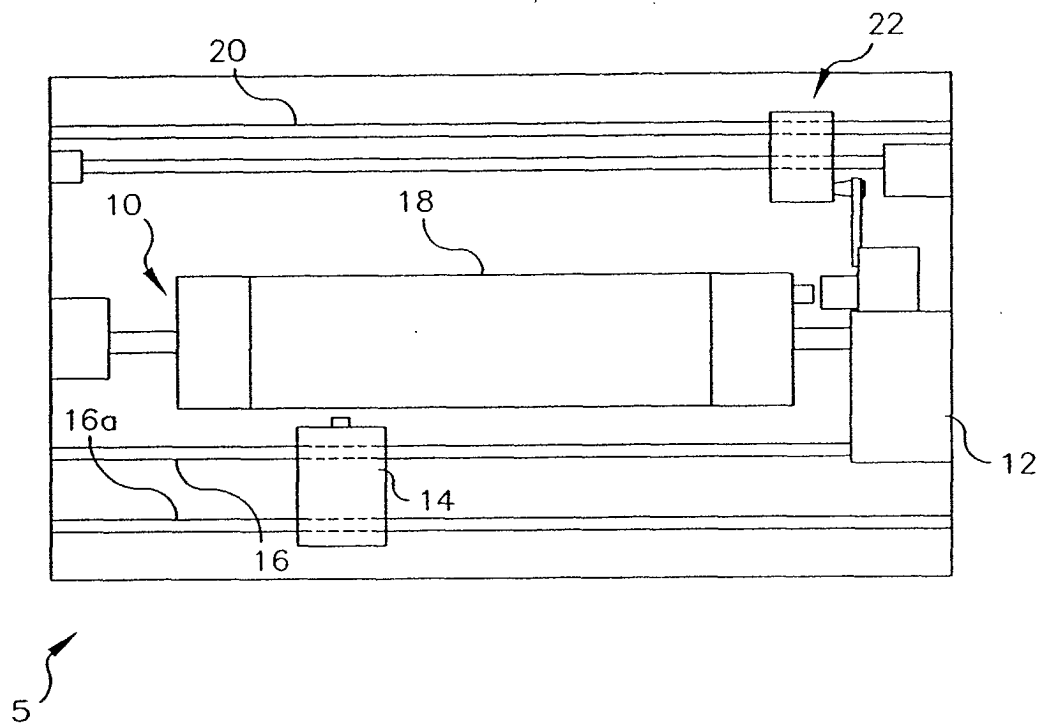
FIG. 1 (PRIOR ART)
