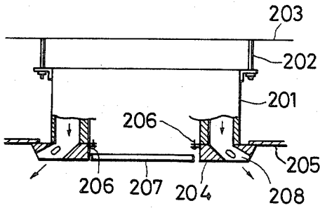
FIG. 5 PRIOR ART
