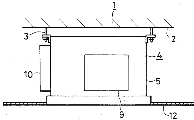
FIG. 3 PRIOR ART
