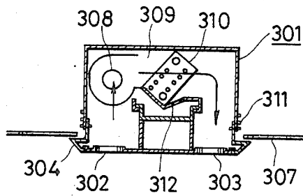
FIG. 7 PRIOR ART
