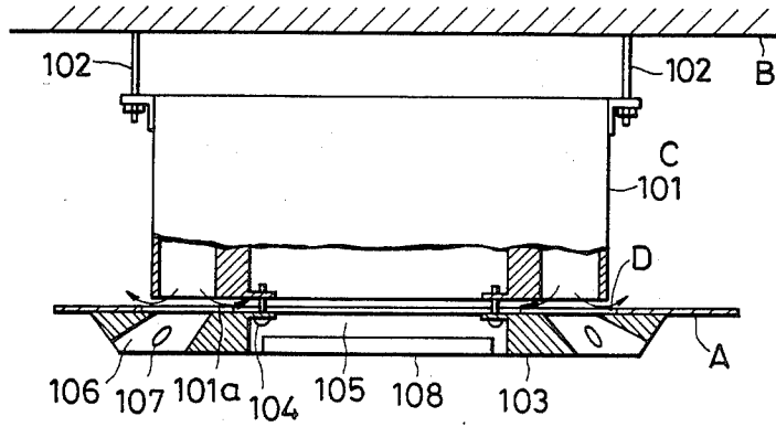
FIG. 4 PRIOR ART
