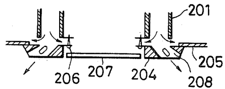
FIG. 6 PRIOR ART
