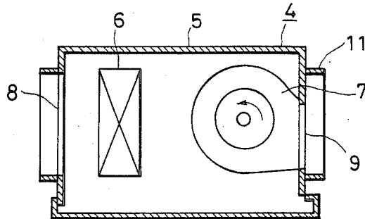
FIG. 1 PRIOR ART
