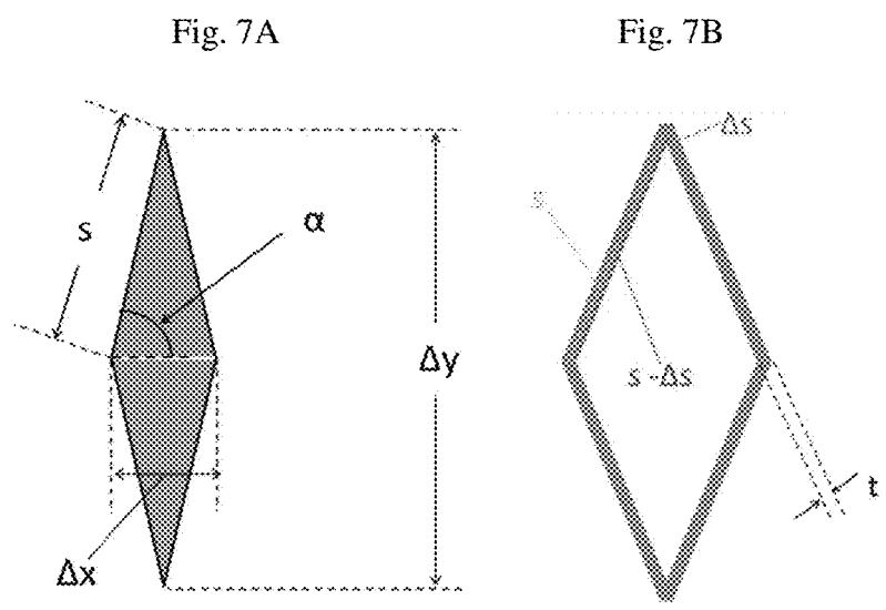
Figure 7: Fluid pathway geometry definitions
