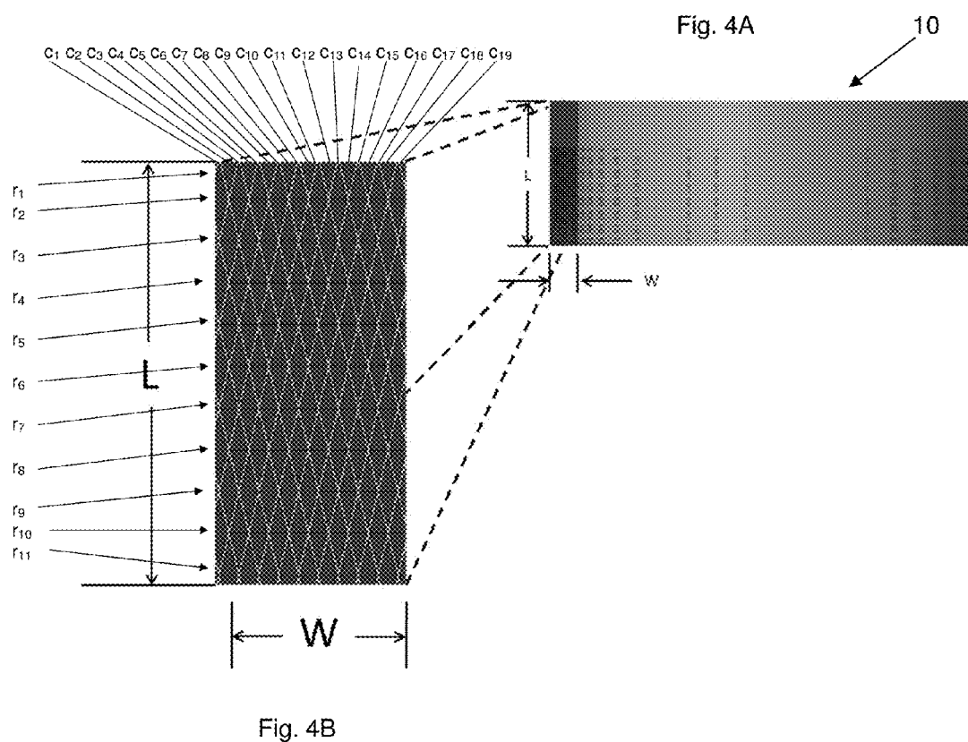
Figure 4: Swept cross sectional view of the 3d spiral heat exchanger showing fluid pathways created in this embodiment.
