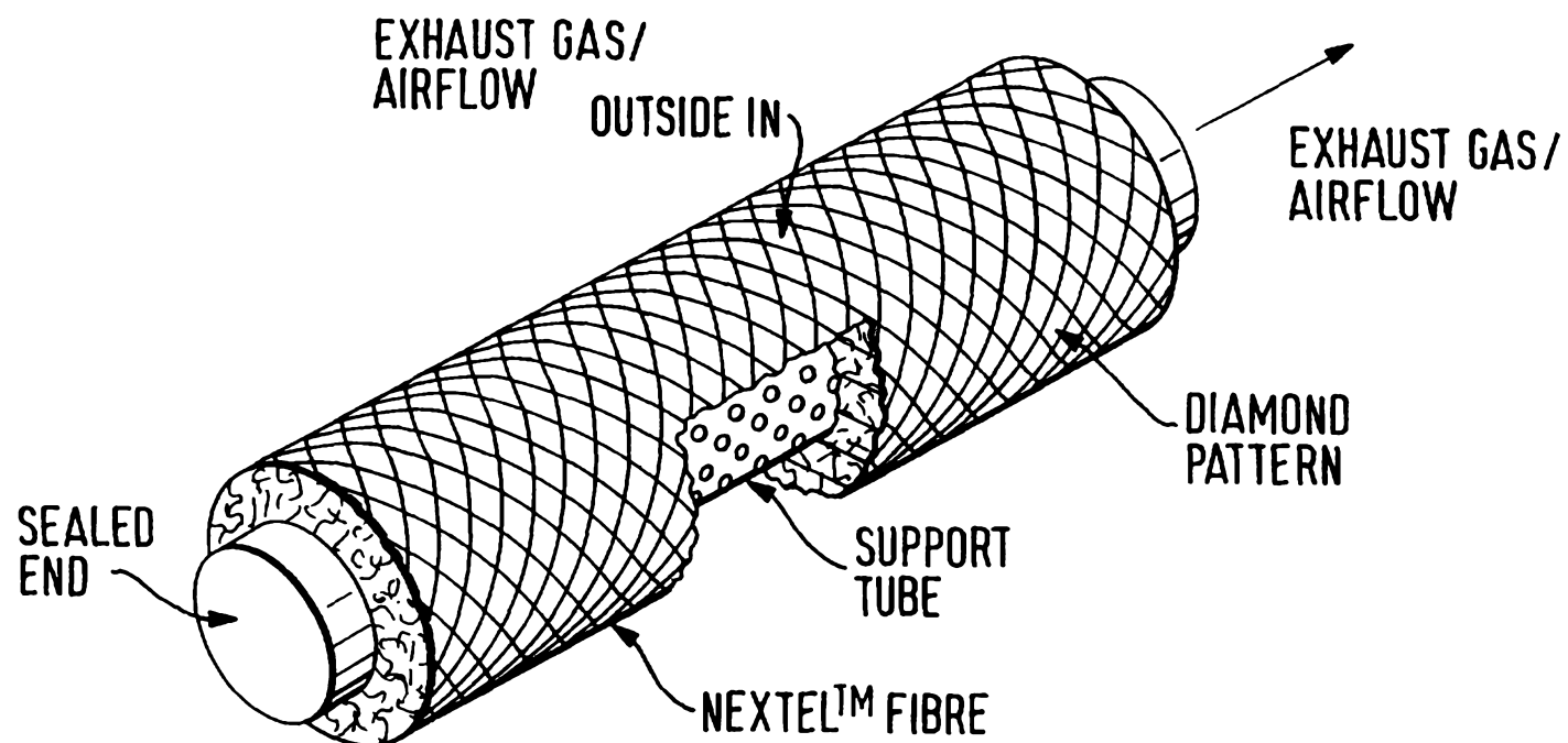
TYPICAL 3M DIESEL FILTER CARTRIDGE
