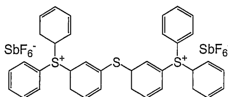
triarylsulfonium hexafluoroantimonate salts
