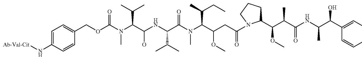
Ab-Val-Cit-PABC spacer-MMAE
