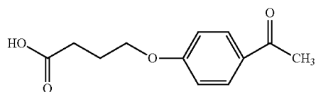
4-(4-acetylphenoxy)butanoic acid
