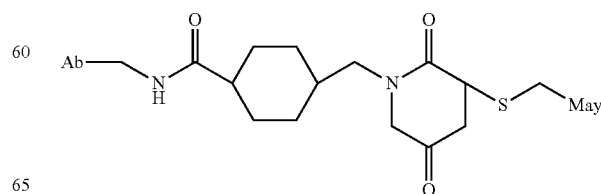
Formula XII
