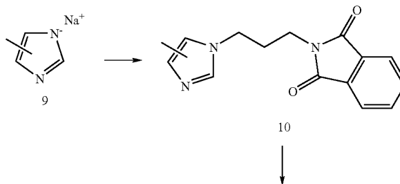
Scheme 2: Synthesis of 3-(4-methyl-1H-imidazol-1-yl)propan-1-amine (12)
