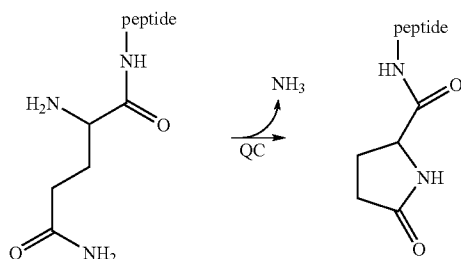
Scheme 1: Cyclization of glutamine by QC
