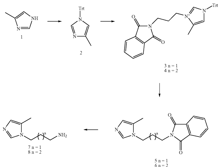
Scheme 1: Synthesis of 3-(5-methyl-1H-imidazol-1-yl)propan-1-amine (7)
