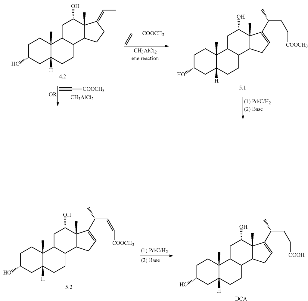
Scheme 5. Ene reaction and catalytic reduction for installation of DCA side chain
