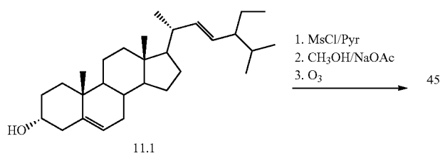
Scheme 11. Ozonolysis of i-steroid and side chain reduction
