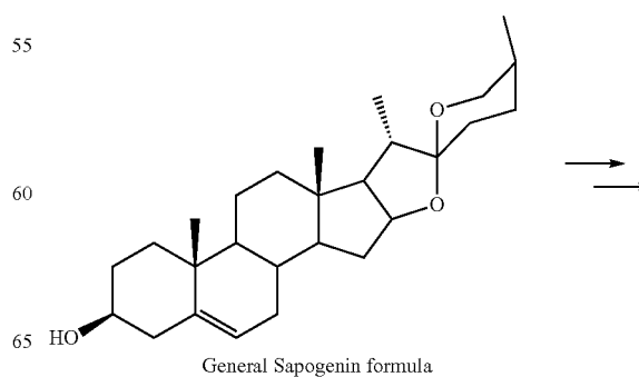
Scheme 10B. Synthetic route from saponin.
