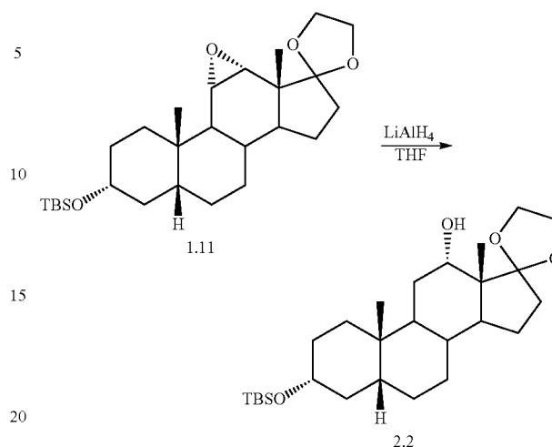
Scheme 3. Stereoselective Reduction of C 11 -C 12 epoxide.
