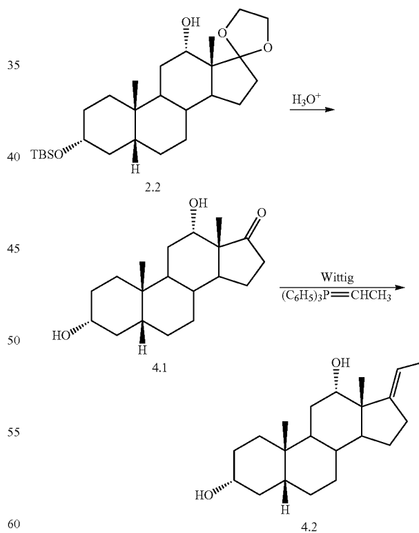
Scheme 4. Deprotection and Wittig Reaction
