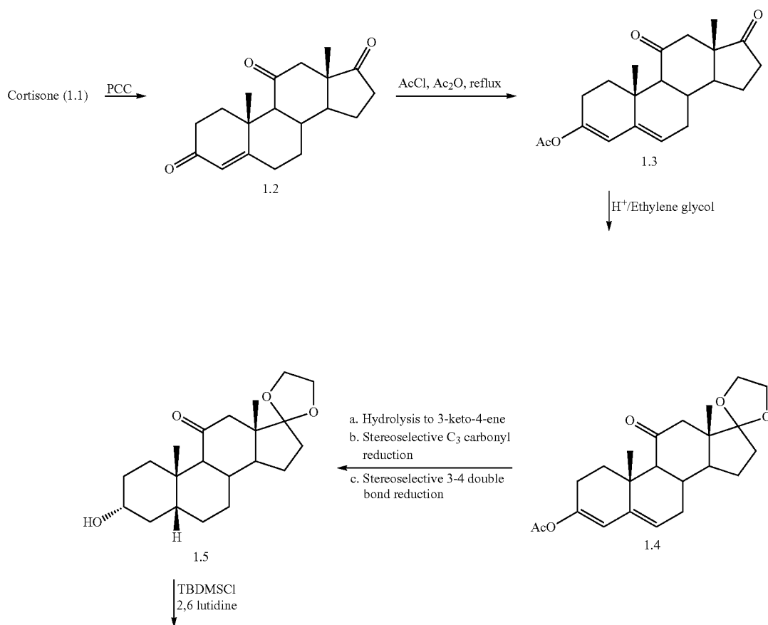
Scheme 1A. Synthesis of the two C-ring precursors of the C 12 hydroxyl group of DCA
