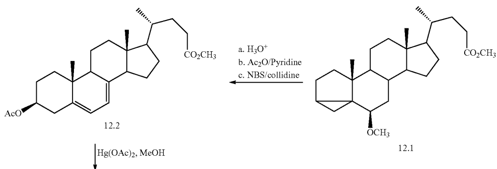
Scheme 12. Triene formation and allylic oxidation
