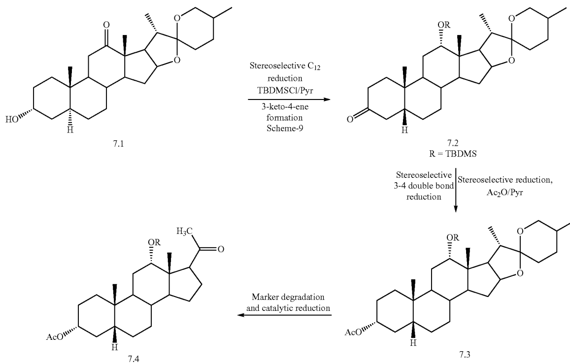
Scheme 7. C_{12} -hydroxyl group introduction, AB ring modification and side chain cleavage
