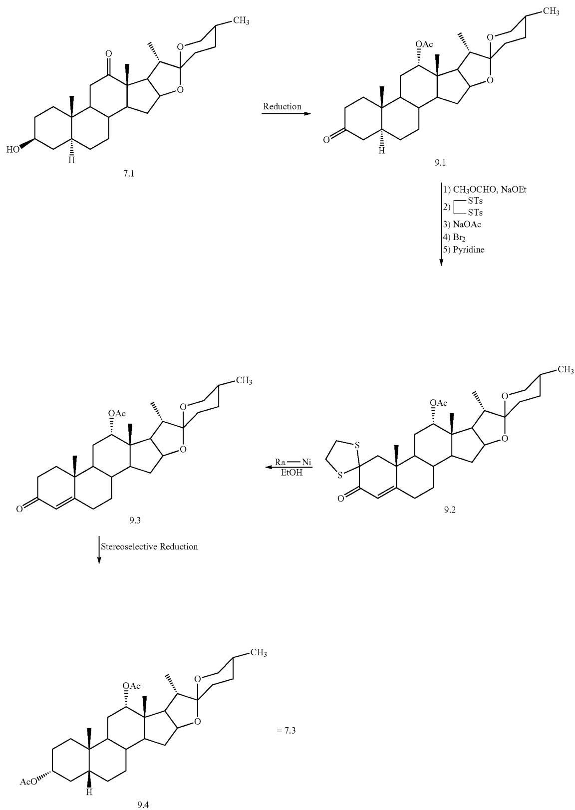
Scheme 9. Dithioethane route to 3-keto-4-ene
