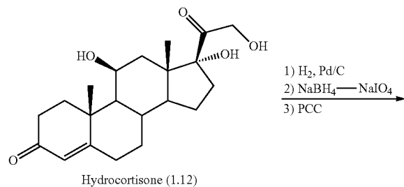
Scheme 1B. Synthesis of DCA from Hydrocortisone
