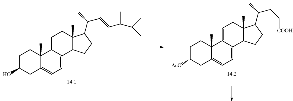
Scheme 14. Triene formation from Ergosterol
