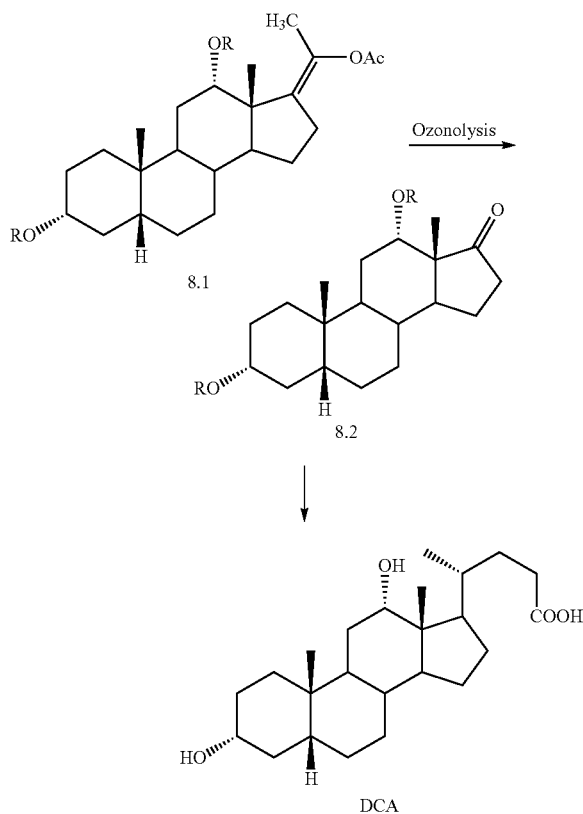
Scheme 8. Side-chain introduction
