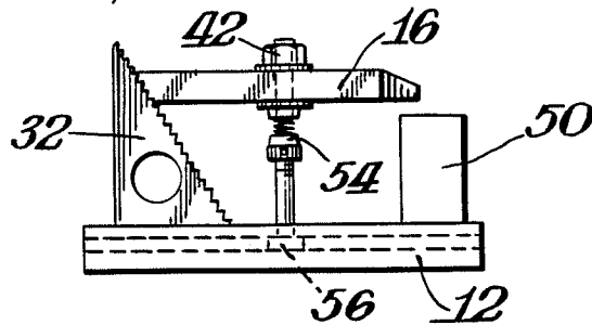
Fig. 6. (Prior Art)
