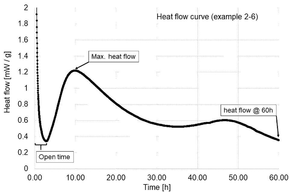
Figure 1: heat flow curve (example 2-6)
