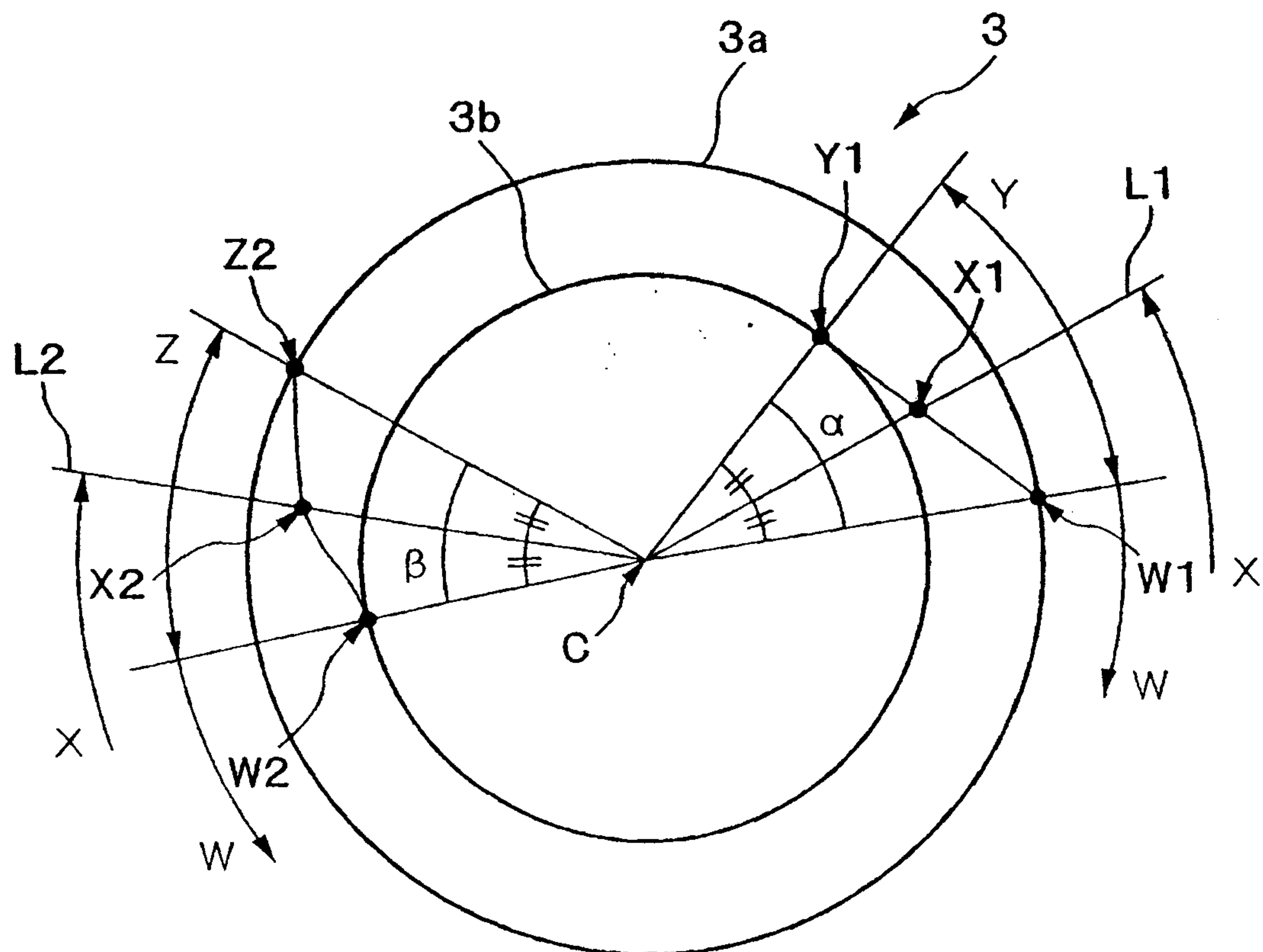
FIG. 8 PRIOR ART
