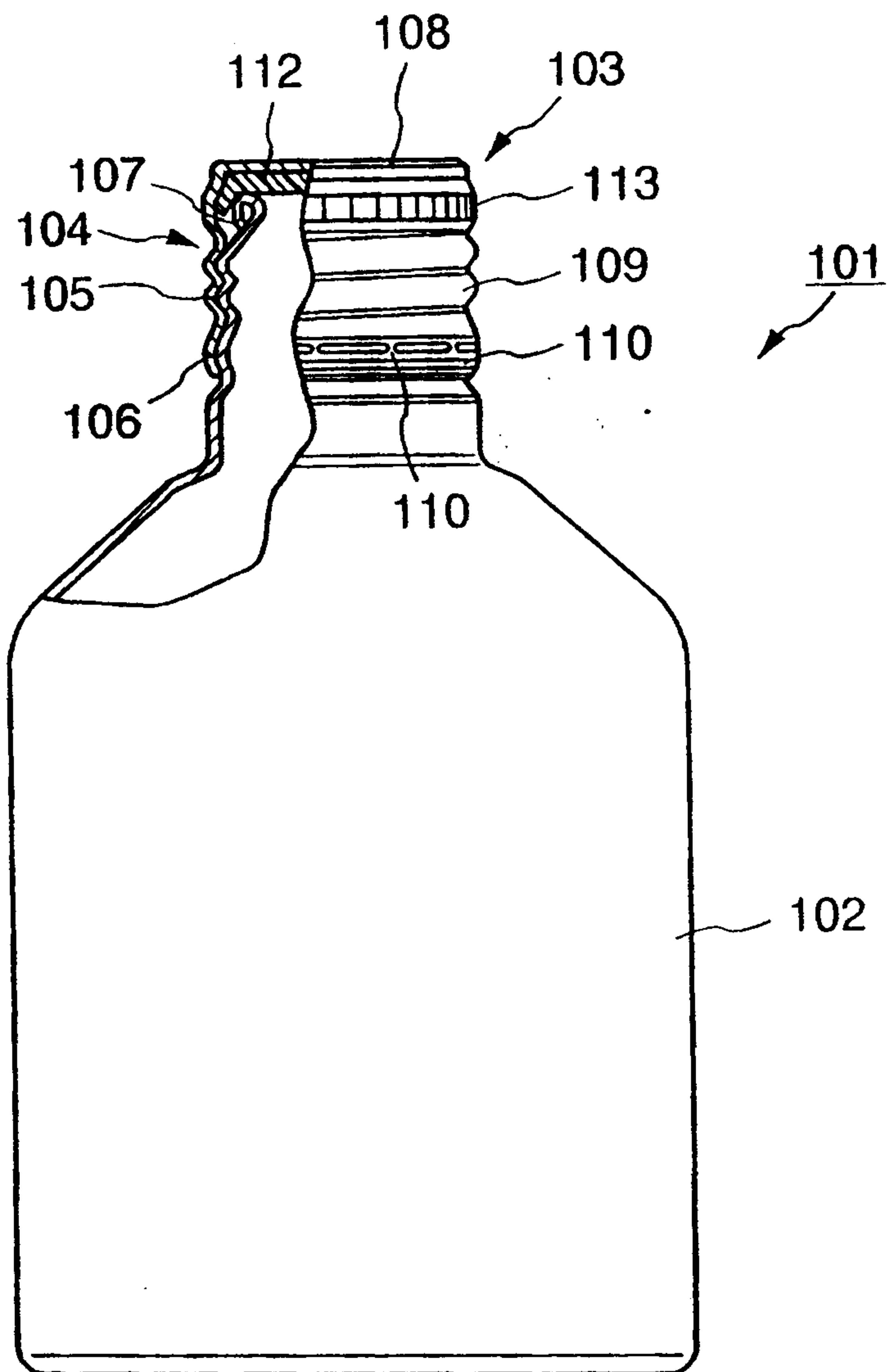
FIG. 11 PRIOR ART
