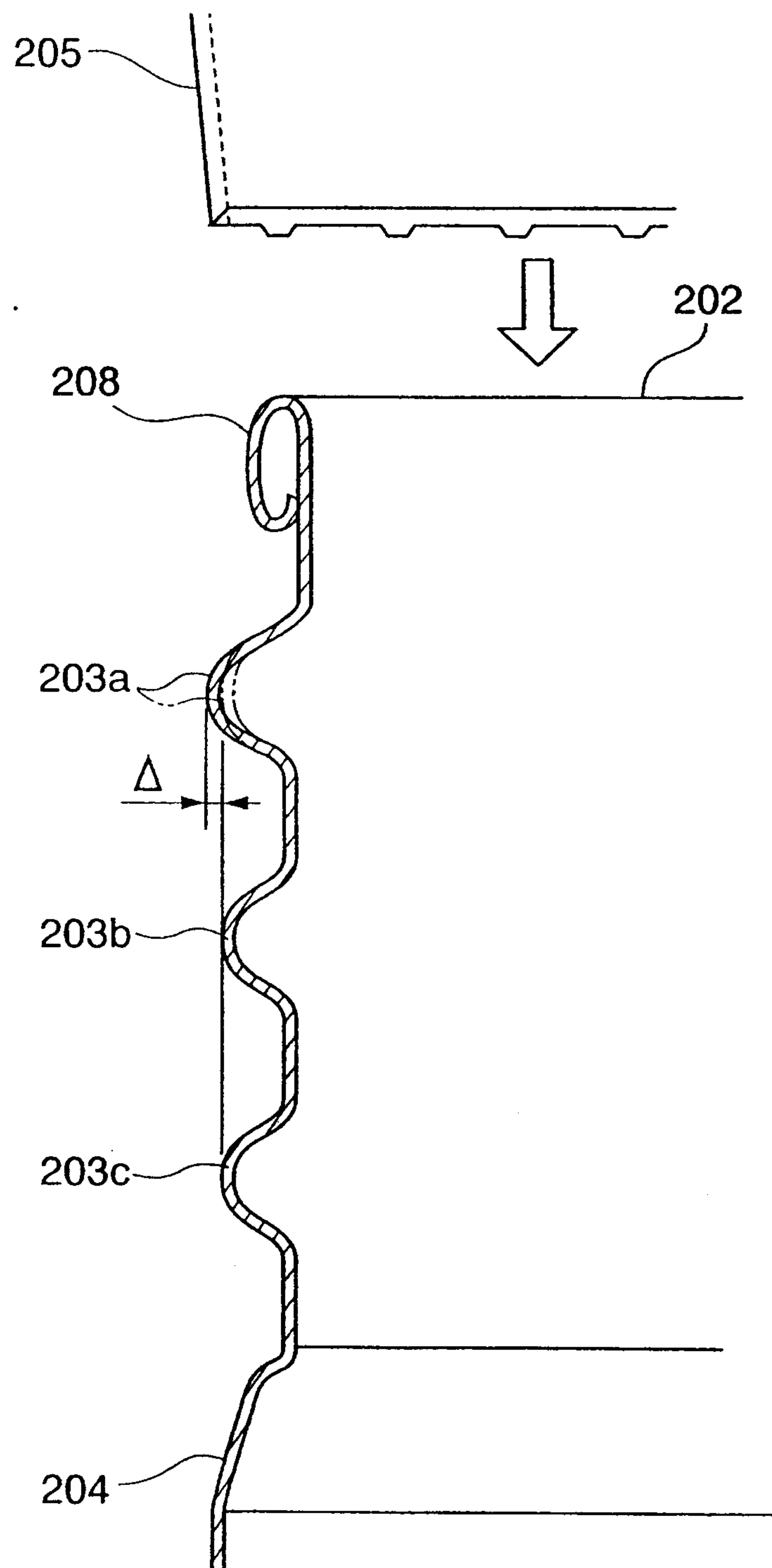
FIG. 22 PRIOR ART
