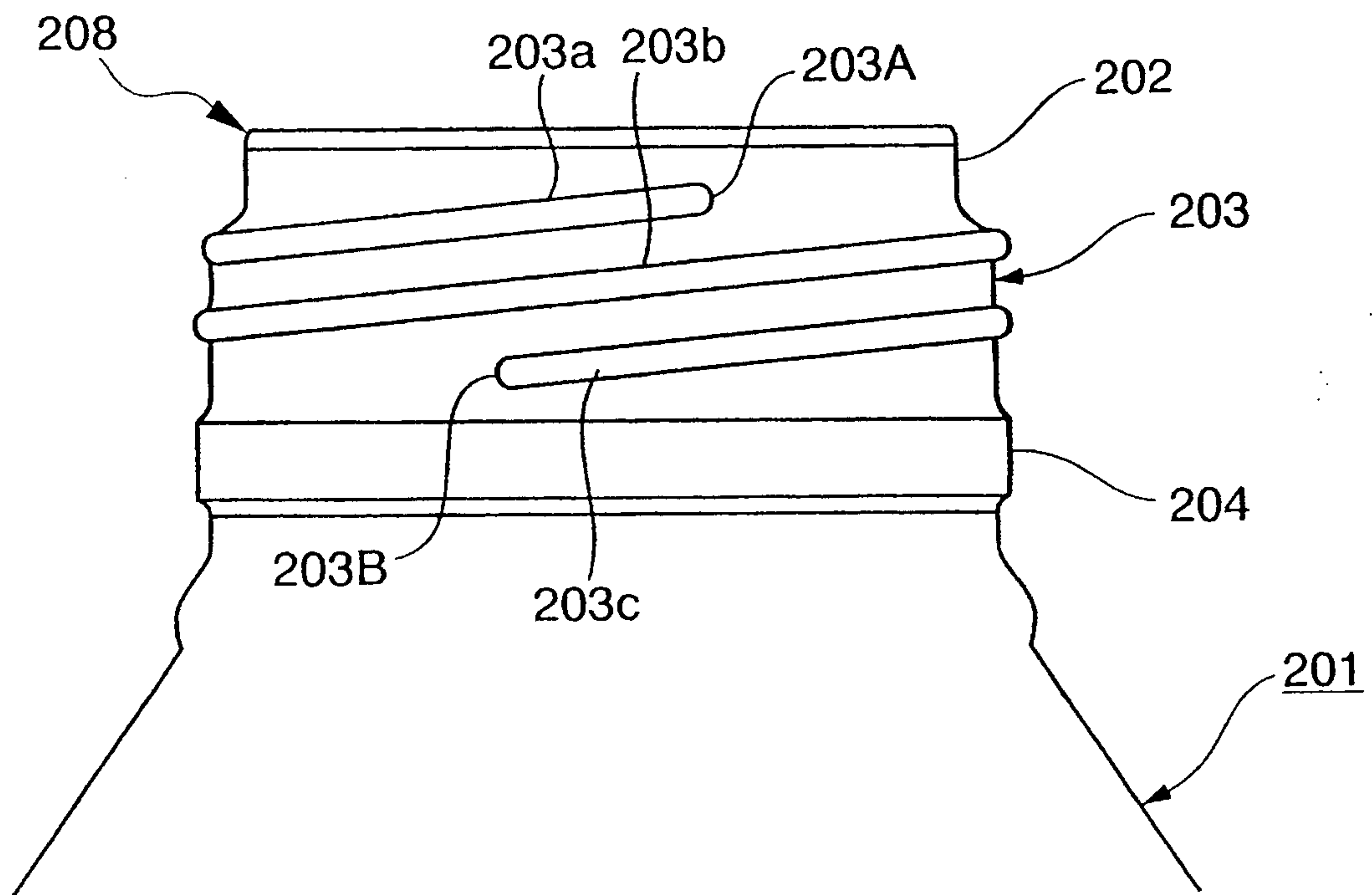
FIG. 21 PRIOR ART
