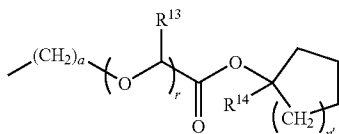
[Chemical Formula 13]
