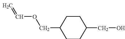
[Chemical Formula 42]
