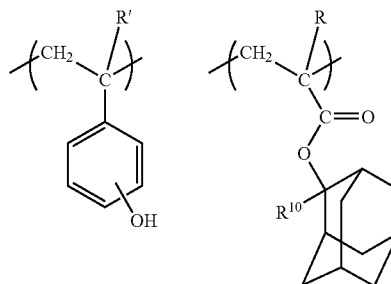
[Chemical Formula 17]
