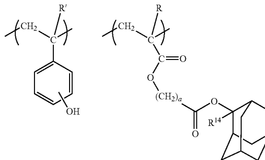
[Chemical Formula 18]
