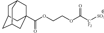
[Chemical Formula 63]
