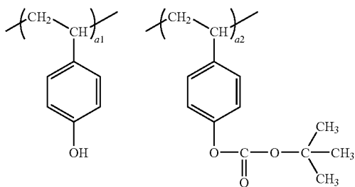
[Chemical Formula 61]
