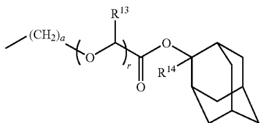
[Chemical Formula 12]
