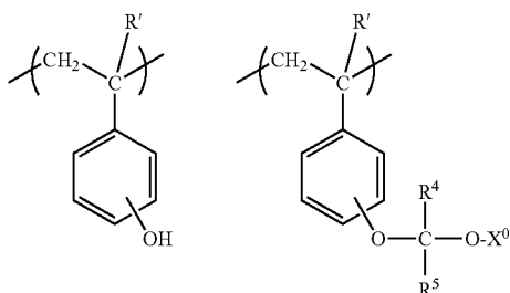
[Chemical Formula 15]
