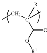
[Chemical Formula 3]
