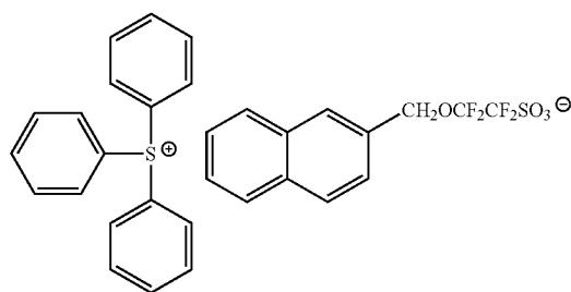
[Chemical Formula 63]
