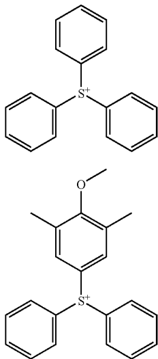
[Chemical Formula 23]
