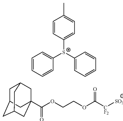
[Chemical Formula 62]
