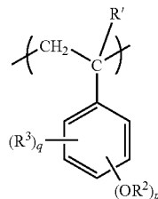
[Chemical Formula 4]
