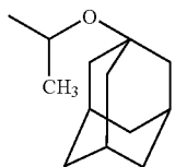
[Chemical Formula 6]
