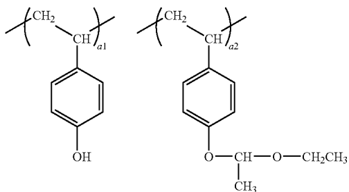
[Chemical Formula 60]
