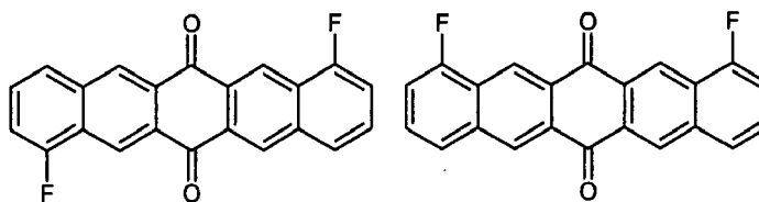
Compound 17
