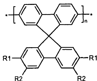
Formula 16
