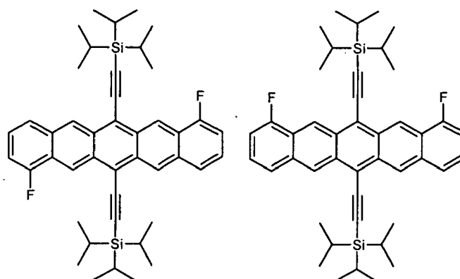
Compound 19
