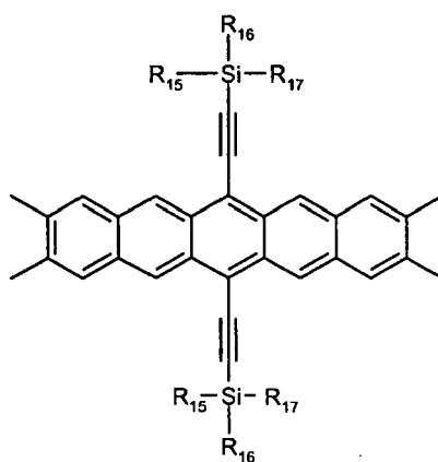
Formula 8A'
