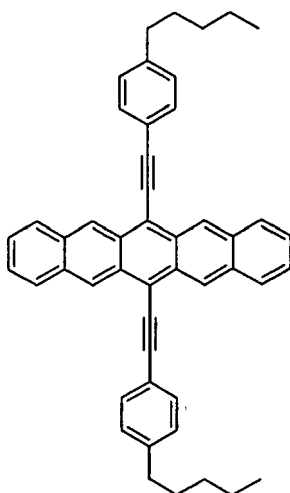
Compound 11
