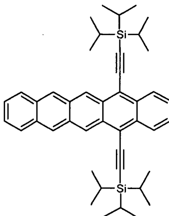
Compound 14
