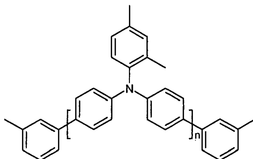
Formula (18)
