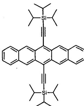
Compound 1
