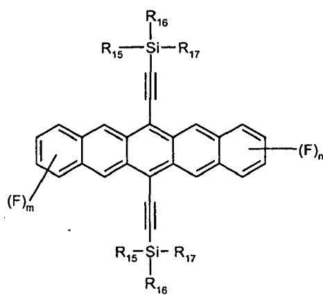
Formula 8B'
