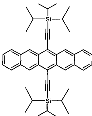
Group 1, example 1
