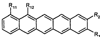
Formula 5
