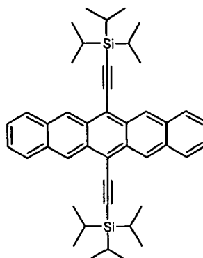
Compound 1
