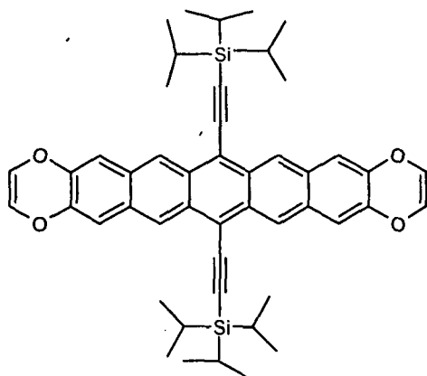
Group 8, example 5
