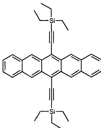
Compound 10
