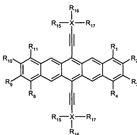
Formula 8
