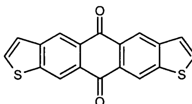
Compound 6
