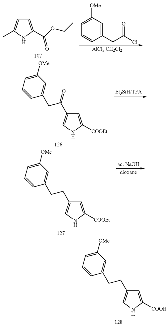
Synthesis of 4-[2-(3-Methoxy-phenyl)-acetyl]-5-methyl-1H-pyrrole-2-carboxylic Acid Ethyl Ester (126)
