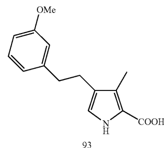
Synthesis of 4-[2-(3-Methoxy-phenyl)-acetyl]-3-methyl-1H-pyrrole-2-carboxylic Acid Ethyl Ester (91)
