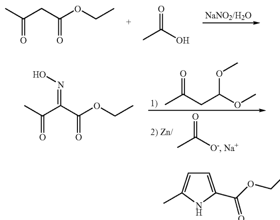
SCHEME 2- Method for the synthesis of 5-substituted-1H-pyrrole-2-carboxylic acid ester starting materials
