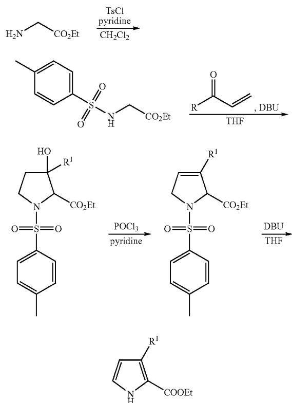
SCHEME 1- Method for the synthesis of 3-substituted-1H-pyrrole-2-carboxylic acid ester starting materials
