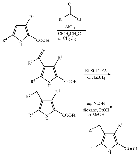
SCHEME 3- Method for the synthesis of 4-substituted-, 3,4-disubstituted-, 4,5-disubstituted-, or 3,4,5-trisubstituted 1H-pyrrole-2-carboxylic acids
