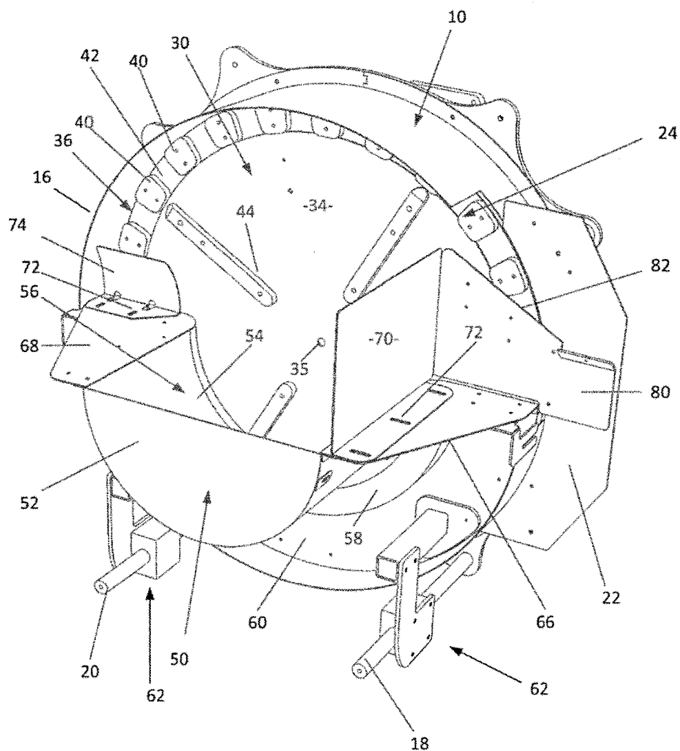
Fig. 1 (PRIOR ART)
